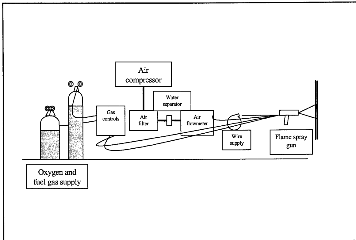
Figure 2-2. Typical flame spray system
