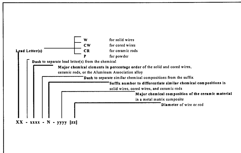
Figure 3-1. Thermal spray feedstock designation nomenclature
