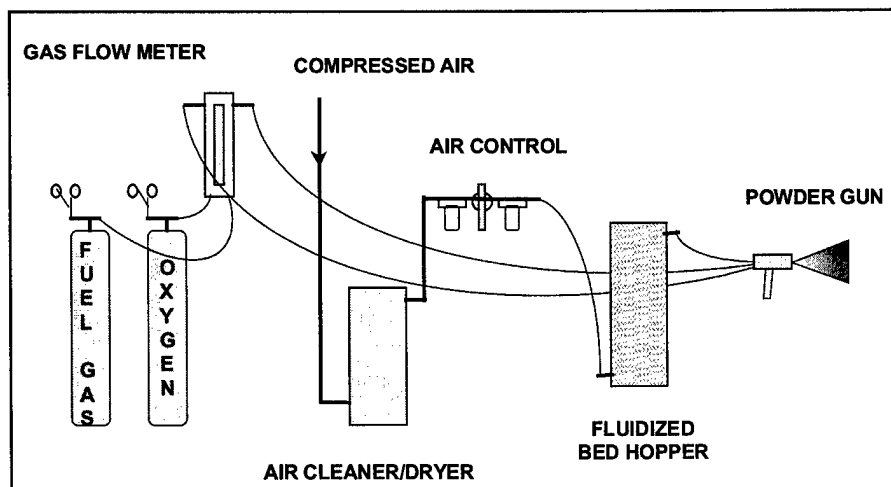
Figure 2-4. Typical combustion powder gun installation
