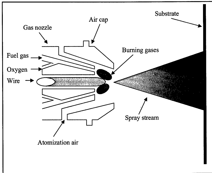
Figure 2-3. Typical flame spray gun
