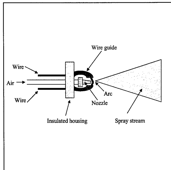
Figure 2-7. Typical two-wire arc spray gun
