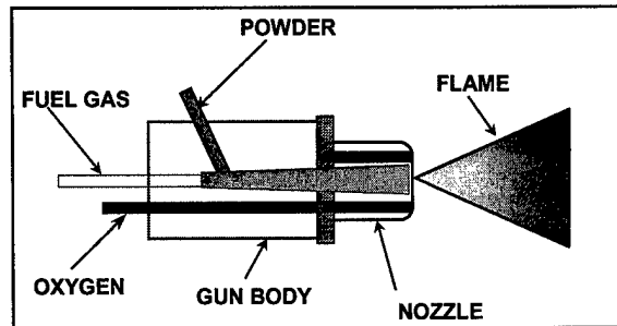
Figure 2-5. Powder gun cross section
