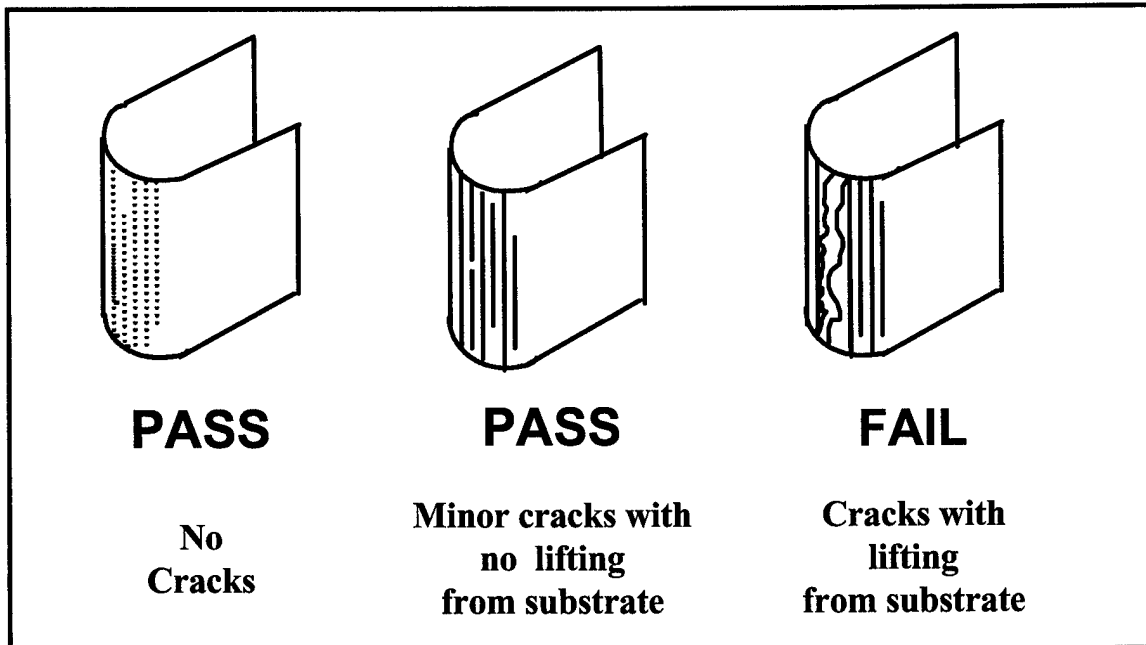
Figure 9-2. Representative pass and fail conditions for qualitative bend test
