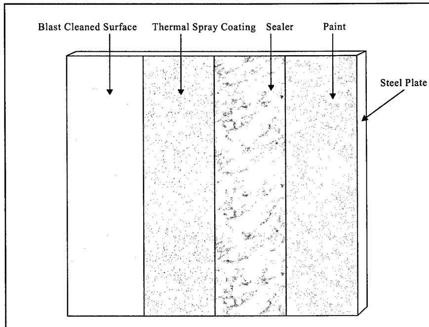
Figure 9-1. Representative job reference standard
