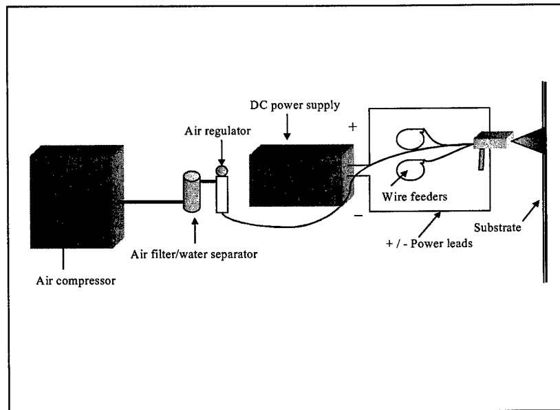
Figure 2-6. Typical two-wire arc spray system
