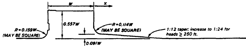
a. PRESSURE DETAILS
