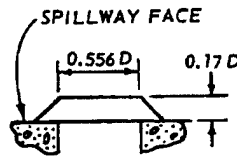
VIEW B - B
