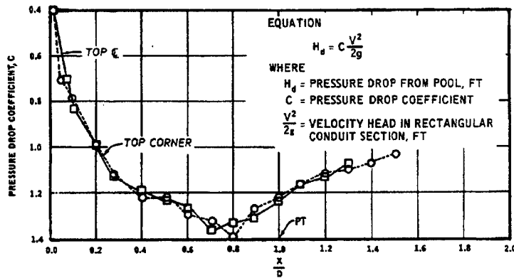
a. "SHORT" CURVE
