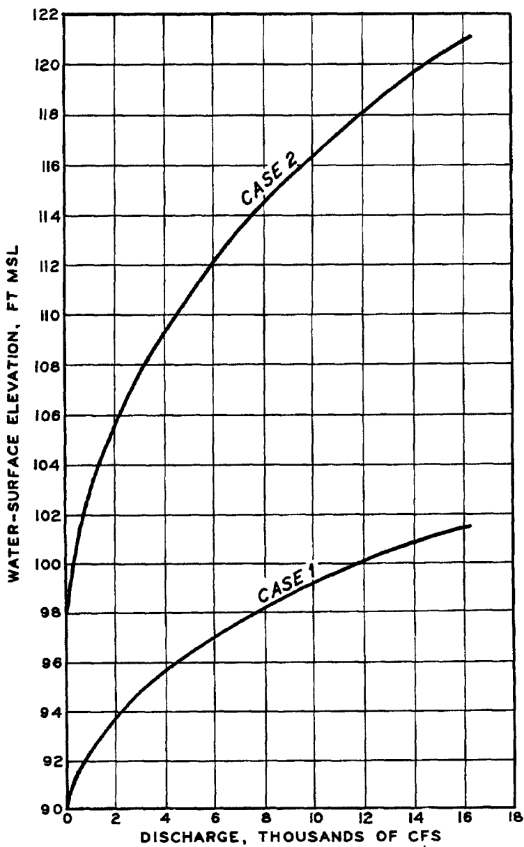
TAILWATER RATING CURVE
