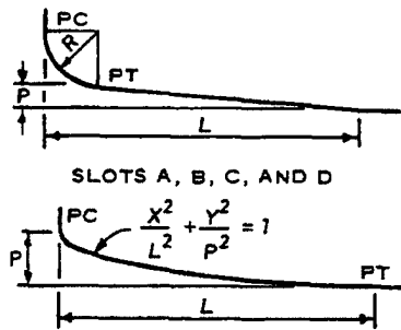
SLOTS A, B, C, AND D SLOTS E, F, G, AND H DOWNSTREAM PLAN OF GATE SLOTS
