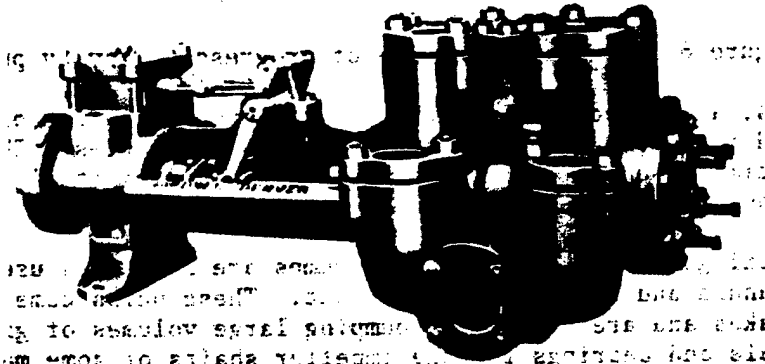
b. DIVIDED FLUID-CYLINDER VALVE-POT-TYPE PUMP
