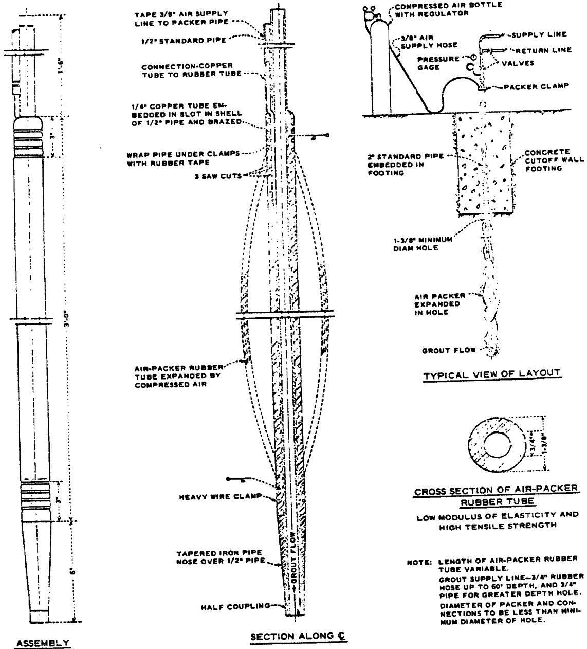
Figure 6-17. Air packer
