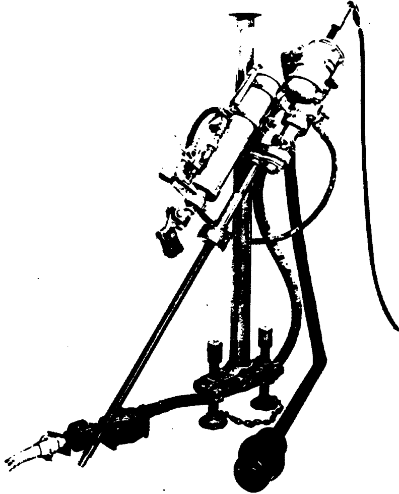
Figure 6-3. Post drill
