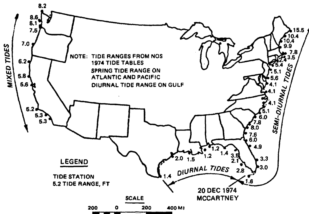
Figure 2-1. Ocean tide ranges for the continental United States
