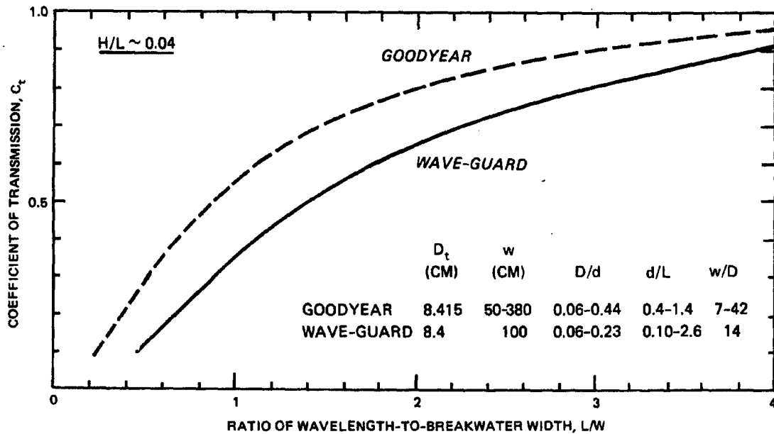
Figure 6-18. Comparison of wave transmission coefficient C_t for wave-guard and Goodyear floating breakwater concepts
