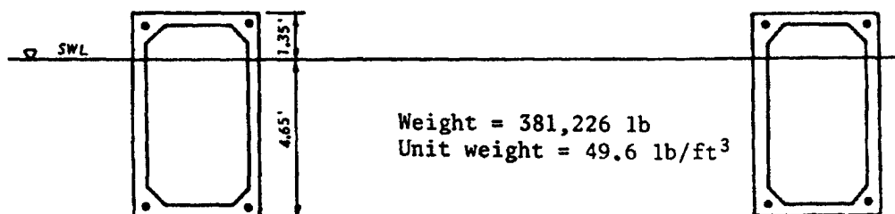
SECTION B-B'
