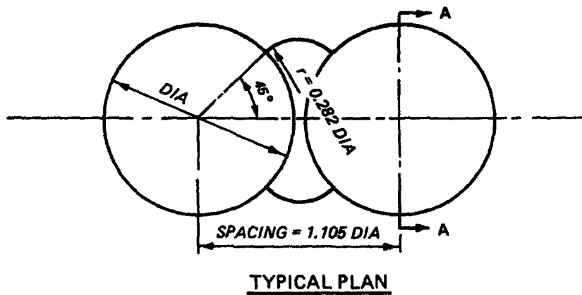
Figure 5-3. Circular type of cellular breakwater
