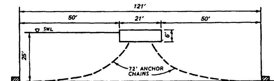
END VIEW
