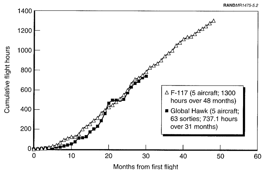
Figure 5.2—Comparison of Global Hawk and F-117 Flight Test Programs
