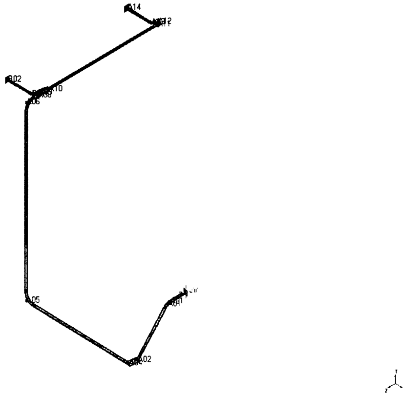
Figure 3. Upper Piping Flexibility Analysis Model
