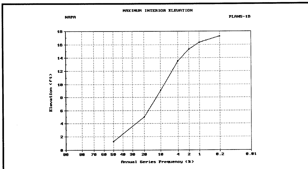
Figure D-17. Stage-frequency for minimum facility - Interior Area 5 - HEA, unblocked
