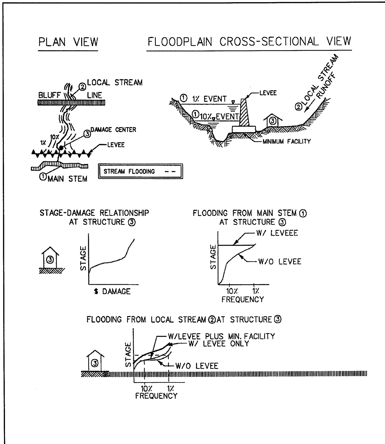
Figure 4-3. Line-of-protection with minimum facility
