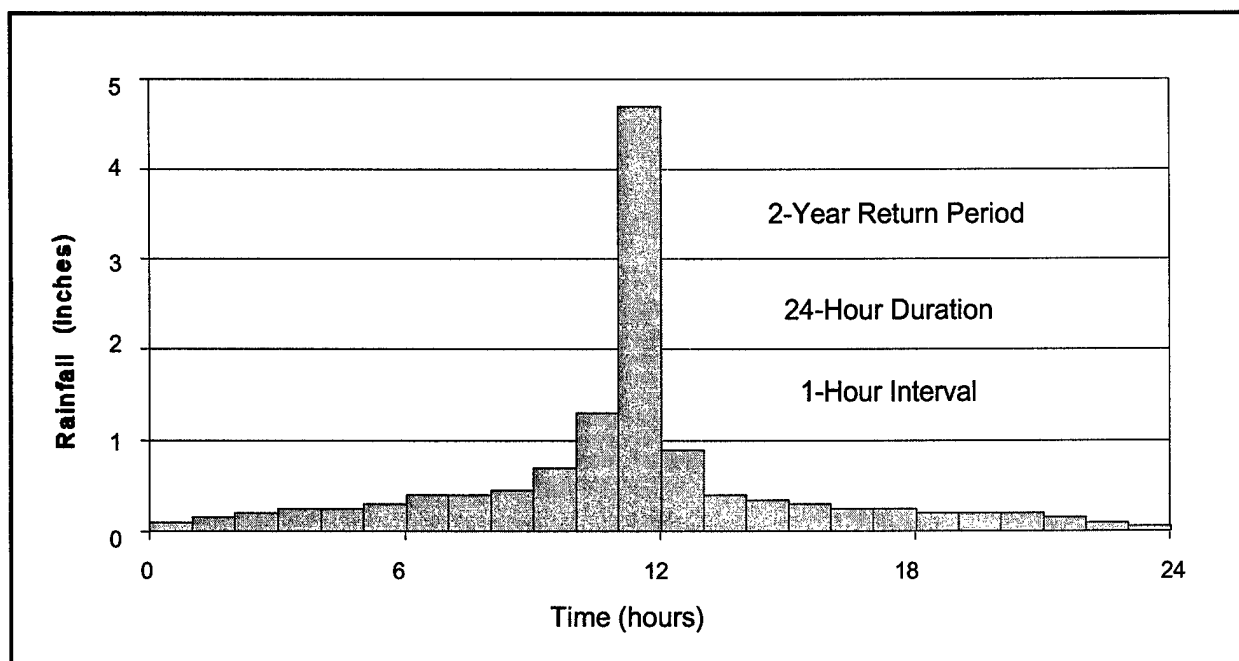
Figure 3-9. Hypothetical frequency storm hyetograph
