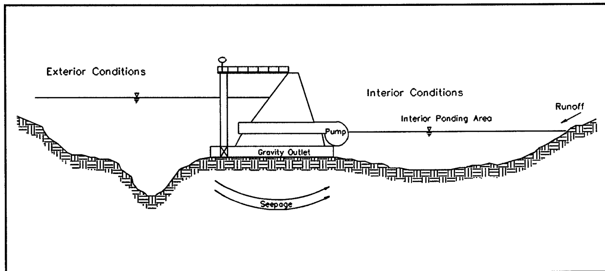
Figure 1-2. Cross section of typical interior system
