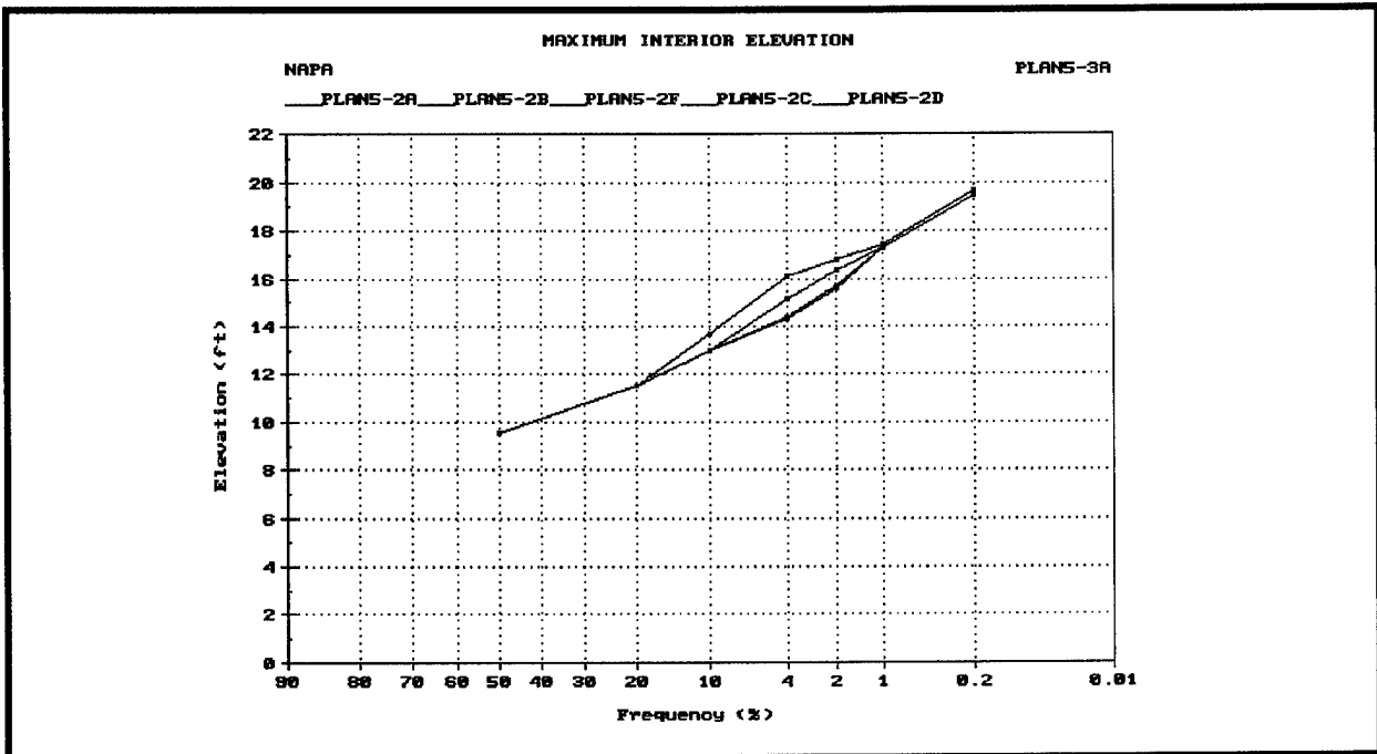
Figure D-23. Stage-frequency relationships for a range of gravity outlet sizes
