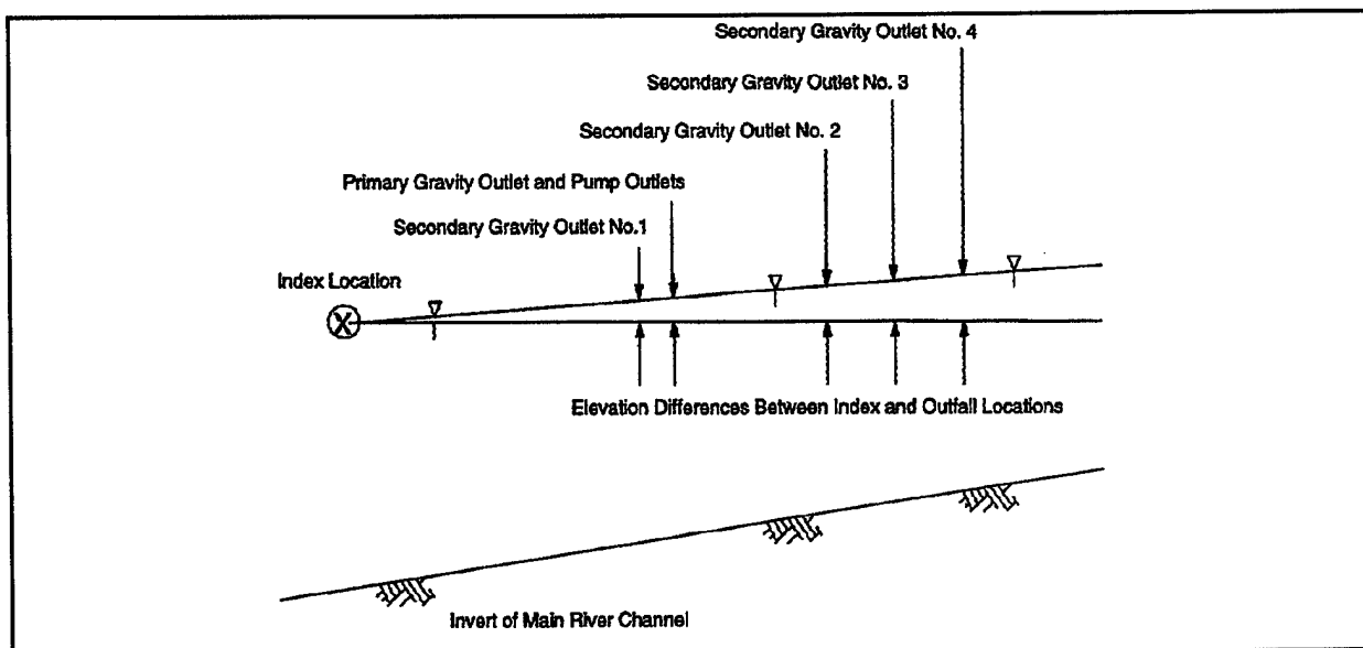
Figure 3-20. Main river transfer concept: slope-profile
