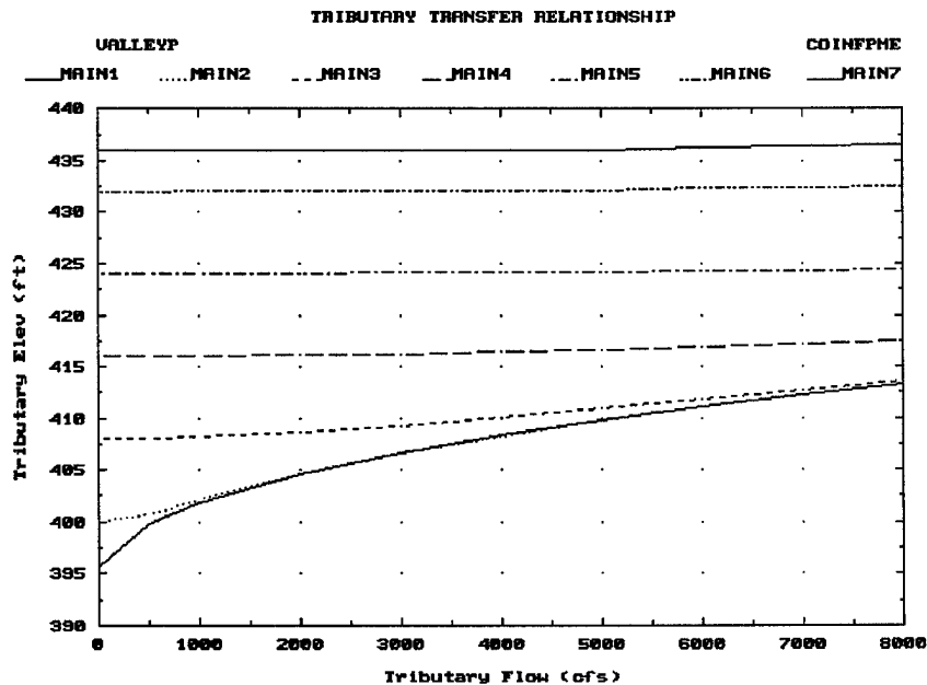
Figure E-4. Plot of tributary rating table
