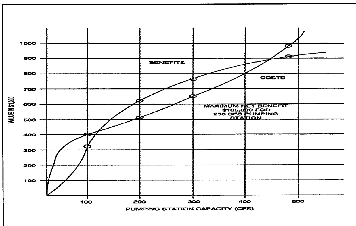
Figure 5-5. Pump station benefit-cost curve
