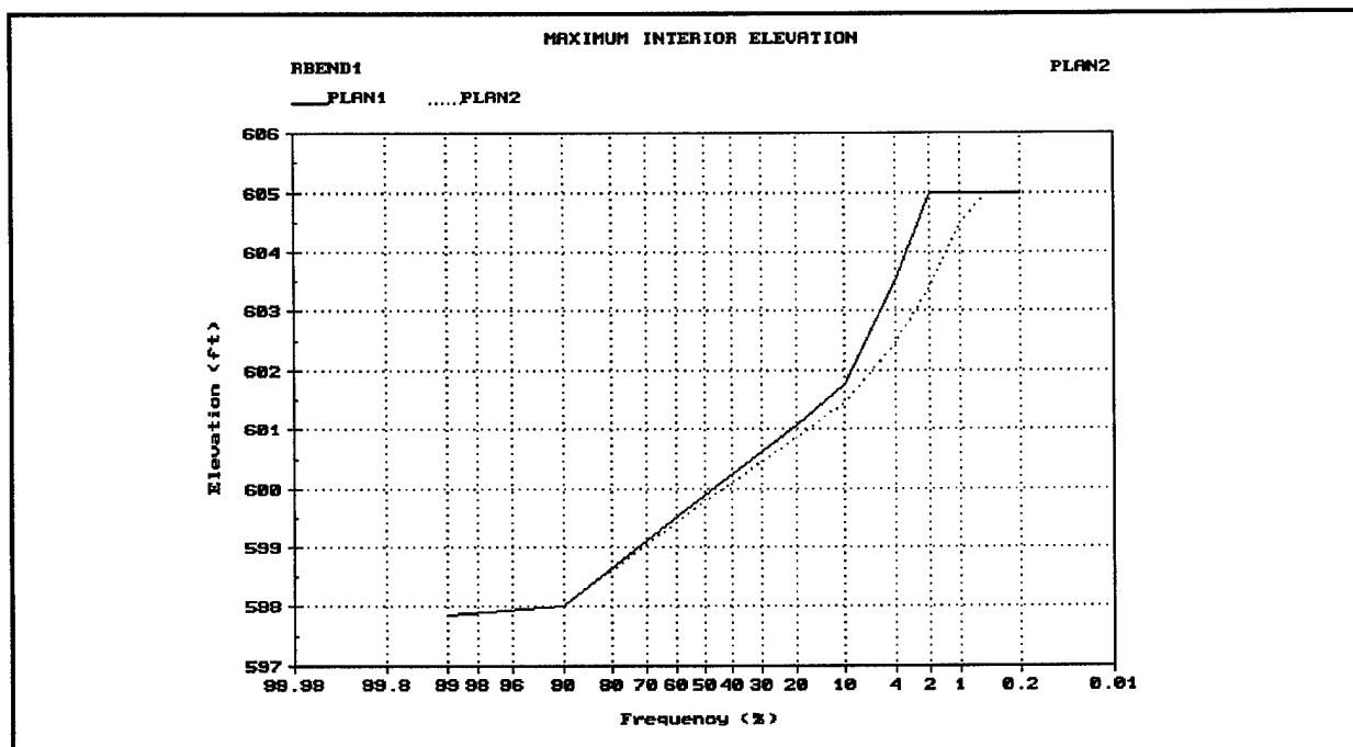
Figure 5-9. Maximum interior elevation-frequency plot
