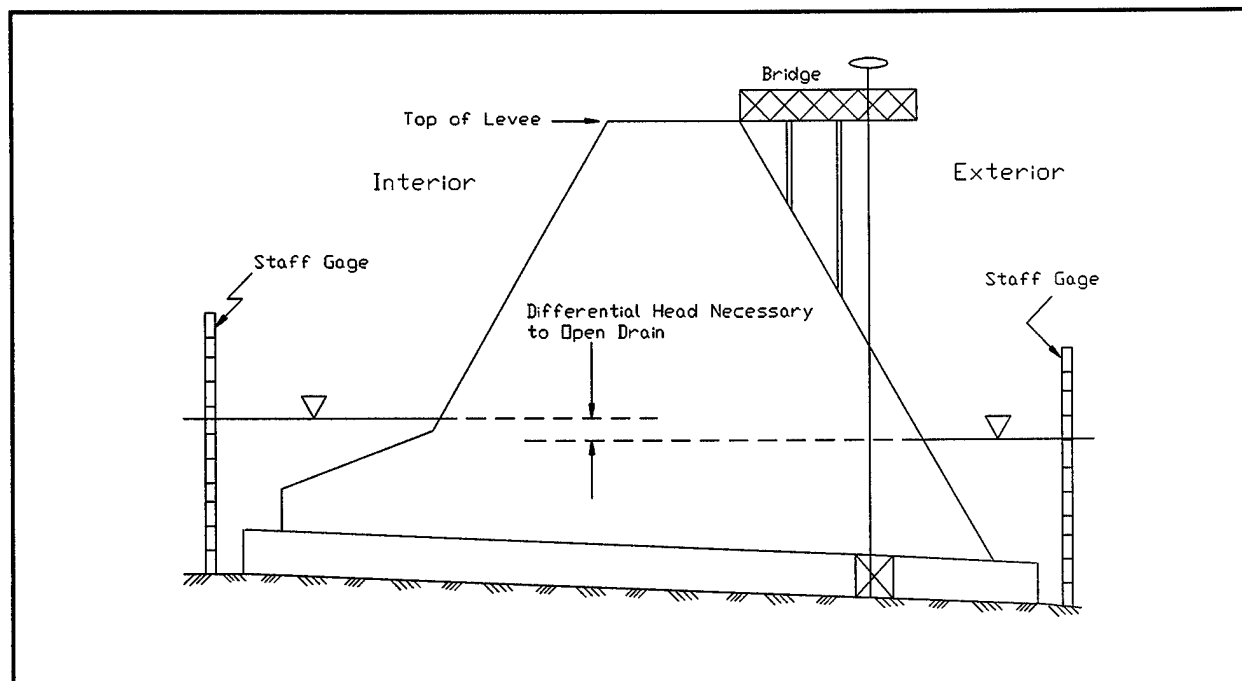
Figure 5-2. Gravity outlet concepts
