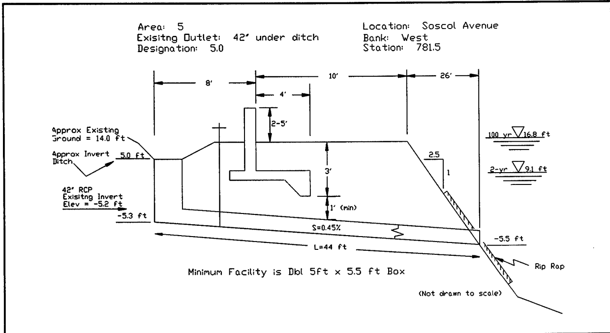
Figure D-11. Typical layout - new box culvert with drop inlet Area 5
