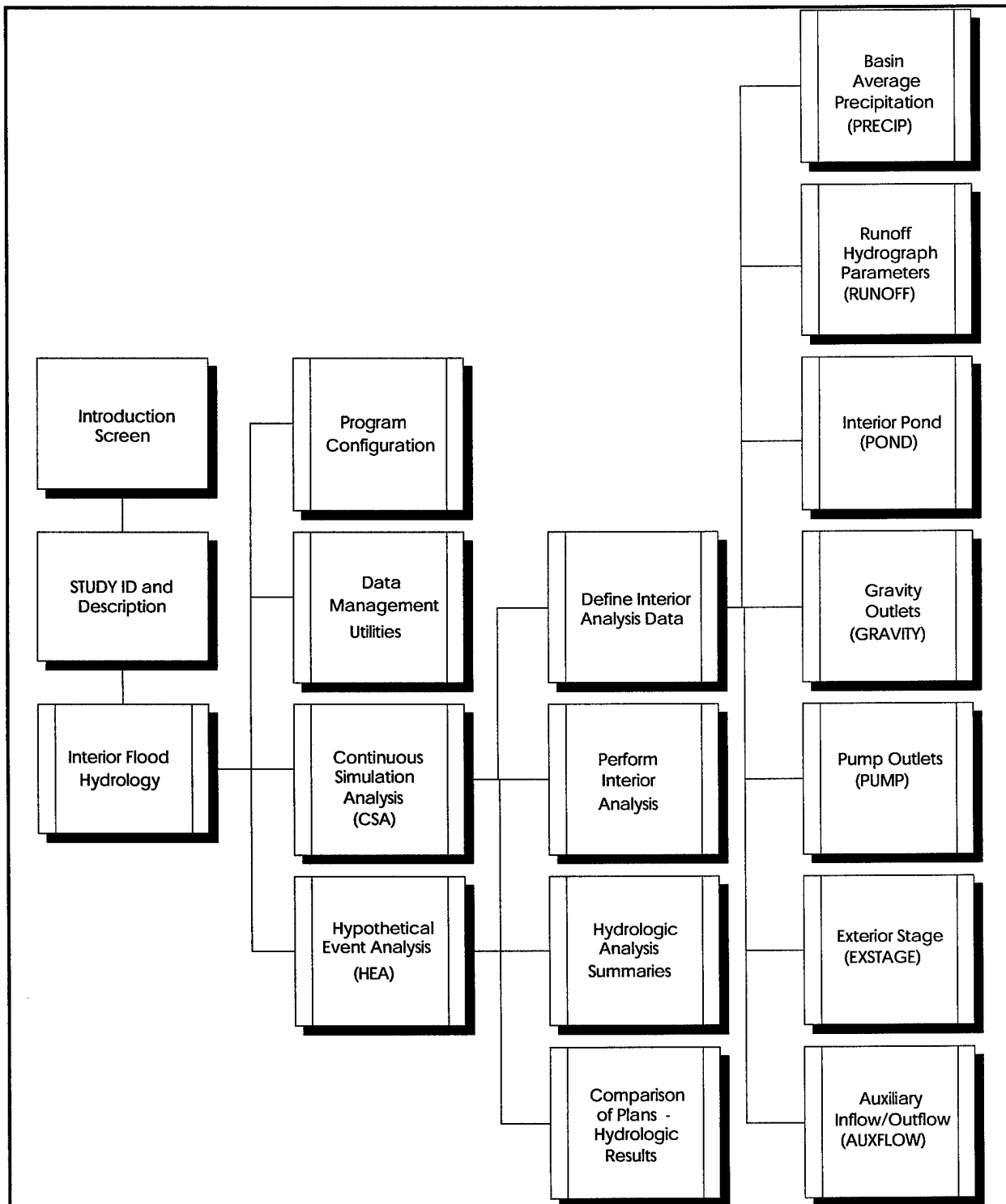
Figure 3-1. HEC-IFH program menu hierarchy
