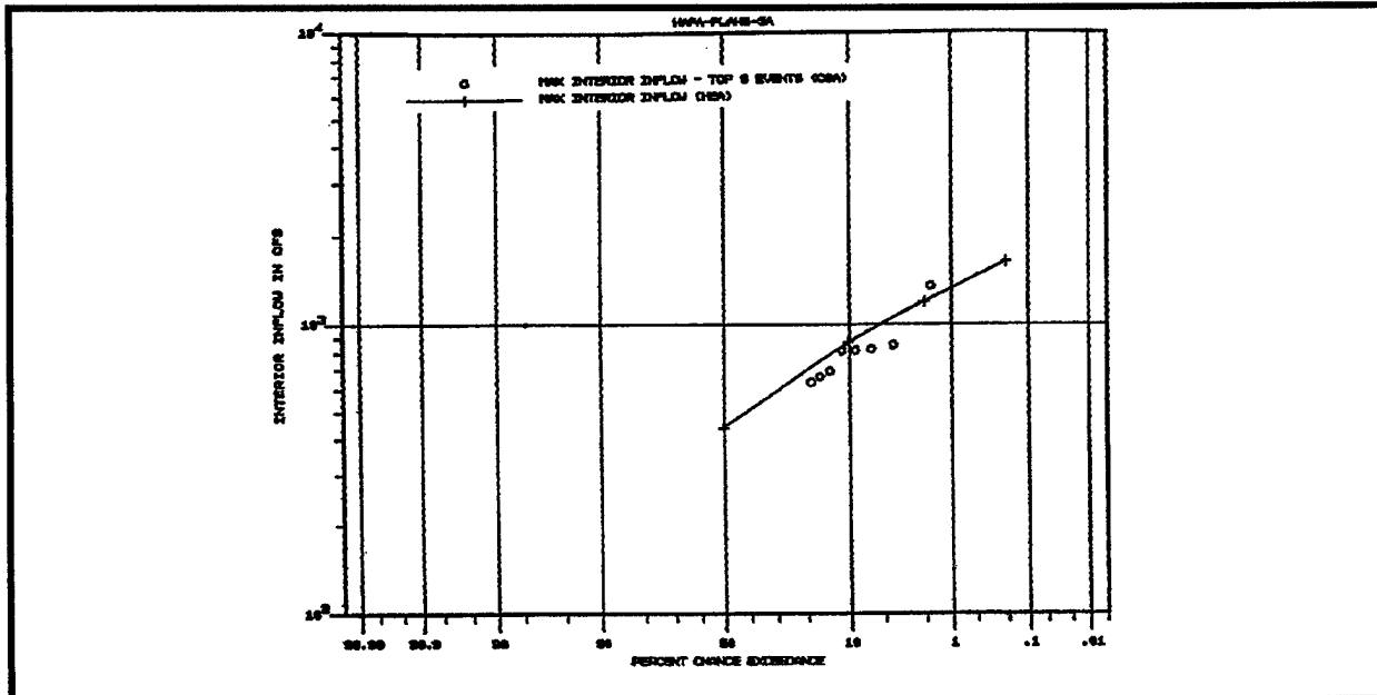
Figure D-6. Interior runoff discharge-frequency relationships - CSA and HEA
