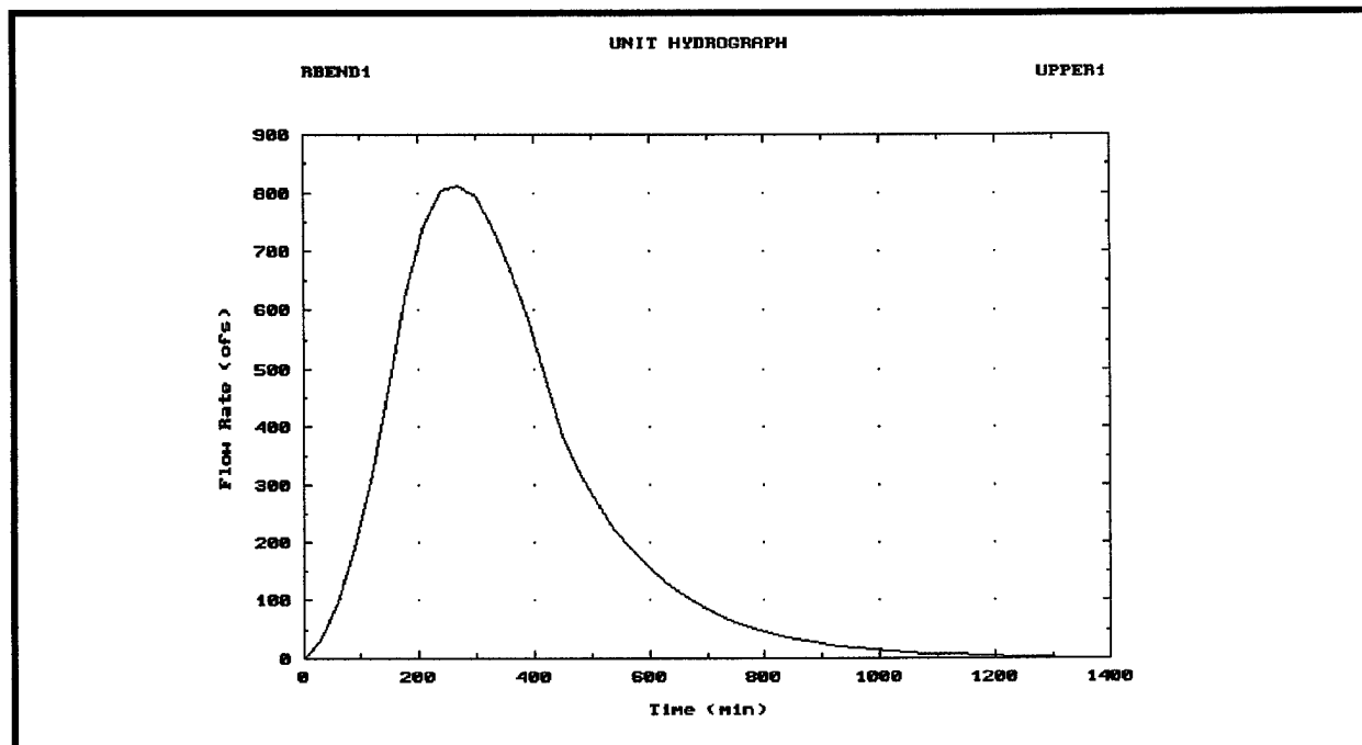
Figure 3-12. Unit hydrograph plot
