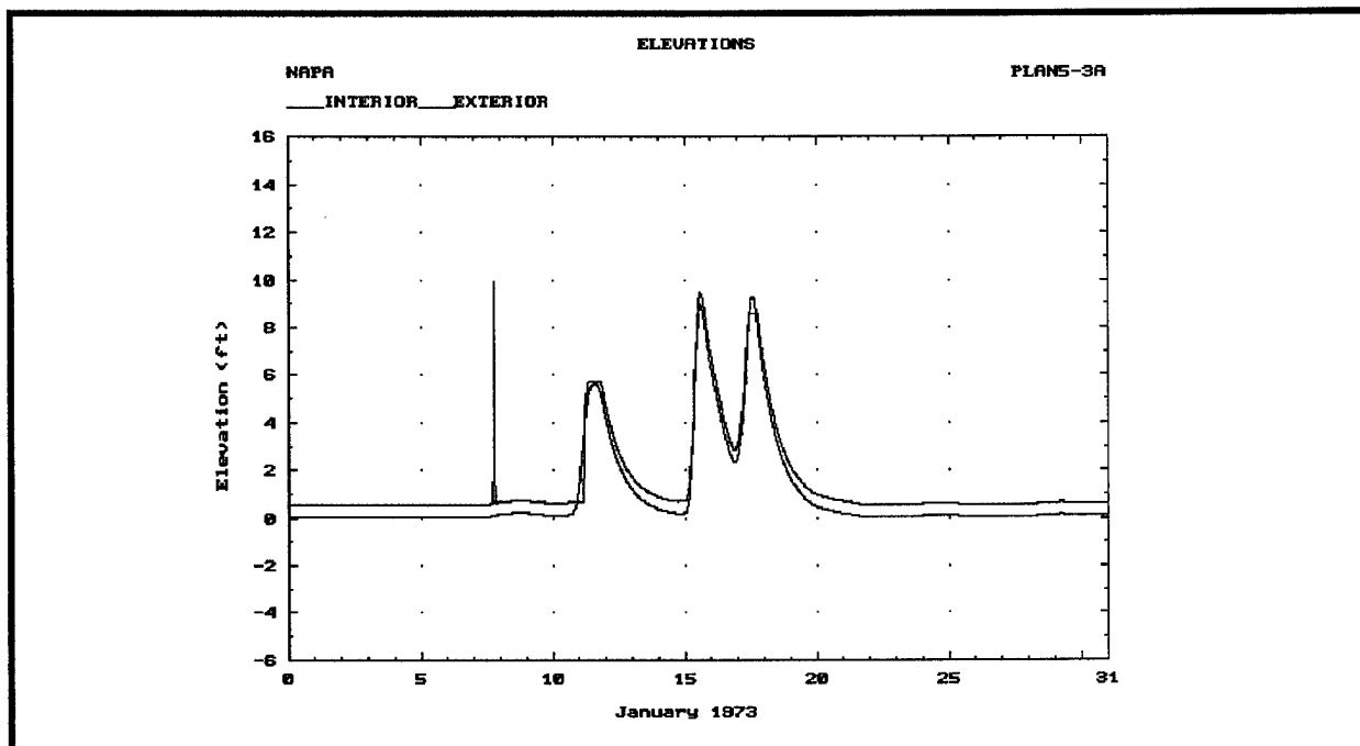
Figure D-20. Interior and exterior stages - January 1973 event, CSA
