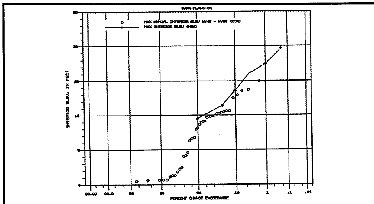
Figure D-21. Interior stage-frequency relationships for CSA and HEA - Area 5
