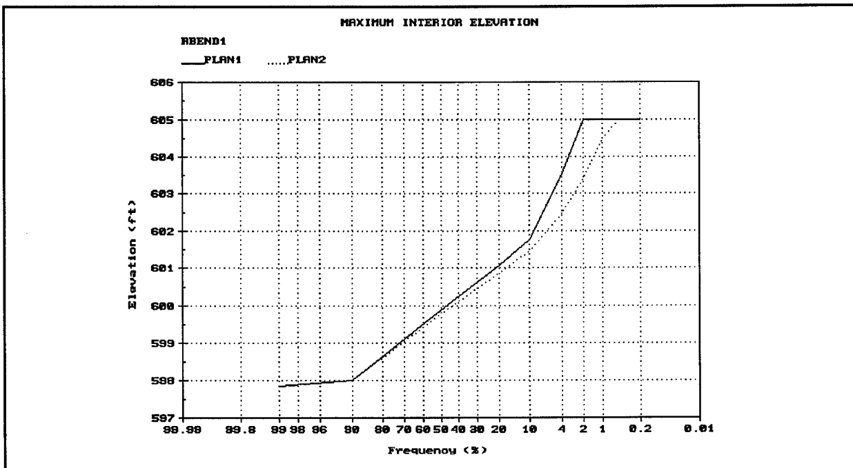
Figure 5-4. Plan comparison of stage-frequency relationships
