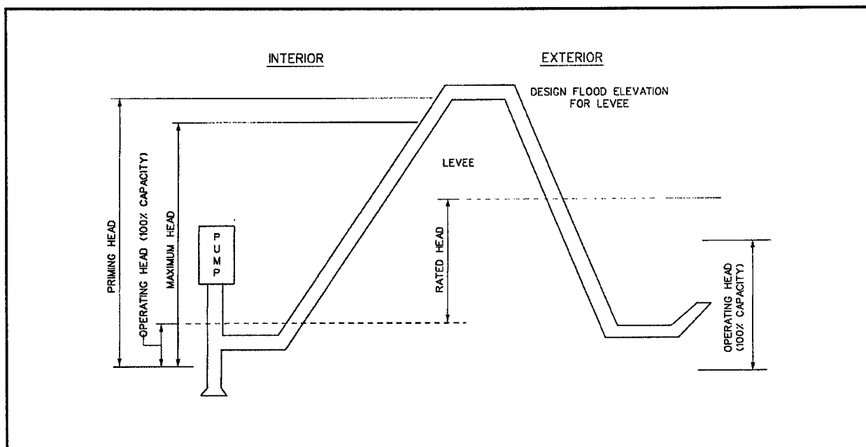
Figure 5-3. Pump station concepts
