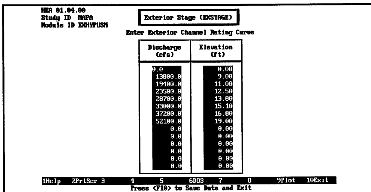
Figure D-15. Exterior rating curve for Interior Area 5
