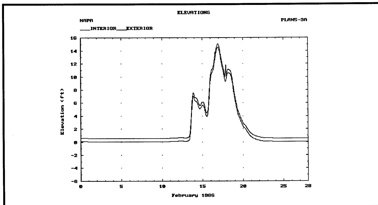
Figure D-19. Interior and exterior elevation - February 1986, CSA
