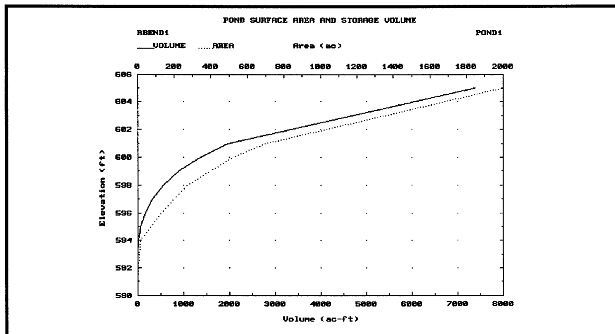
Figure 3-16. Pond surface area and storage volume plot
