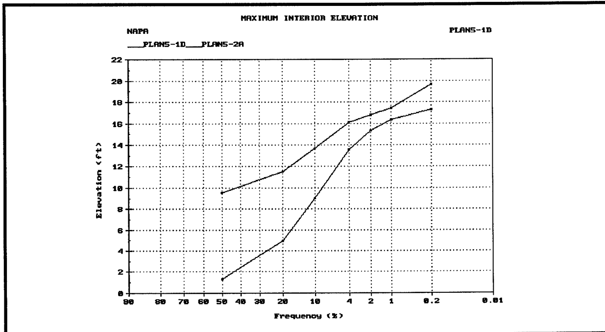
Figure D-18. Stage-frequency relationships - HEA unblocked and interior/exterior
