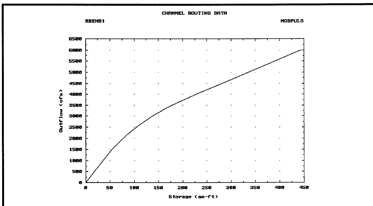
Figure 3-14. Modified Puls storage-outflow plot
