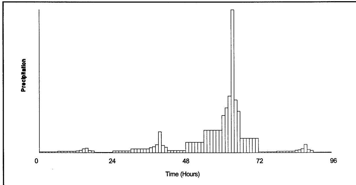
Figure 3-10. Typical SPS precipitation distribution
