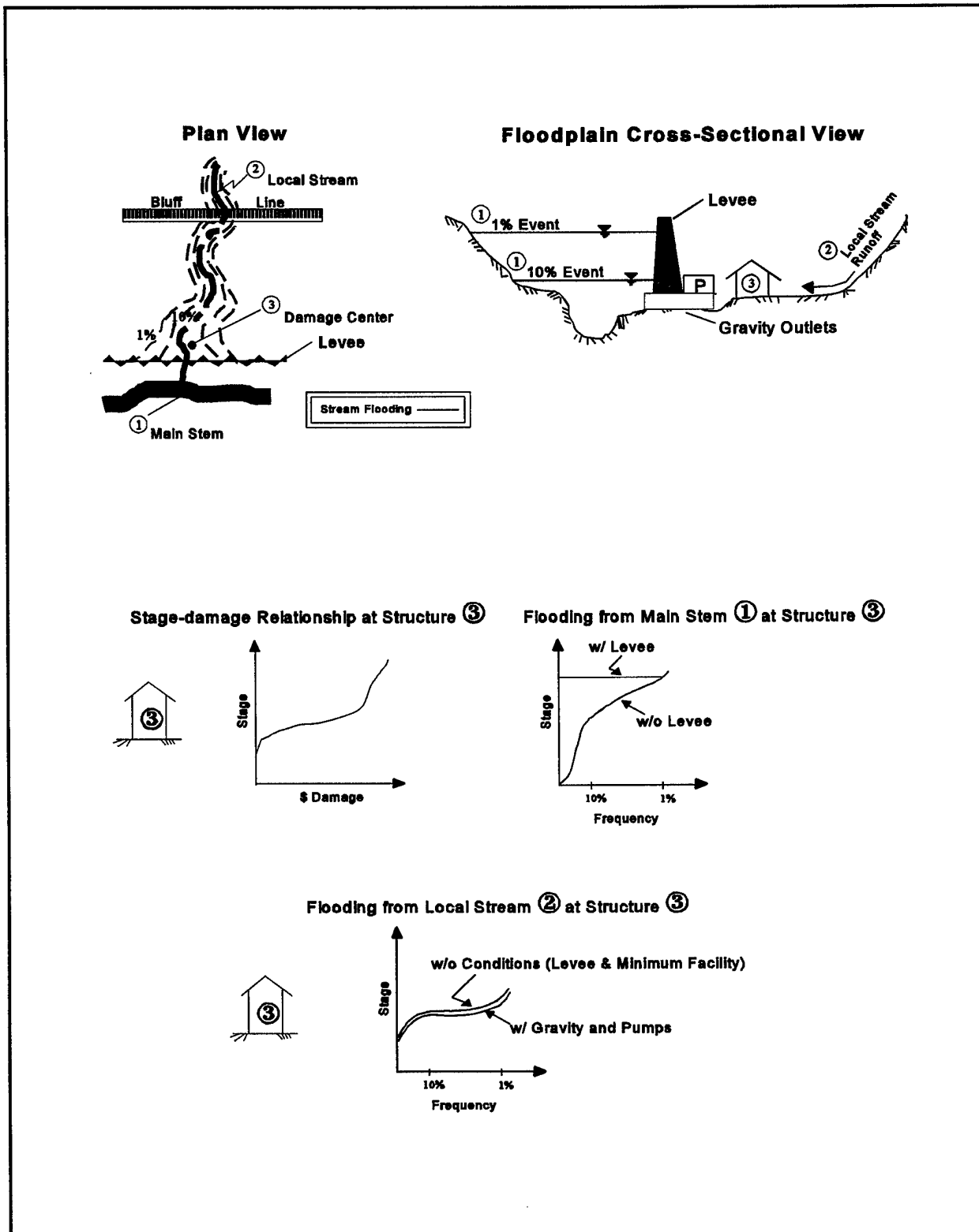
Figure 5-1. Interior system with gravity outlets and pumps
