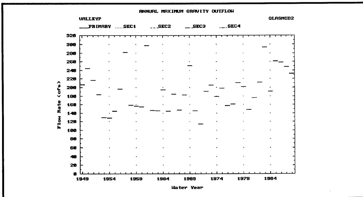
Figure E-11. Maximum annual gravity outflow
