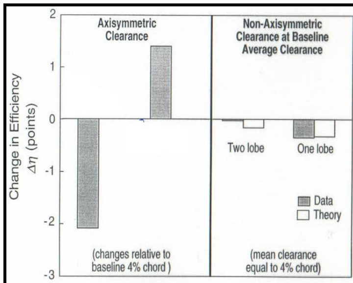
Figure 19 - Changes in peak efficiency with asymmetric clearance, with the flow condition corresponding to the peak efficiency points in next figure
