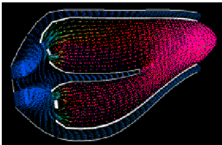
Figure 25 - ALLSPD simulation of a combustor
