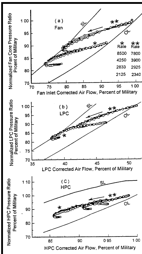
Figure 67 - Ops line migration due to indicating stalling stag temperature ramps
