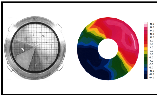
Figure 37 - Imposed distortion pattern, produced by distortion screen
