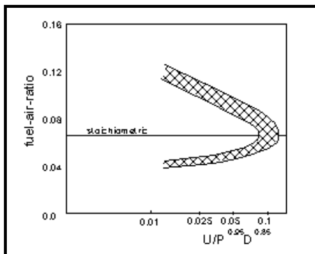
Figure 11 - Stability limits
