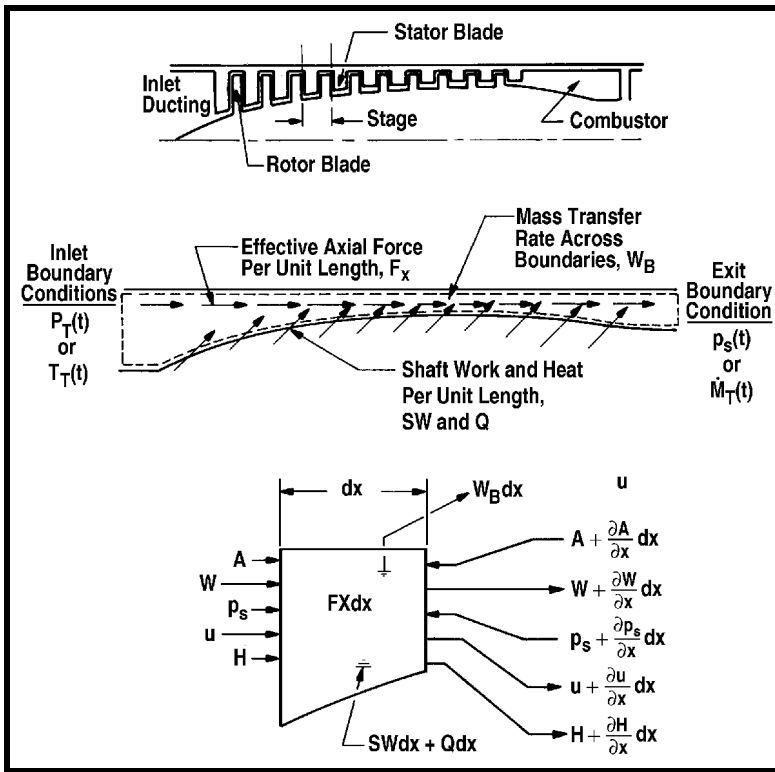
Figure 33 - DYNTTECC control volume technique
