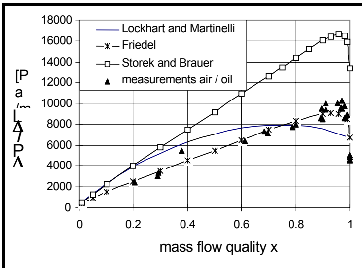
Figure 103 - Comparison of available correlations with air/oil measurements
