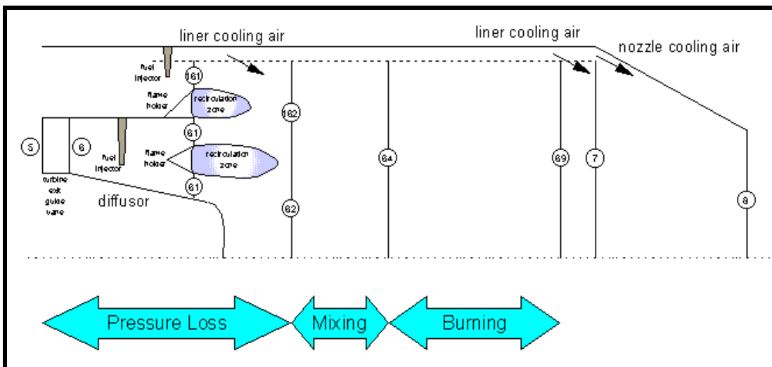
Figure 7 - Afterburner nomenclature
