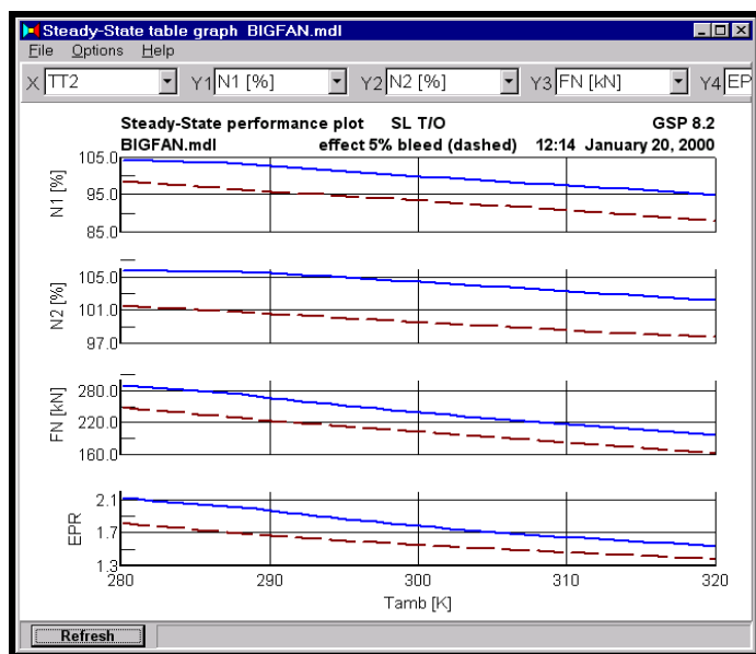
Figure 20 - Effect of compressor bleed on take-off performance
