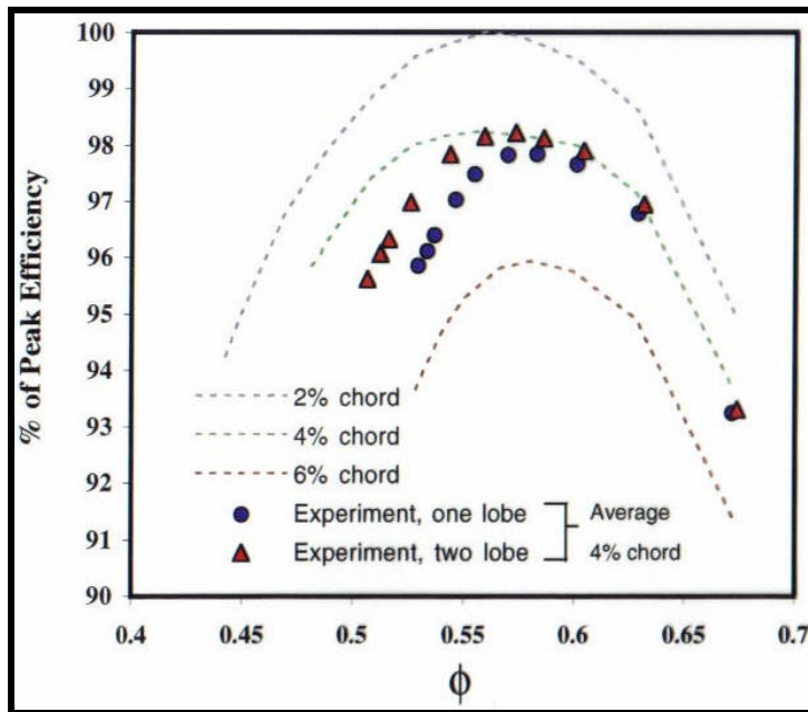
Figure 18 - Effect of tip clearance distribution on compressor efficiency
