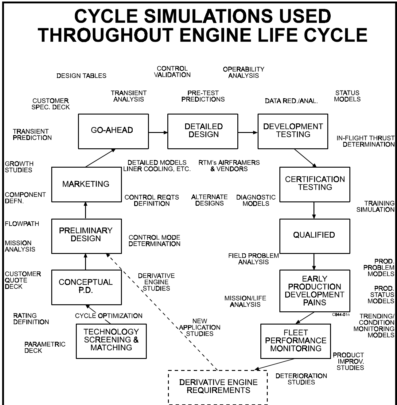
Figure 2 - Engine models used throughout engine life cycle
