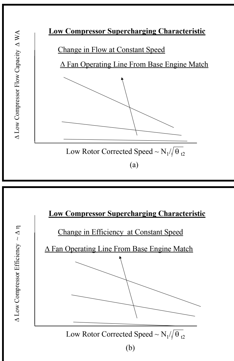
Figure 34 - Super charging curve for primary stream
