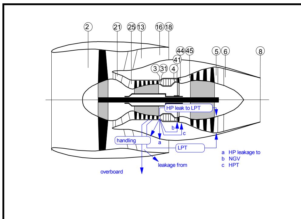
Figure 13 - Nomenclature
