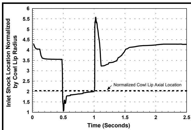
Figure 56 - Inlet shock location
