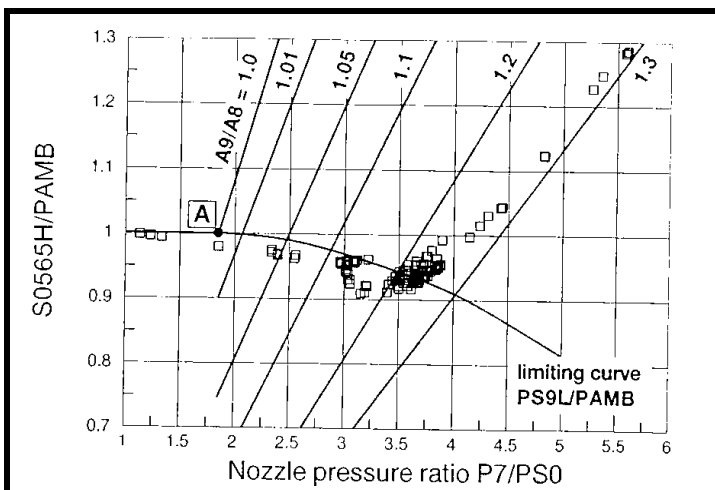
Figure 68 - Correlation of static pressure near the nozzle exit with nozzle pressure ratio
