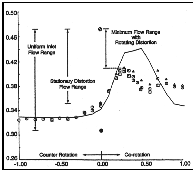
Figure 47 - The effects of co and counter-screen rotation on compressor stability limit
