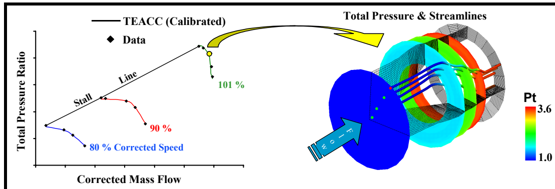
Figure 41 – Point inlet performance and corresponding flow-field for a typical three-stage military fan
