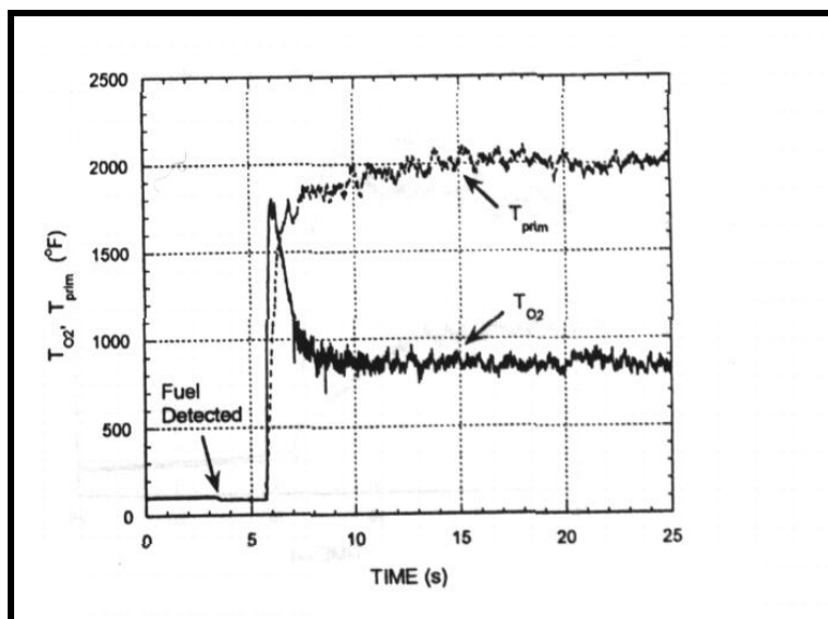
Figure 52 - Ignition event
