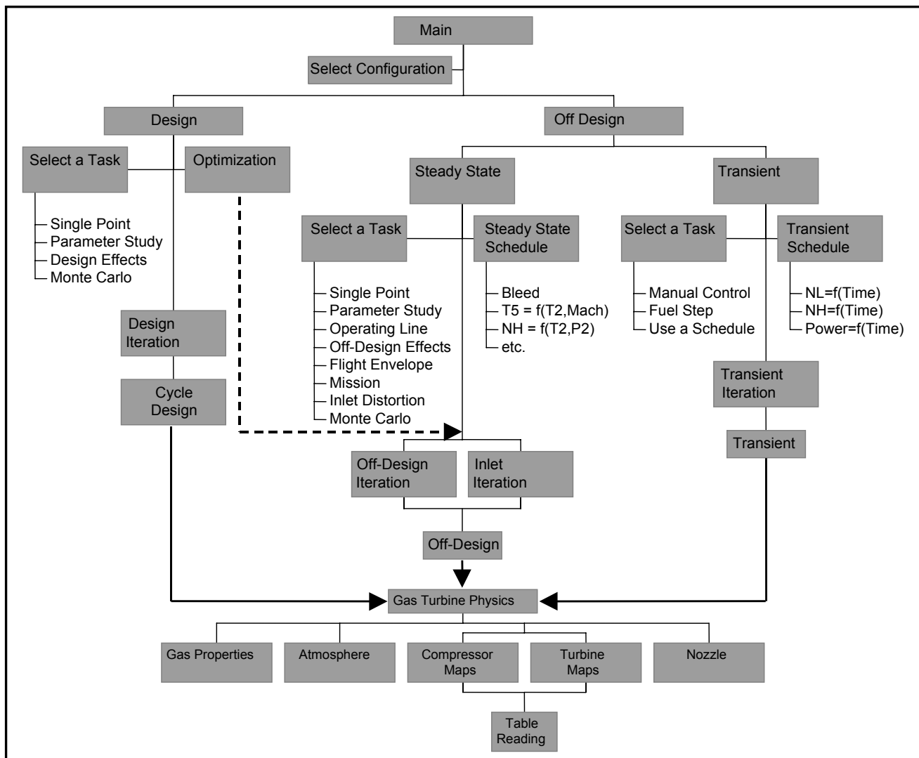
Figure 8 - GasTurb architecture
