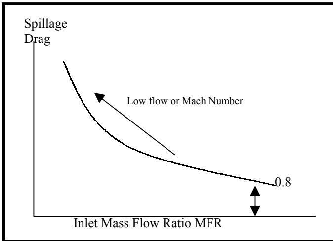
Figure 74 - Inlet spillage drag is a function of mass flow ratio
