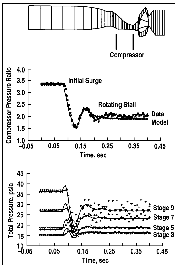
Figure 35 - Post-stall dynamic event - DYNTTECC
