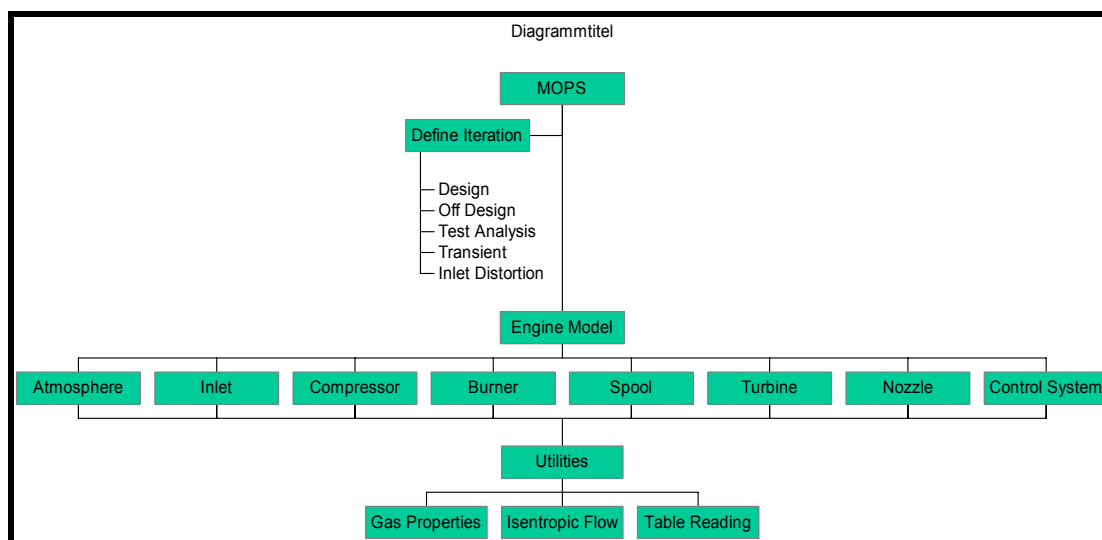
Figure 6 - MOPS architecture
