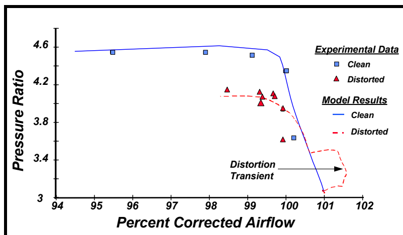
Figure 38 - Model prediction and comparison
