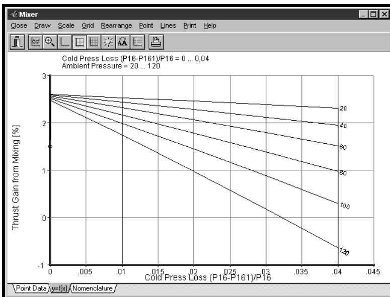
Figure 16 - Effect of nozzle back pressure on theoretical thrust gain ( P_8=200\text{kPa} )
