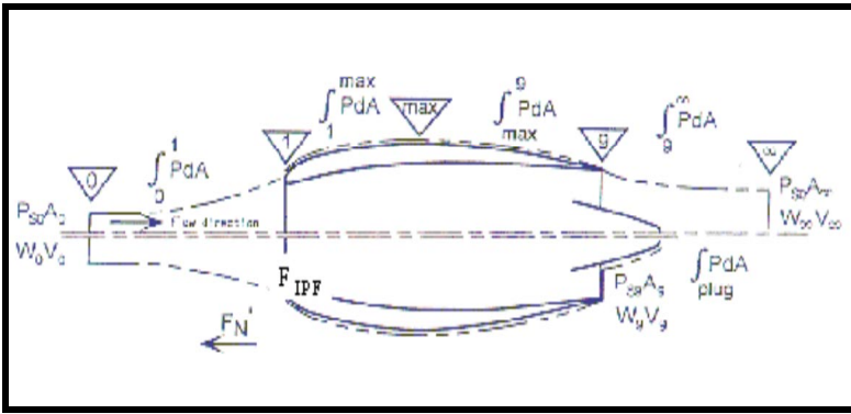
Figure 47 - Single stream control volume for thrust definition
