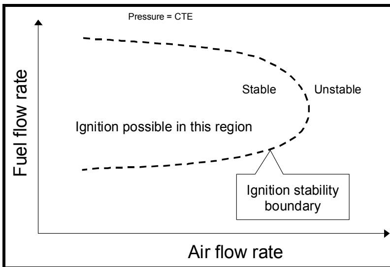
Figure 44 – Region of stable ignition
