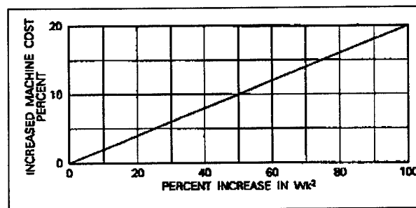
Figure 3-3. Effect of increased Wk^2 on generator cost (included by permission of Westinghouse Electric Corp)
