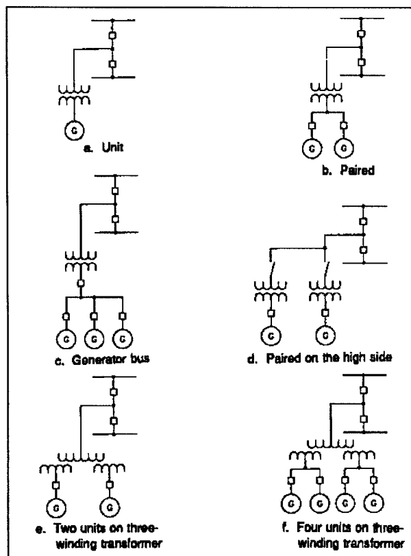
Figure 2-1. Main unit switching schemes
