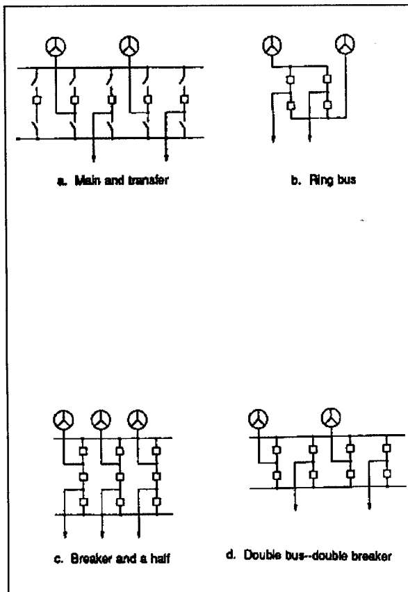
Figure 5-1. Switchyard bus arrangements
