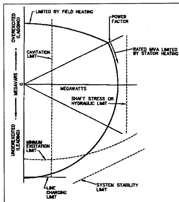
Figure 3-1. Typical hydro-generator capability curve
