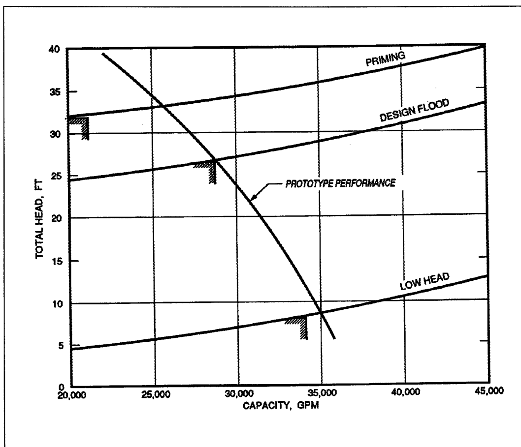
Figure B-5. Prototype performance curve superimposed on the system head curves (pump bowl) pump MF-1
