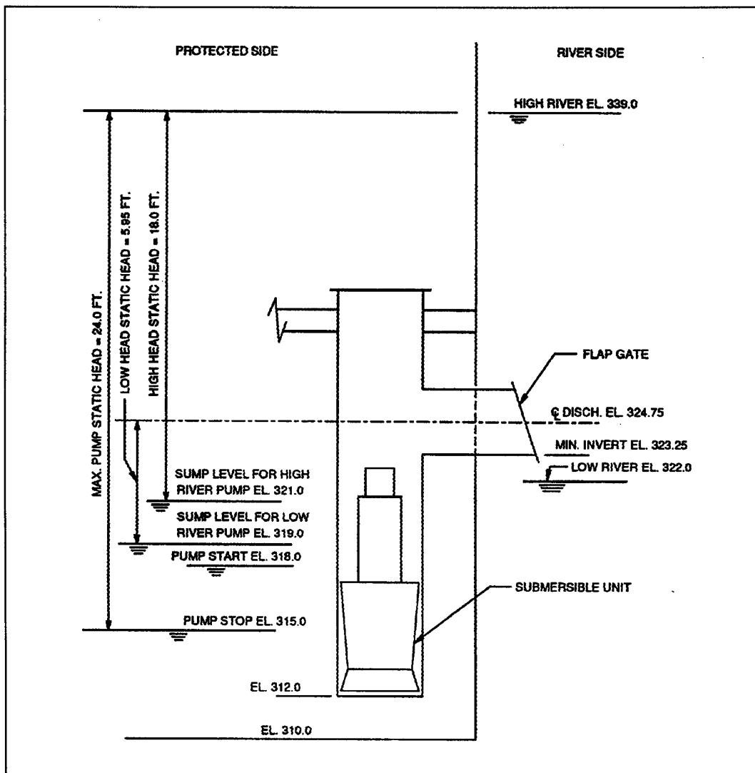
Figure B-8. Static head diagram
