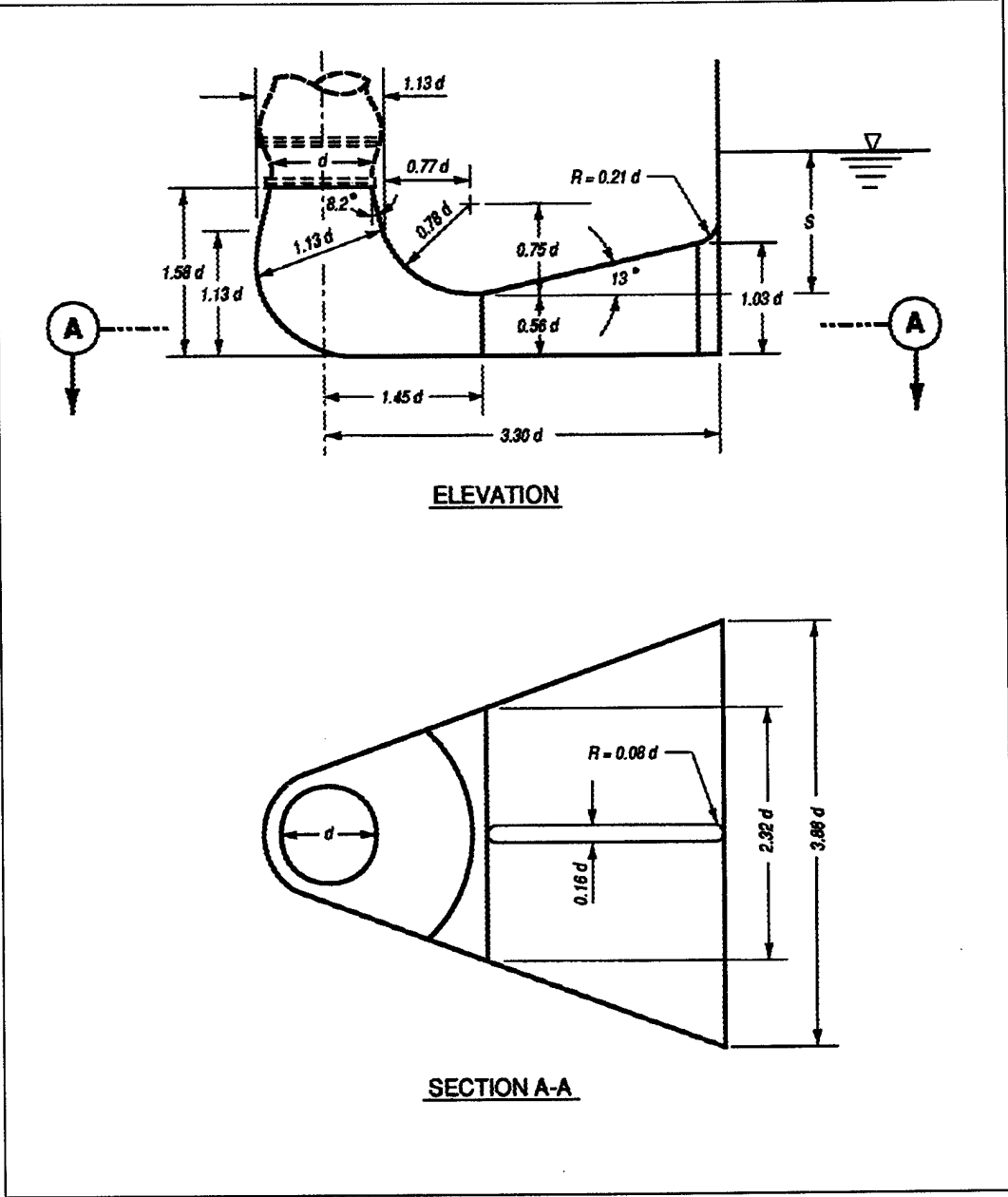
Figure B-12. Typical formed suction intake
