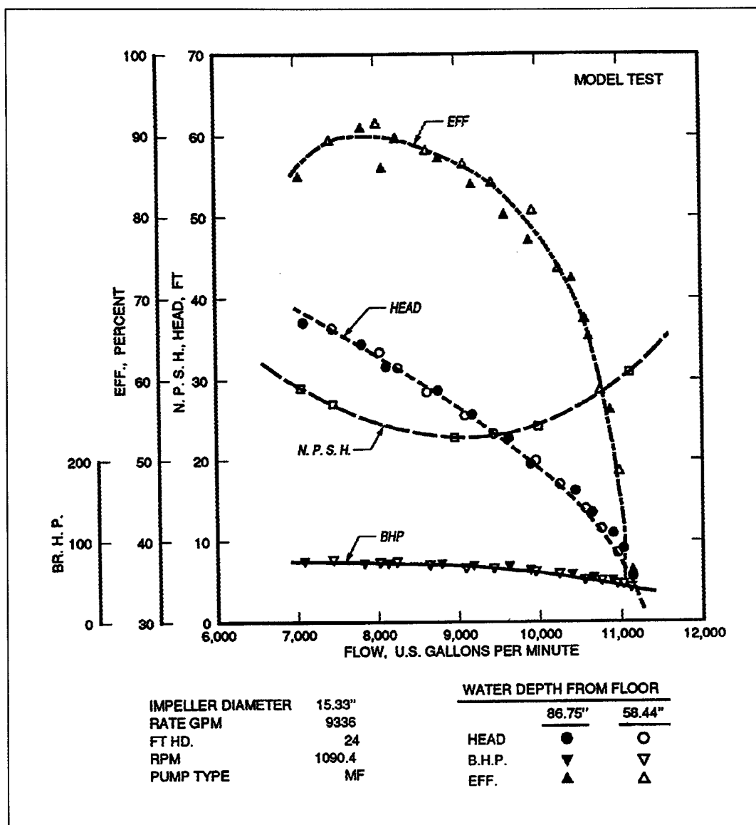
Figure B-4. Pump model curve MF-1
