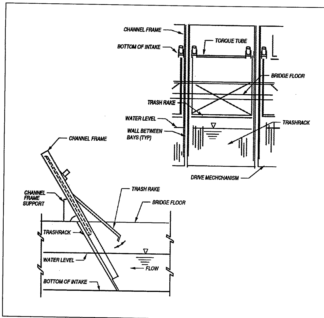
Figure C-4. Mechanical climber screen arrangement
