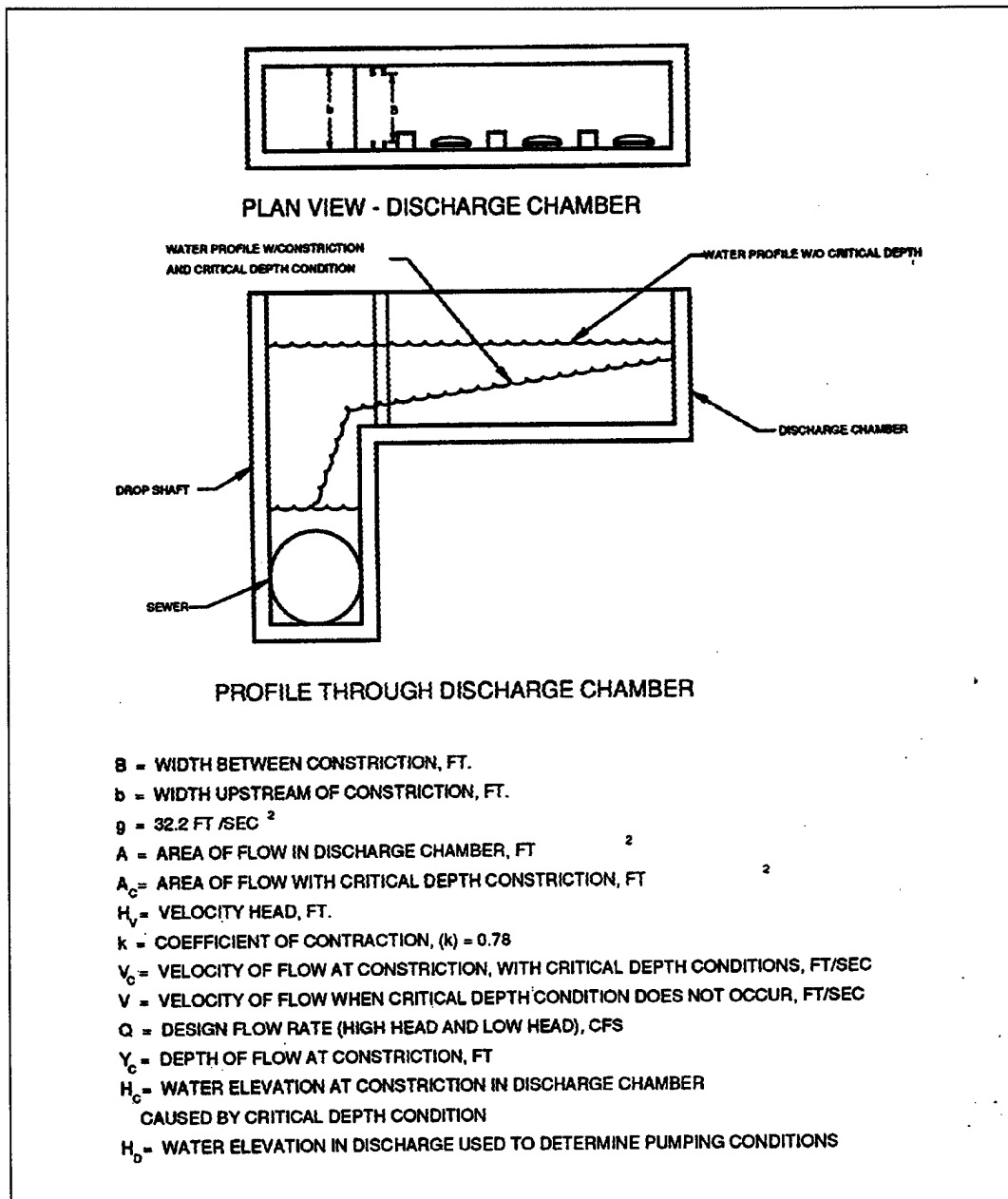
Figure E-1. Discharge chamber critical depth
