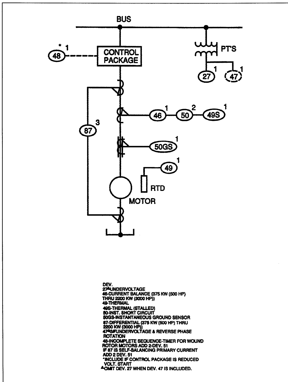
Figure 15-1. Recommended minimum protection for medium-voltage induction motors (all horsepower except as noted)
