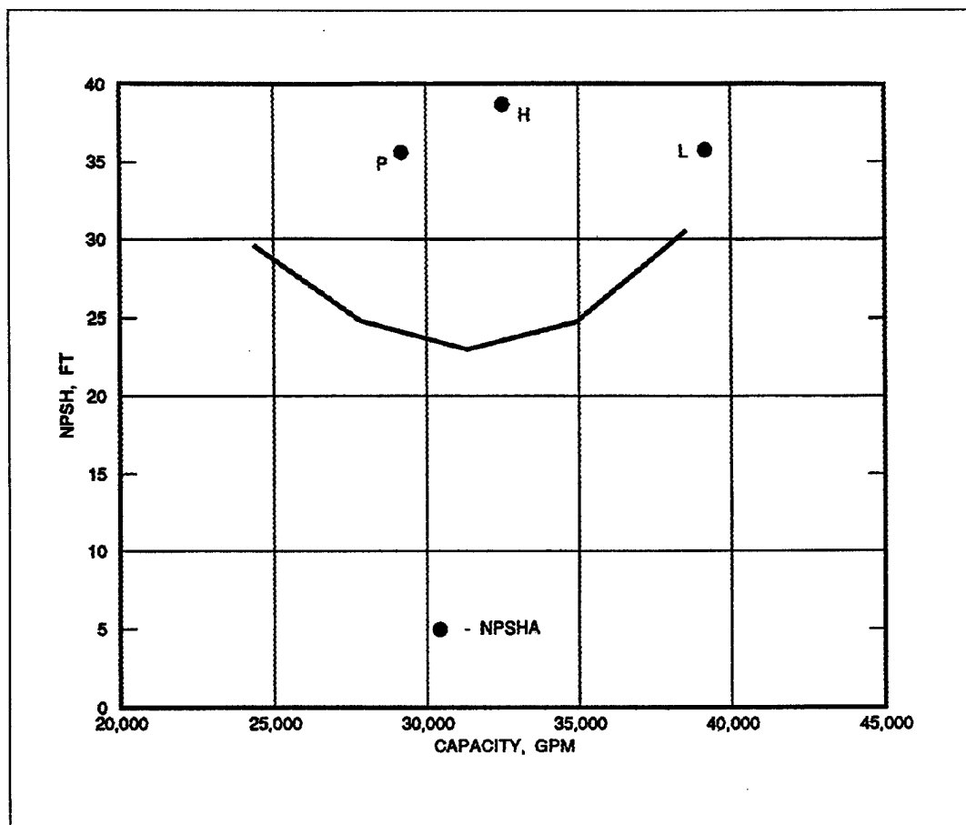
Figure B-6. Cavitation curve MF-1
