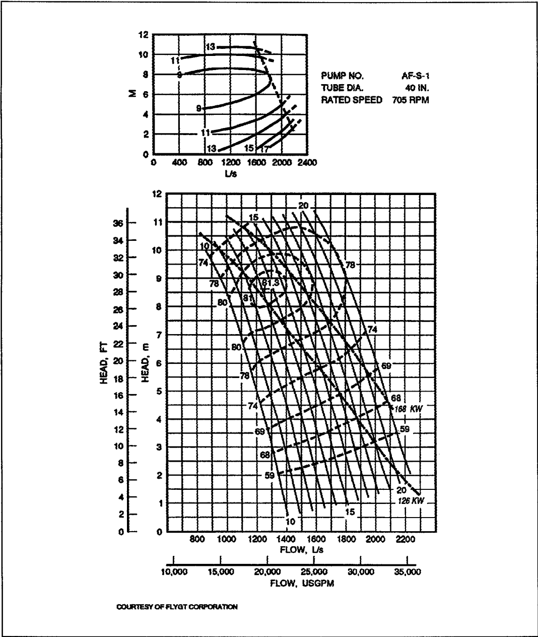
Figure B-10. Submersible pump curve AF-S-1
