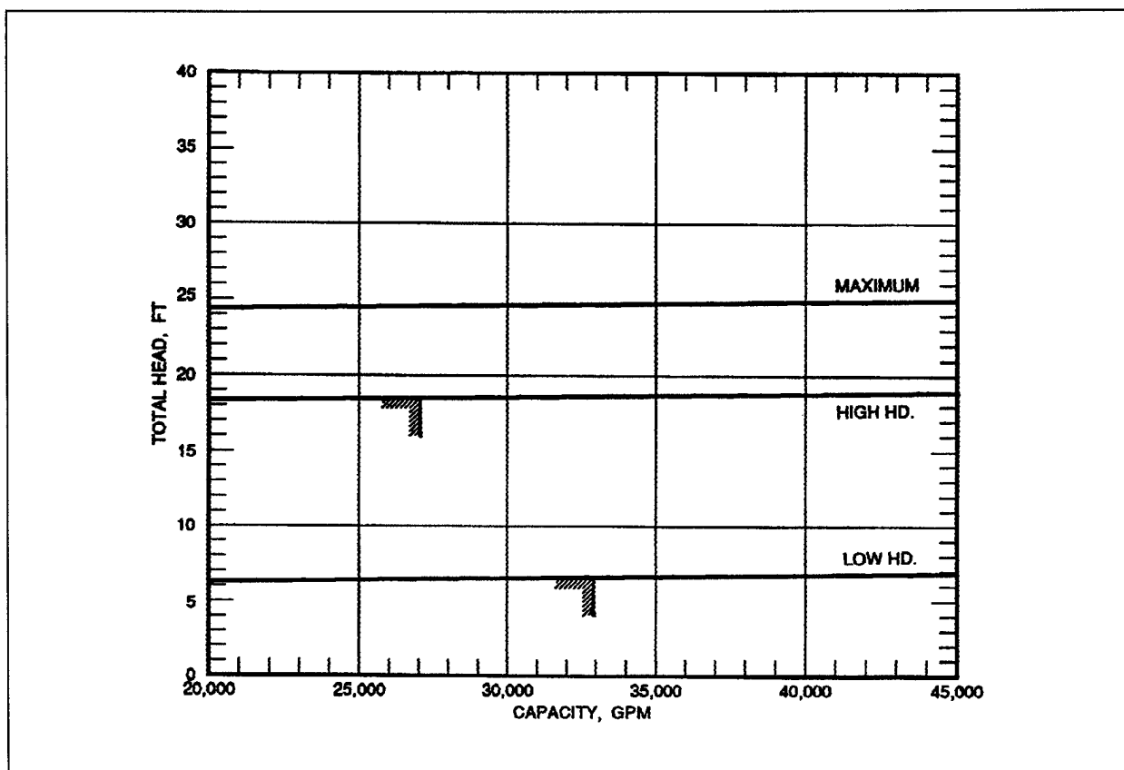
Figure B-9. System head loss curves
