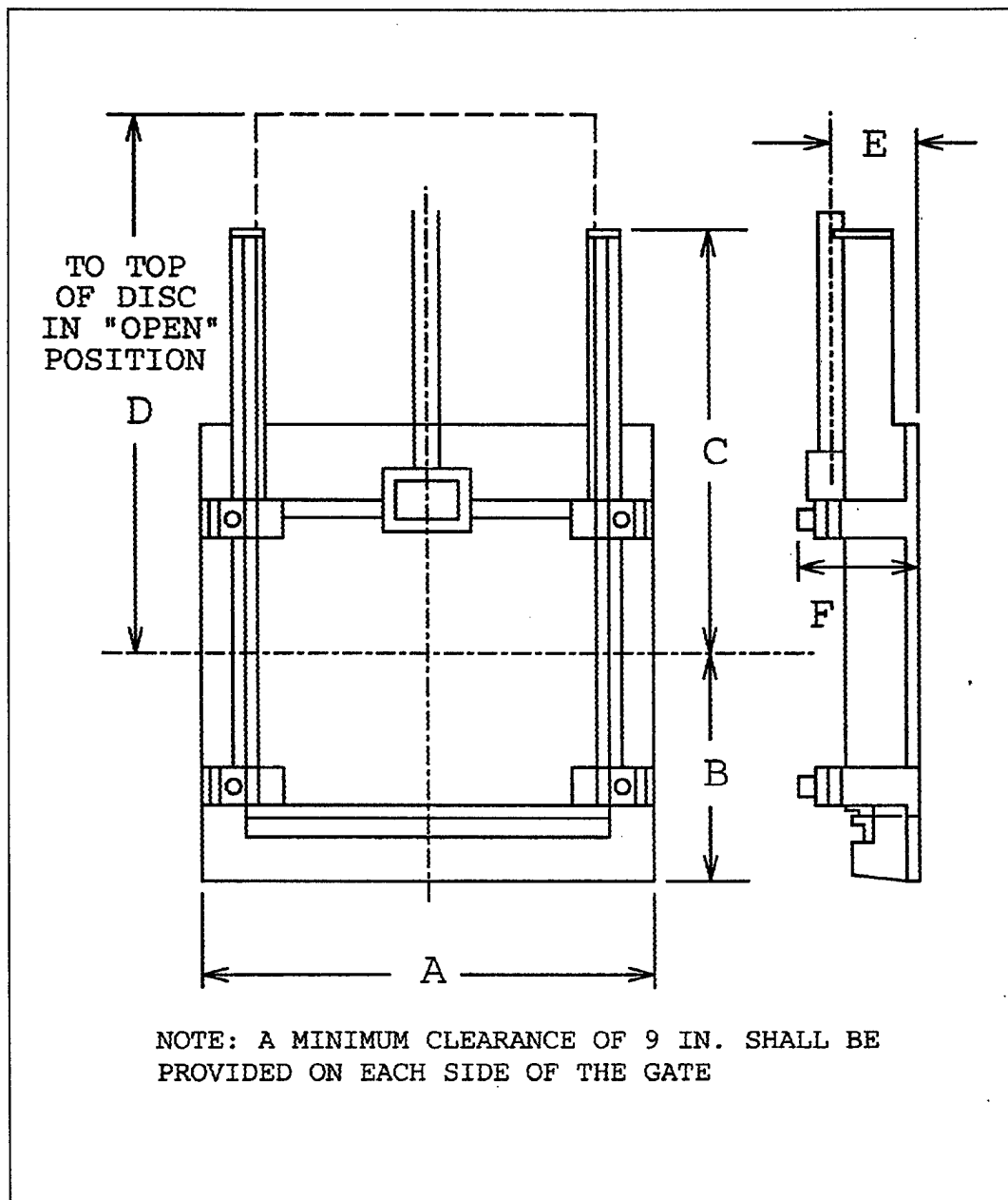
Figure D-2. Sluice gate layout
