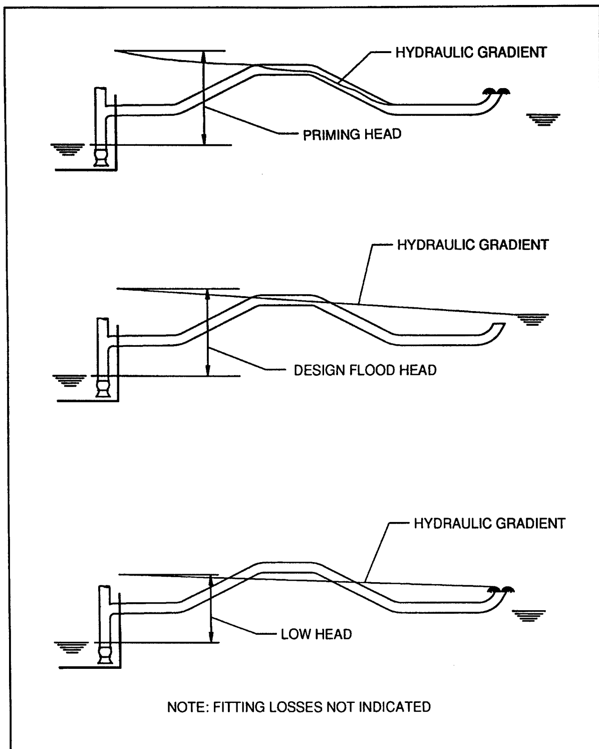
Figure B-1. Discharge pipe system
