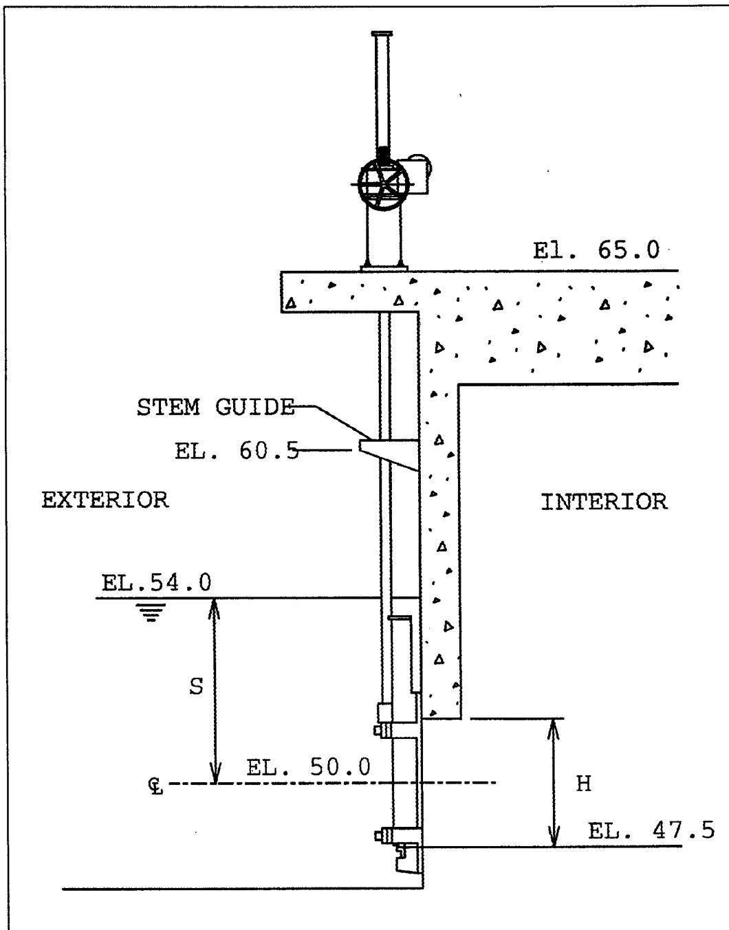
Figure D-1. Sluice gate and operator
