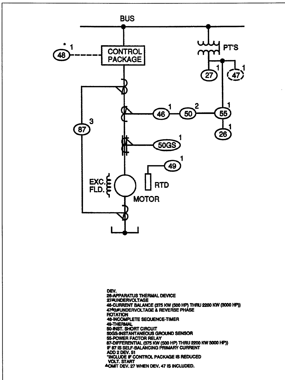
Figure 15-2. Recommended minimum protection for medium-voltage brushless synchronous motors (all horsepowers except as noted)
