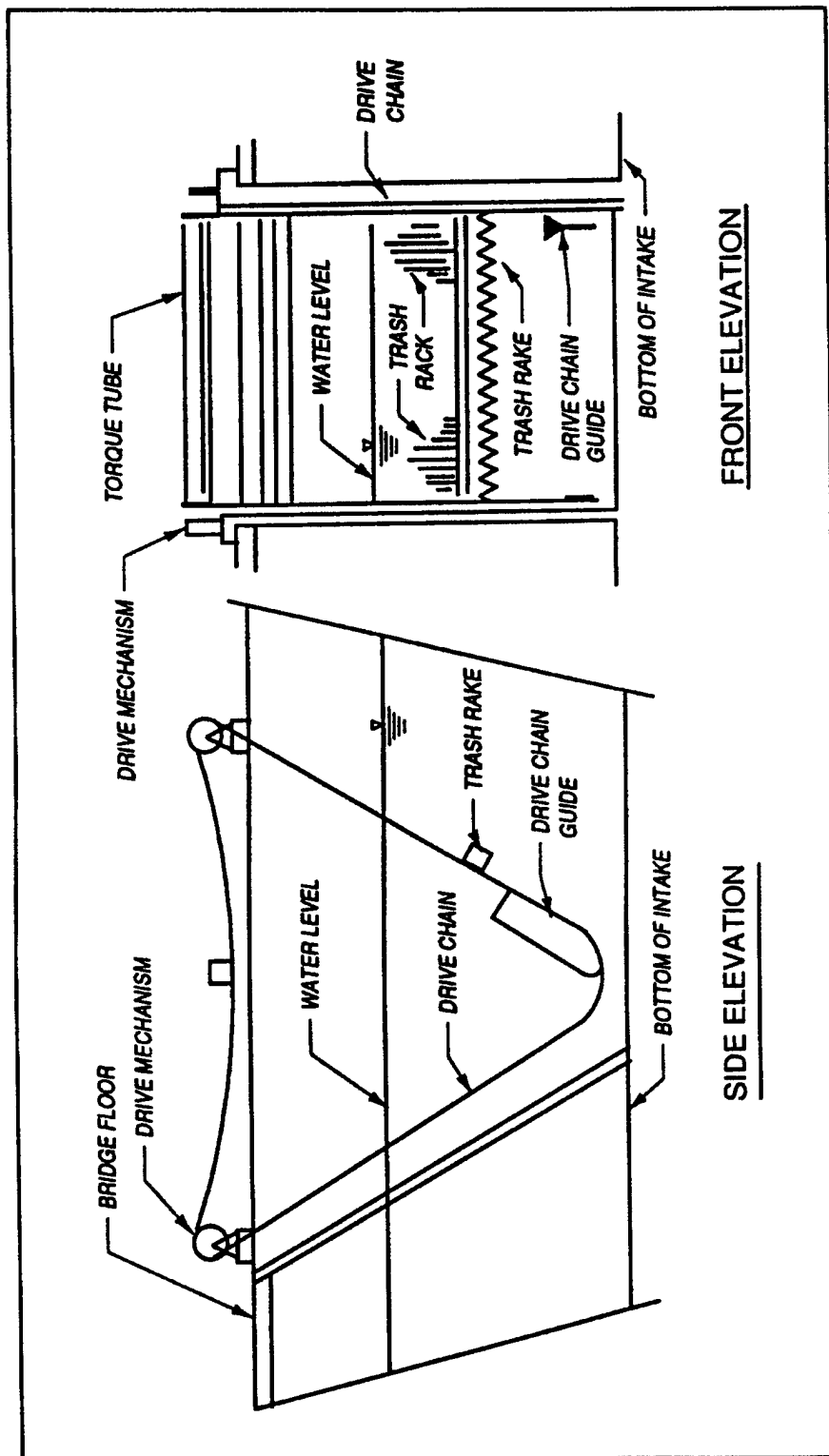
Figure C-3. Guided catenary arrangement
