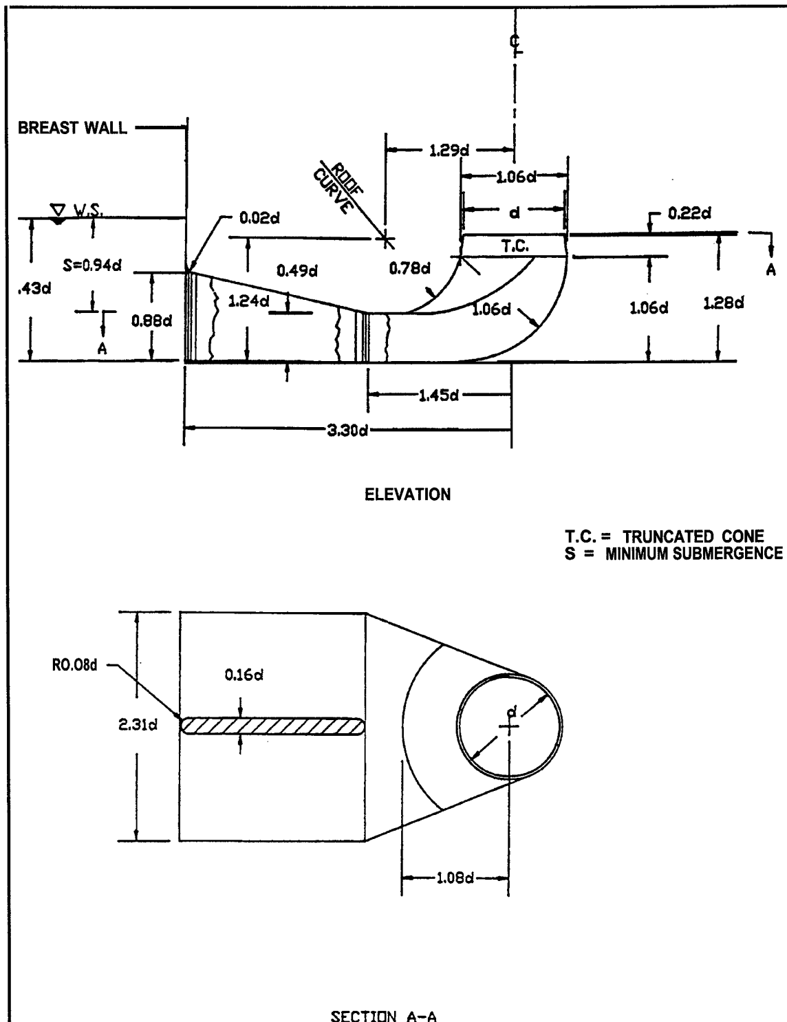
Figure I-2. FSI type 10 design
