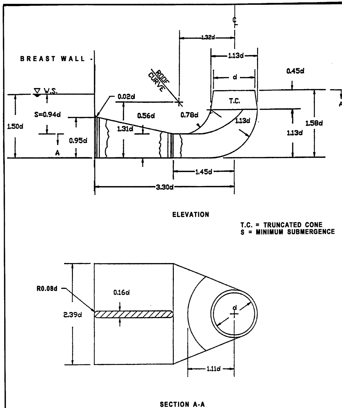
Figure I-1. FSI type 1 design
