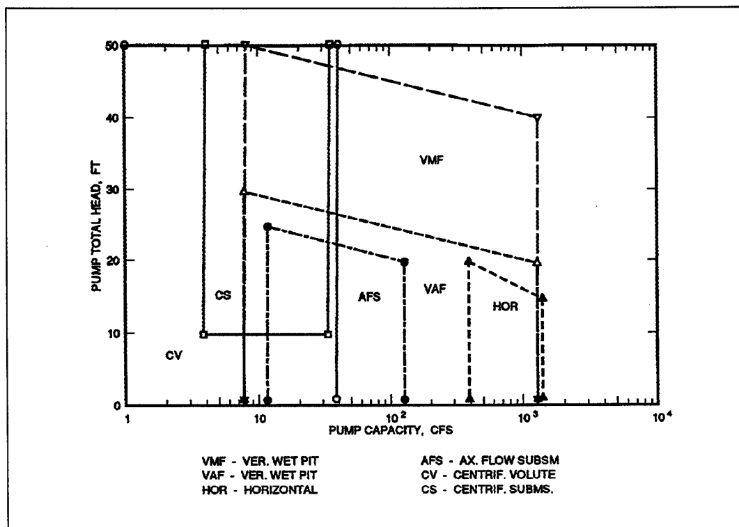
Chart B-1. Operating range of typical pumps
