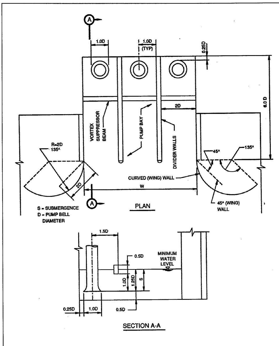
Chart B-2. Vertical pump sump dimensions
