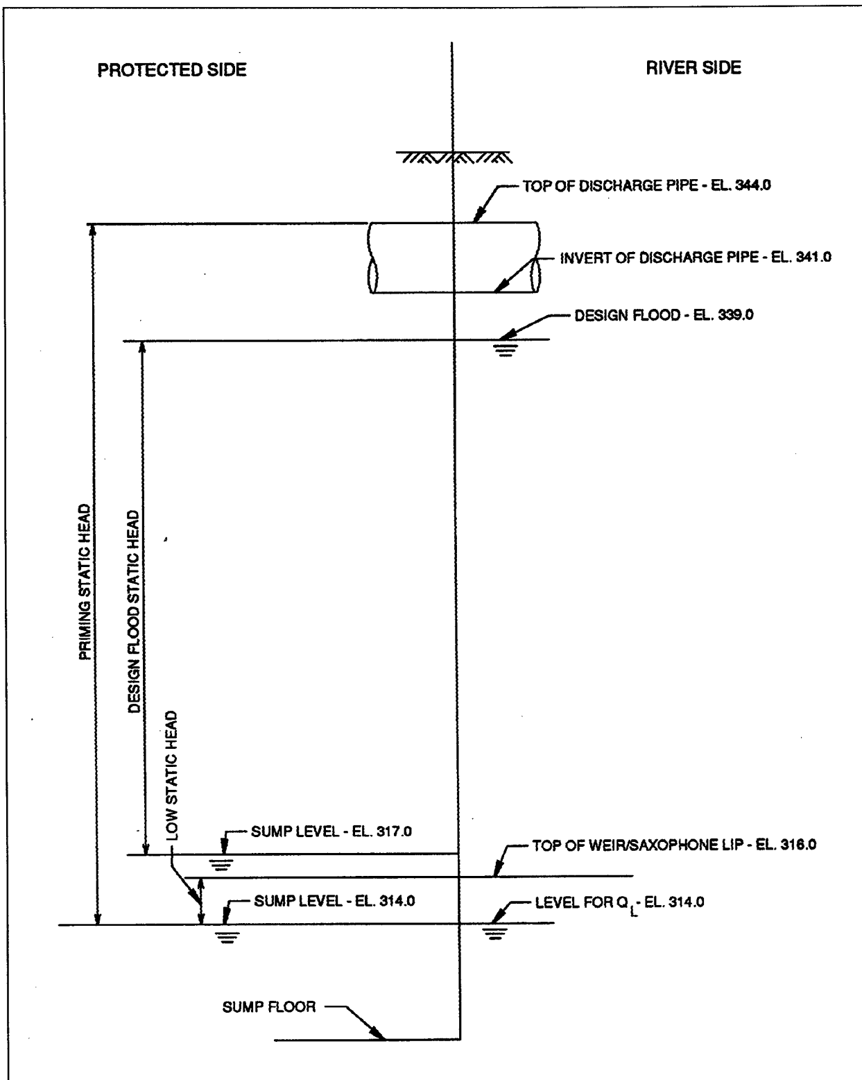
Figure B-2. Construct the static head diagram
