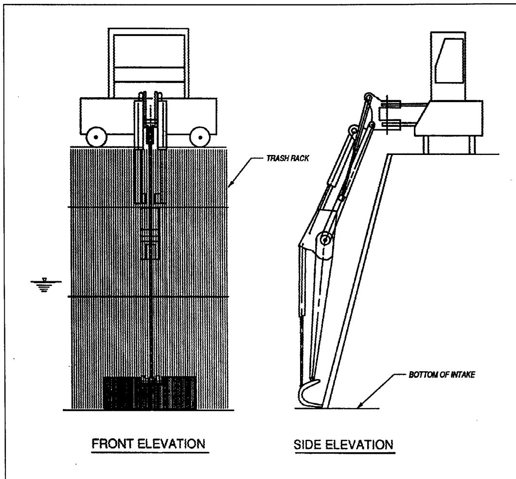
Figure C-5. Mechanical elbow arm arrangement
