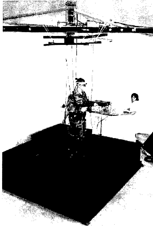
Figure 5. The Omni-Directional Treadmill with the sound enclosure.
