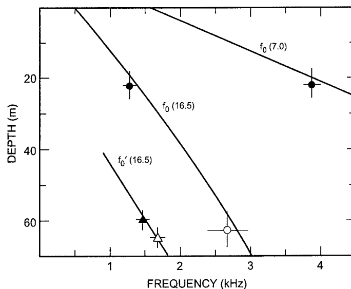
Fig. 5— Measured resonance frequencies of dispersed sardines at night (●) and dawn (○); schools of sardines during night (▲) and day (Δ) as a function of depth; and theoretical calculations of f_0 of 7.0- and 16.5-cm-long dispersed sardines, and f_0' of 16.5-cm-long sardines in schools.
