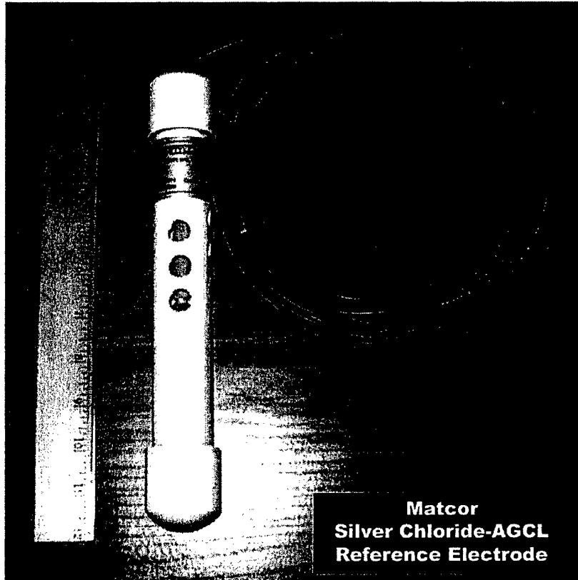
Figure 23. Matcor permanent reference electrode.
