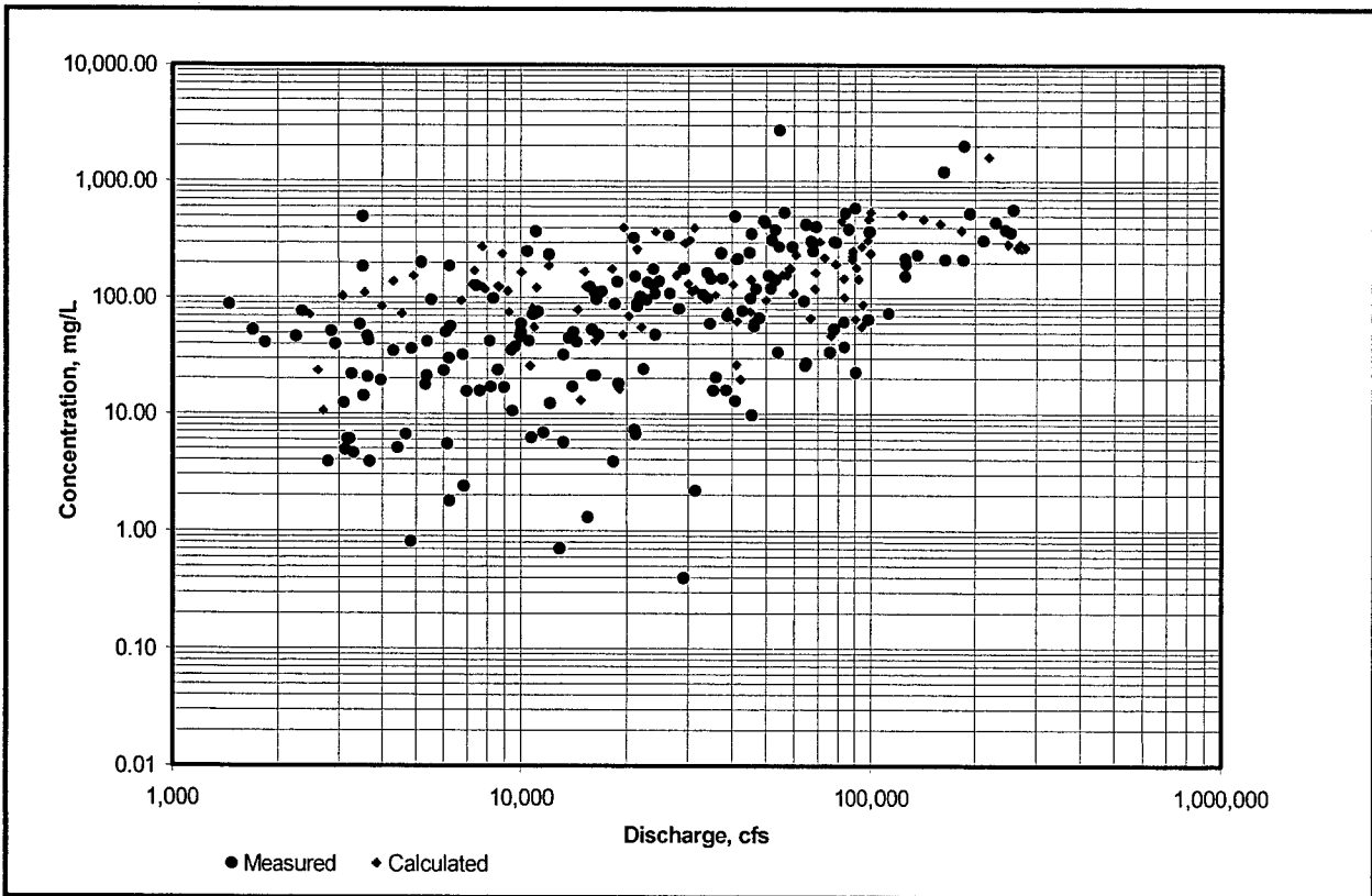
Figure 13. Comparison of measured and calculated very-fine sand transport at Fulton, AR, 1984-1996
