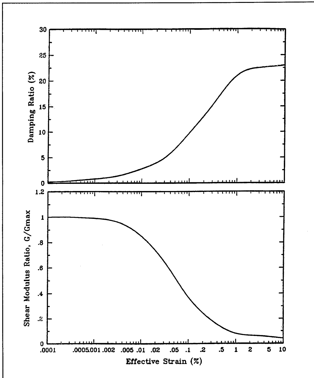
Figure E-3. Variation of shear modulus and damping ratio with shear strain for sand (Seed and Idriss 1970, courtesy of Earthquake Engineering Research Center, University of California at Berkeley)
