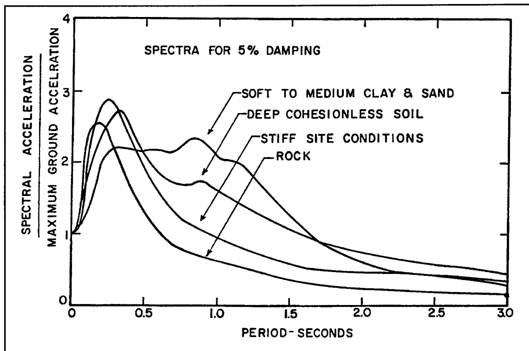
Figure 3-10. Average acceleration spectra for different site conditions (Seed, Ugas, and Lysmer 1976, courtesy of Seismological Society of America)
