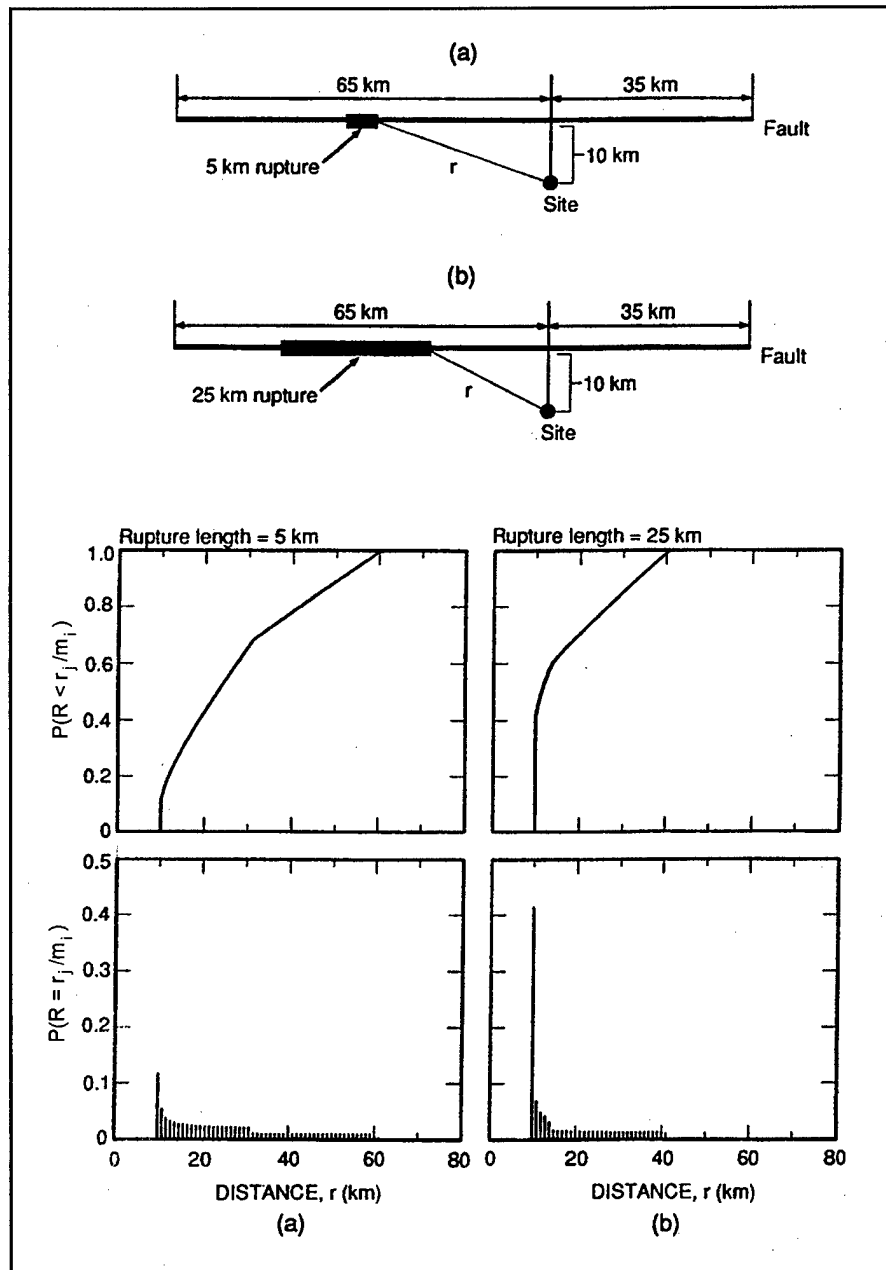
Figure 3-25. Illustration of distance probability distribution
