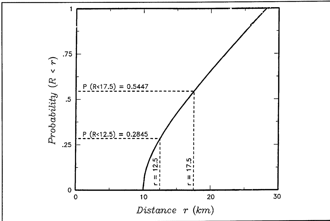
Figure G1-3. Example distance probability calculation
