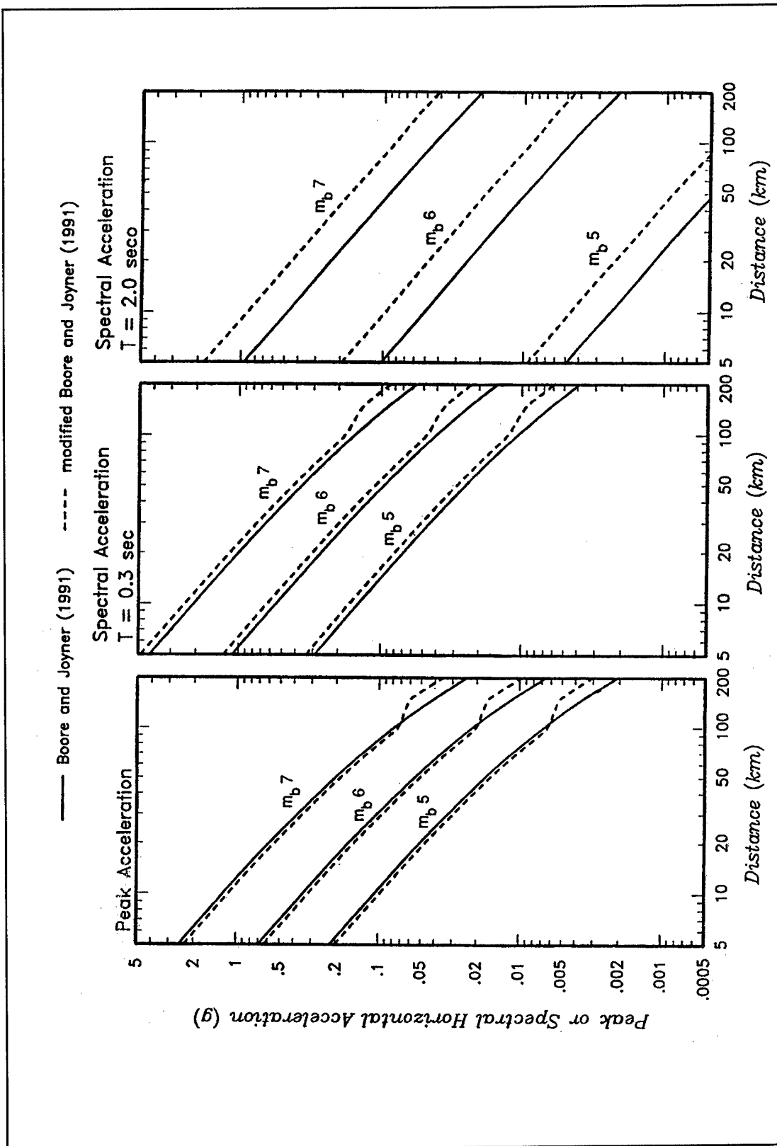
Figure G3-6. Attenuation relationships
