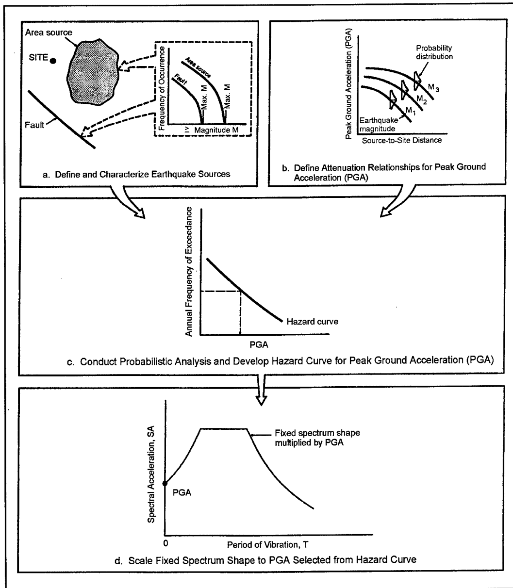
Figure 3-21. Development of response spectrum based on a fixed spectrum shape and a probabilistic seismic hazard analysis for peak ground acceleration
