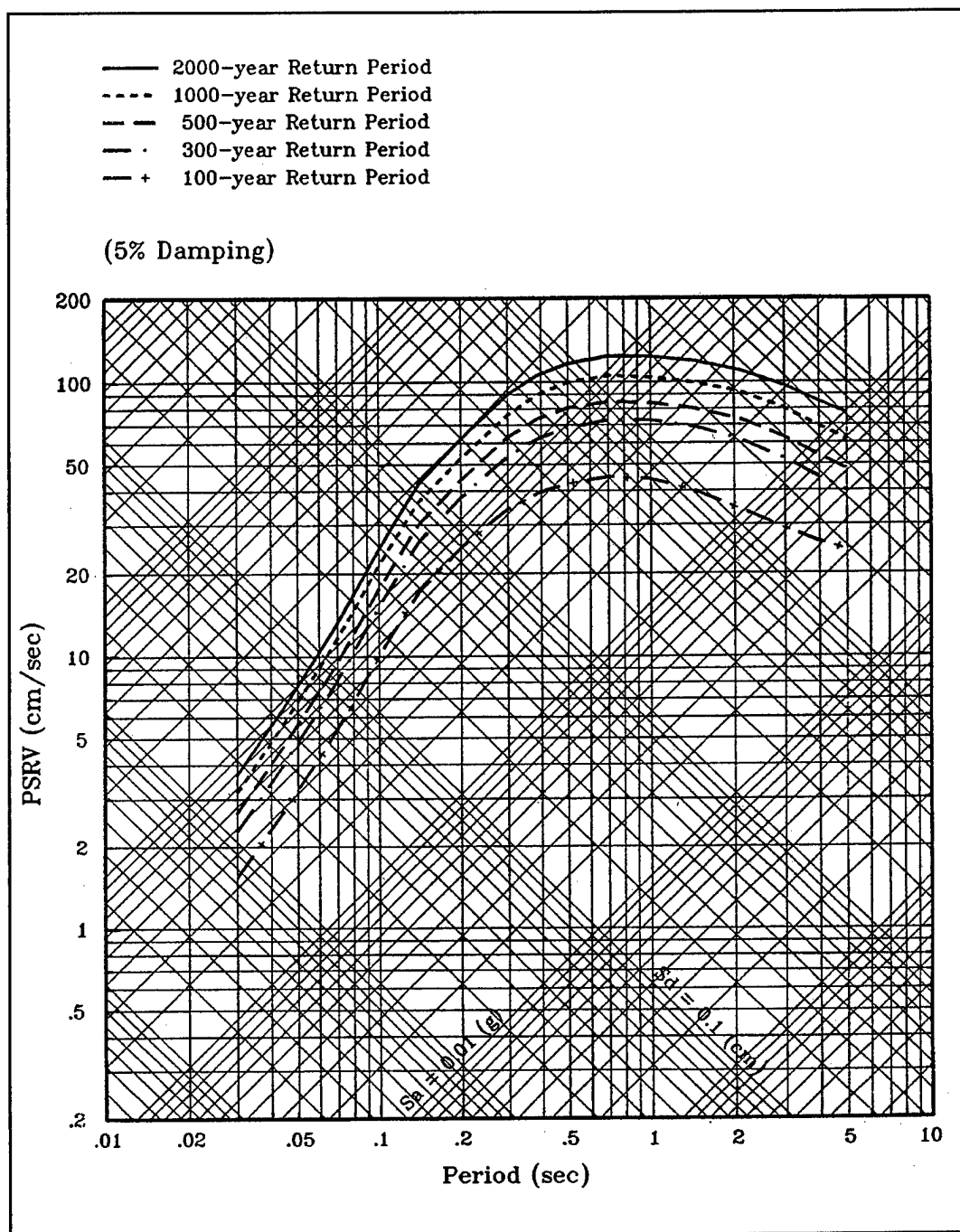
Figure G2-13. Equal-hazard pseudo-relative velocity (PSRV) response spectra for the site (5 percent damping)
