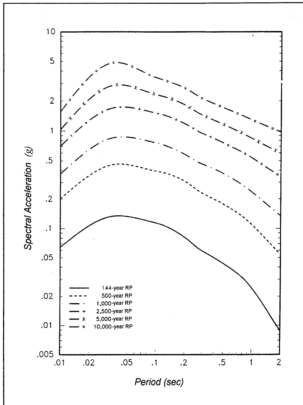
Figure G4-8. Equal-hazard response spectra (5 percent damping)
