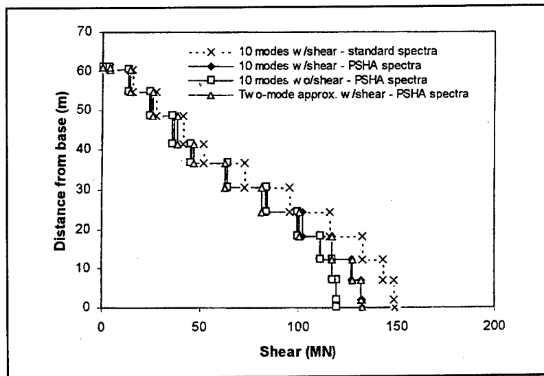
Figure H-13. Maximum shears due to 1000-year San Francisco Bay area response spectra applied along y-axis (longitudinal direction)
