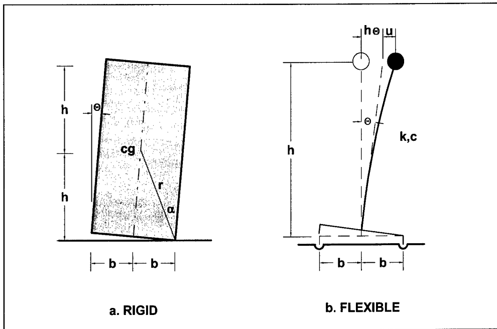
Figure 2-12. Rigid block and SDOF models for rigid and flexible structures
