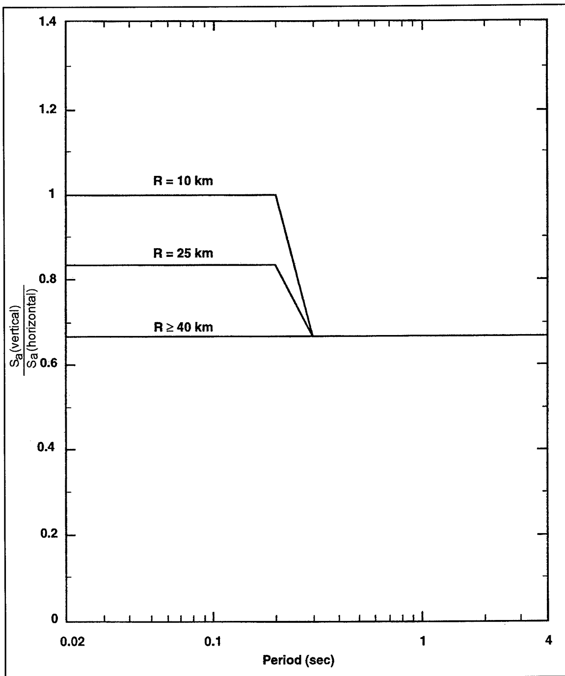
Figure 3-16. Simplified relationships between vertical and horizontal response spectra as a function of distance R
