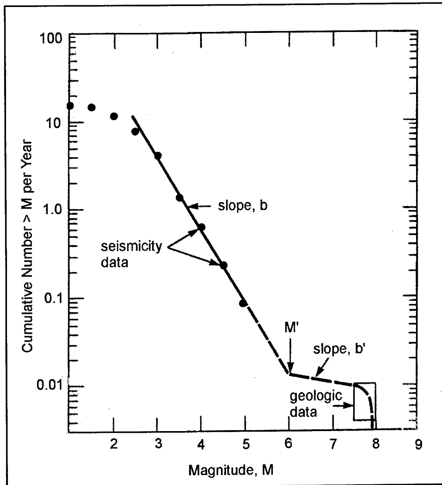
Figure 3-27. Diagrammatic characteristic earthquake recurrence relationship for an individual fault or fault segment. Above magnitude M' a low b value ( b' ) is required to reconcile the small-magnitude recurrence with geologic recurrence, which is represented by the box (Schwartz and Coppersmith 1984; National Research Council 1988)
