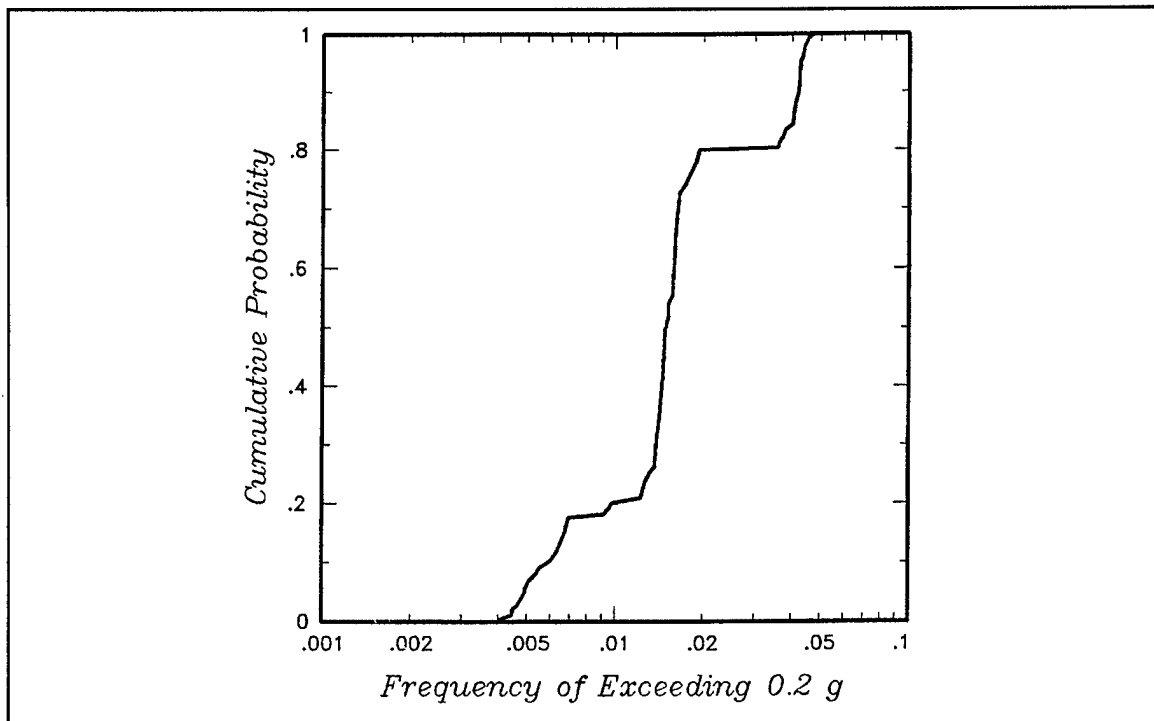
Figure G1-5. Exceedance frequency probability distribution
