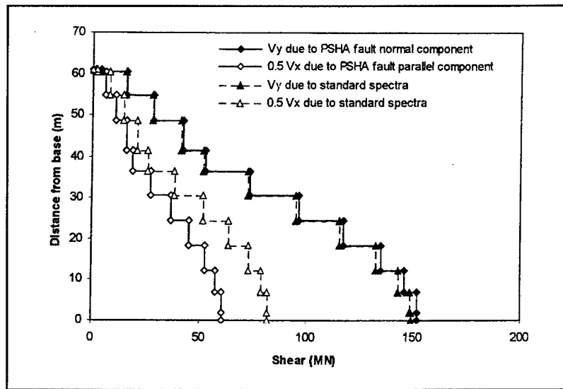
Figure H-17. Combination of shear forces 0.5V_x and V_y for site-specific and standard ground motions
