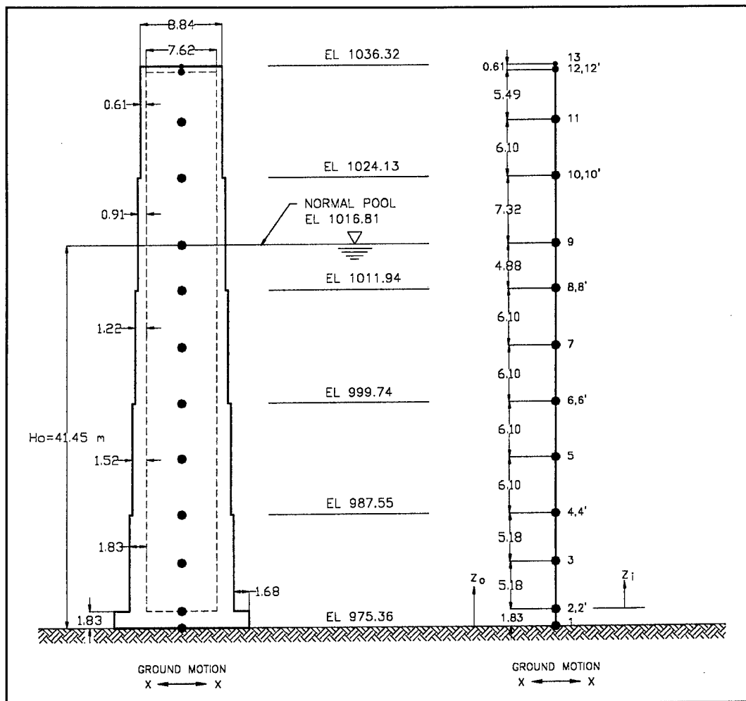
Figure H-3. Structural idealization for excitation along transverse axis (x-axis)
