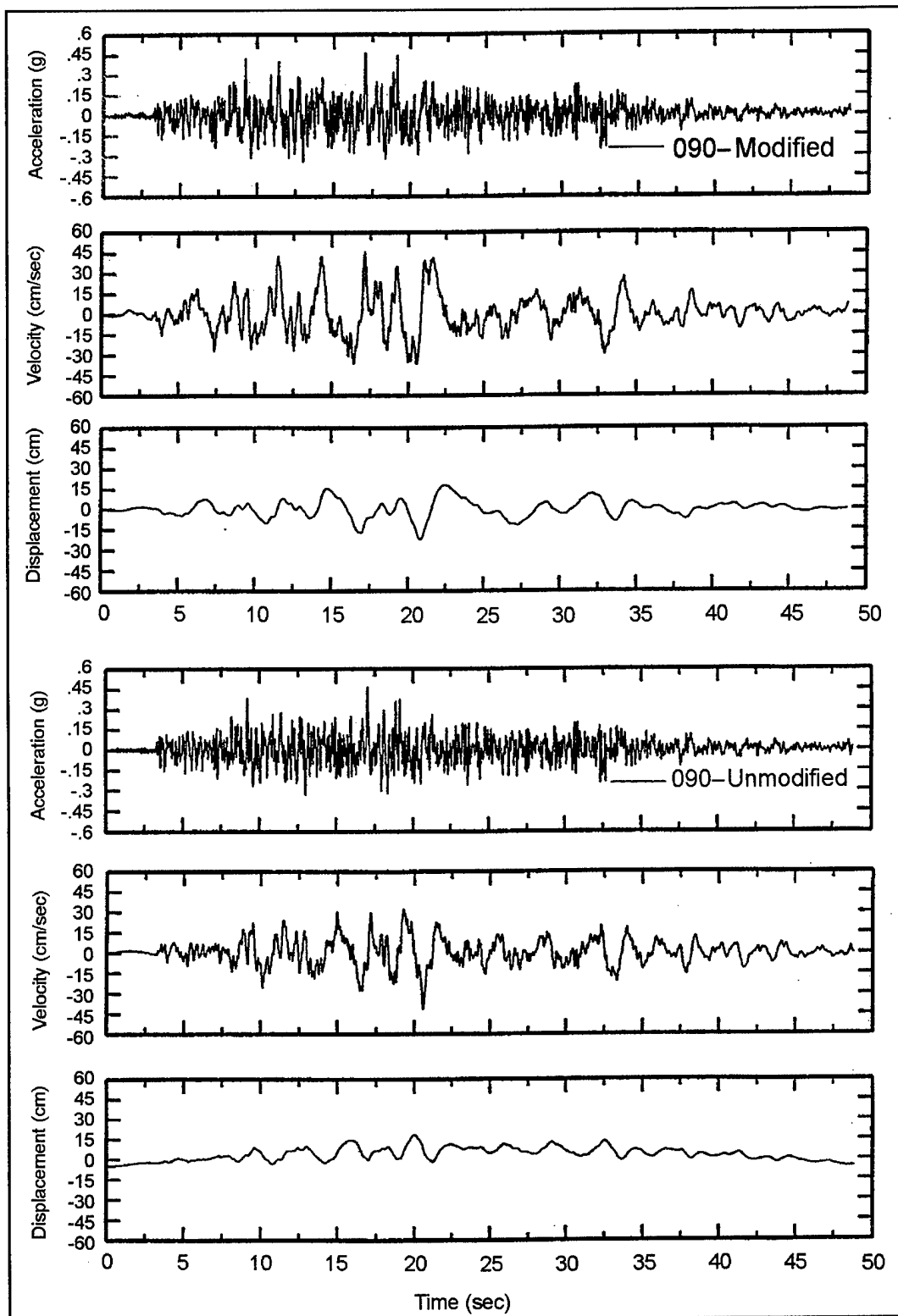
Figure 3-17. Example of original time-histories and time-histories after a spectral matching process
