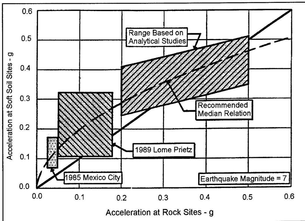
Figure 3-8. Variation of accelerations on soft soil sites versus rock sites (Idriss 1991a, courtesy of I. M. Idriss and Shamsheer Prakesh, ed.)
