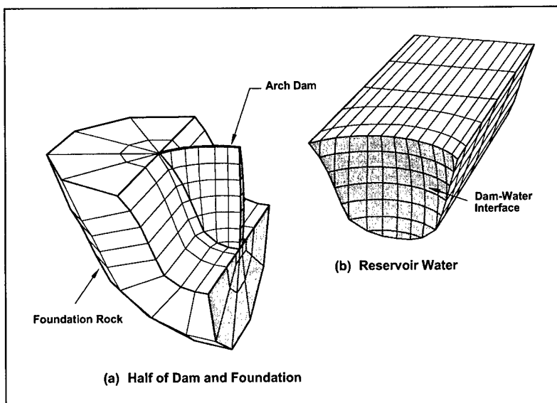
Figure 2-8. 3-D model of arch dam-water-foundation system
