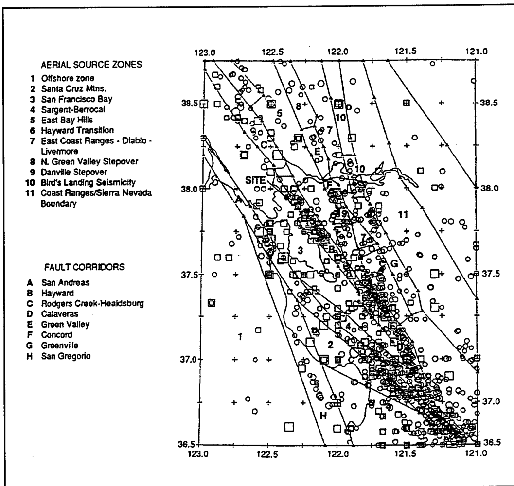
Figure G2-2. Map of the San Francisco Bay area showing independent earthquakes, fault corridors, and areal source zones. Fault corridors define the area within which seismicity is assumed to be related to fault-specific sources
