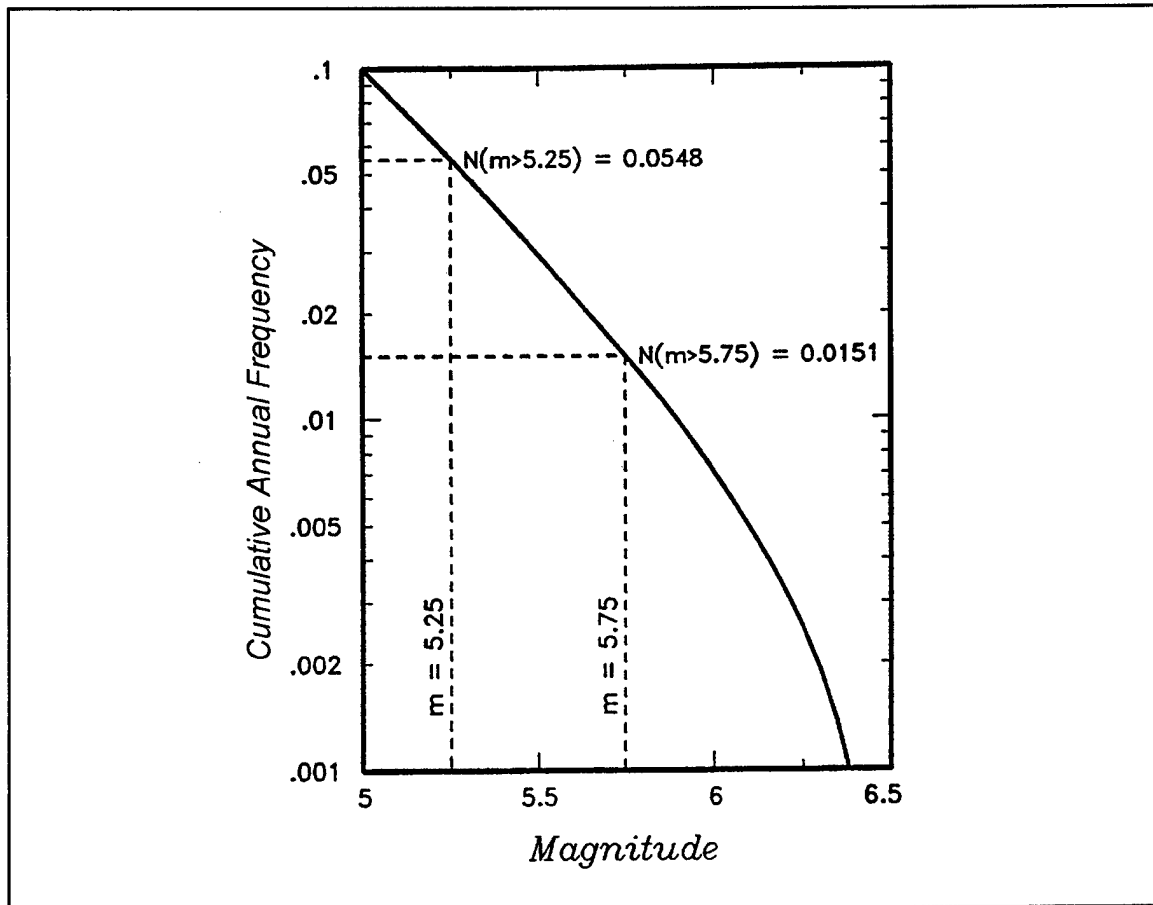
Figure G1-2. Example recurrence rate calculation
