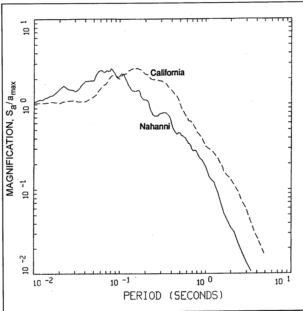
Figure 3-11. Comparison of average 5 percent damped response spectral shapes ( S_a / a_{max} ) computed from strong-motion data recorded at rock sites in Nahanni, Canada, and California for M_w 5.3 earthquakes (Darragh et al. 1989)
