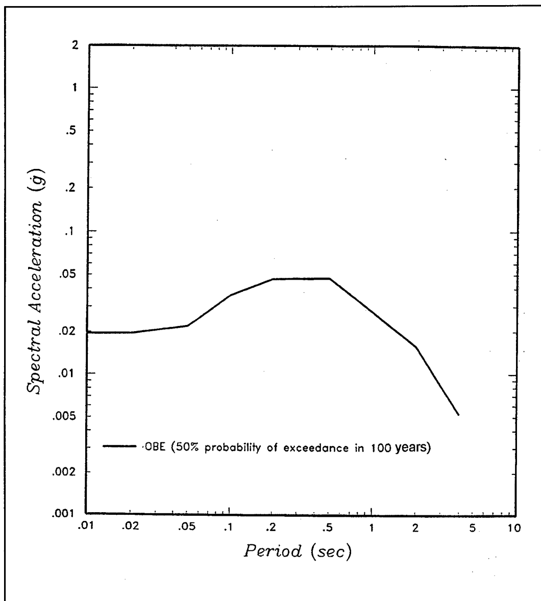
Figure G3-13. OBE spectrum (5 percent damping)
