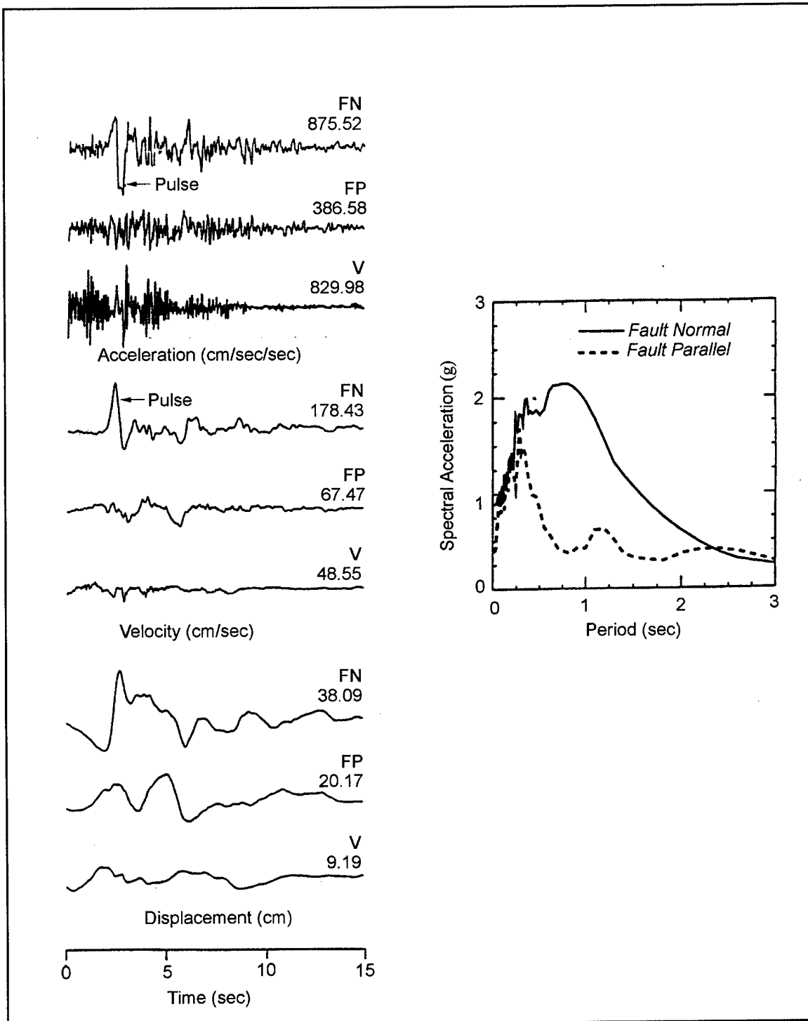
Figure 3-6. Time-histories and horizontal response spectra (5 percent damping) for the fault strike-normal (FN) and fault strike-parallel (FP) components of ground motion (V = vertical) for the Rinaldi recording obtained 7.5 km from the fault rupture during the 1994 Northridge, California, earthquake (Somerville (1997), courtesy of Multidisciplinary Center for Earthquake Engineering Research, State University of New York at Buffalo)
