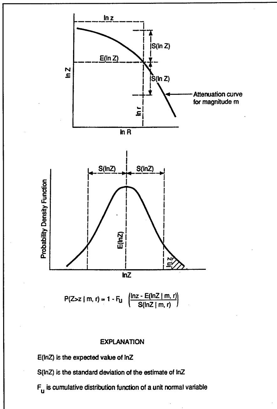
Figure 3-26. Ground motion estimation conditional probability function
