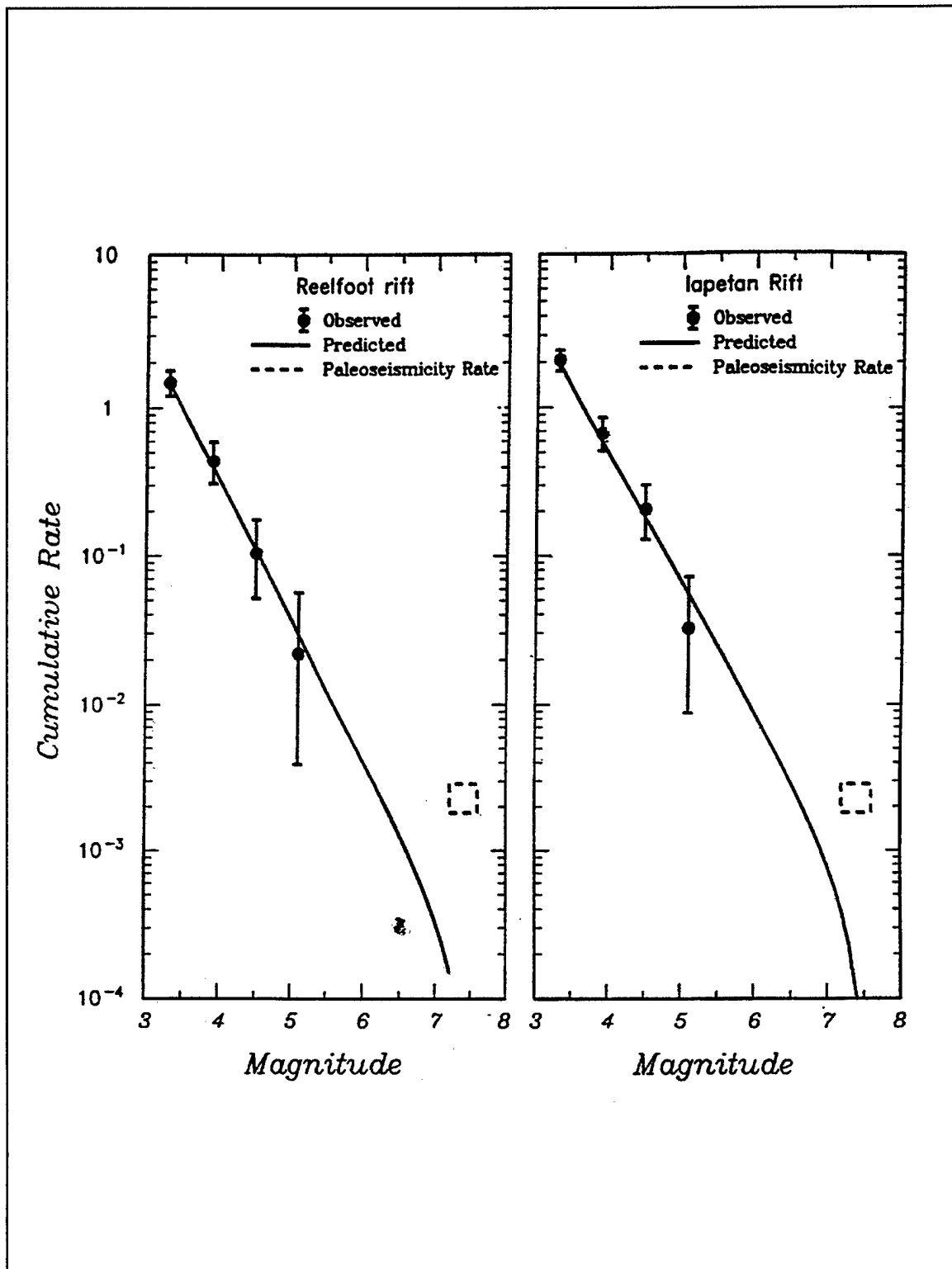
Figure G4-2. Comparison of historical and paleoseismic recurrence estimates for the Reelfoot Rift and Iapetan Rift seismic zone
