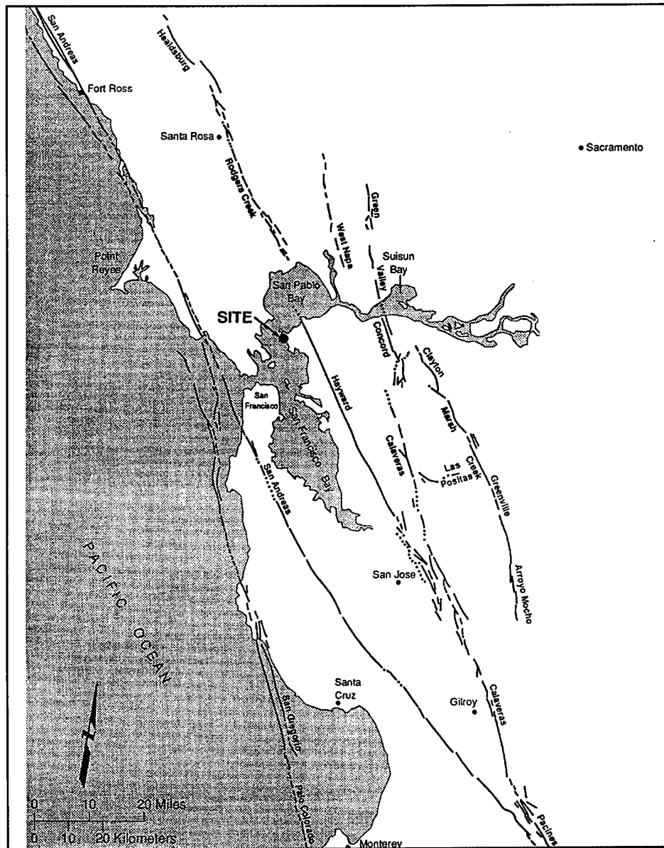
Figure G2-1. Regional active fault map
