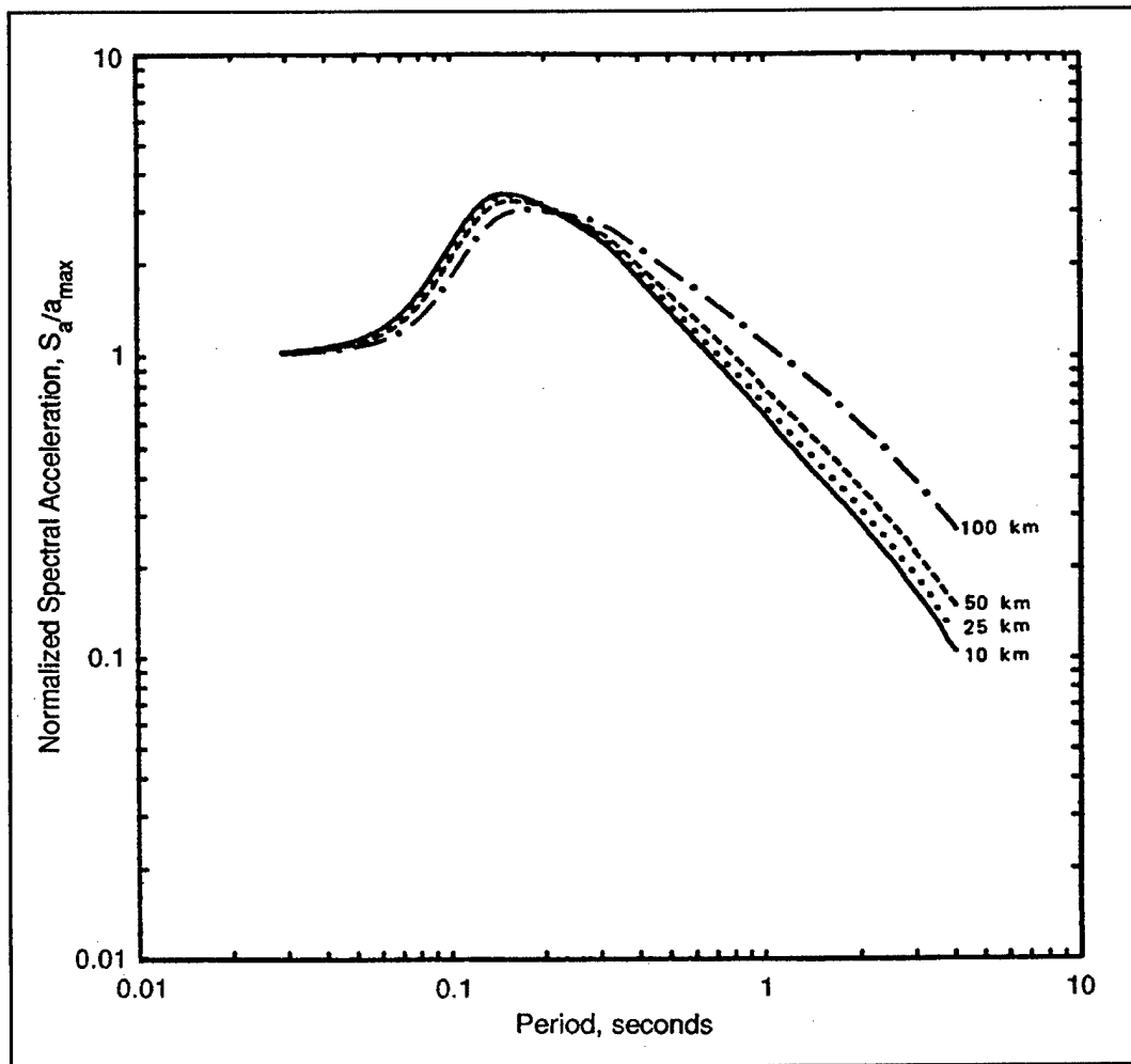
Figure 3-5. Effect of distance on response spectral shapes for a moment magnitude M_w 6.5 earthquake using western North American parameters (Silva and Green 1989, courtesy of Earthquake Engineering Research Institute, Oakland, CA)
