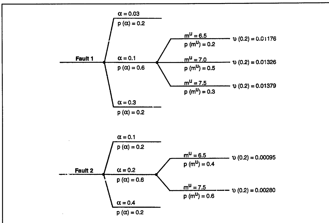
Figure G1-4. Logic trees
