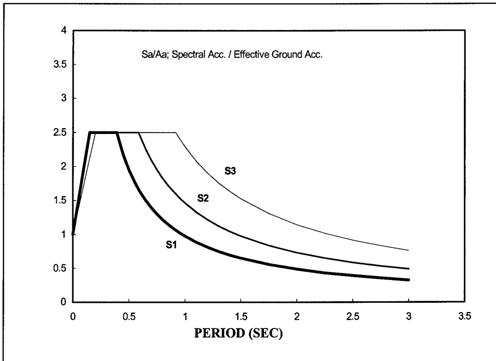
Figure 2-14. Normalized SEAOC's design response spectra
