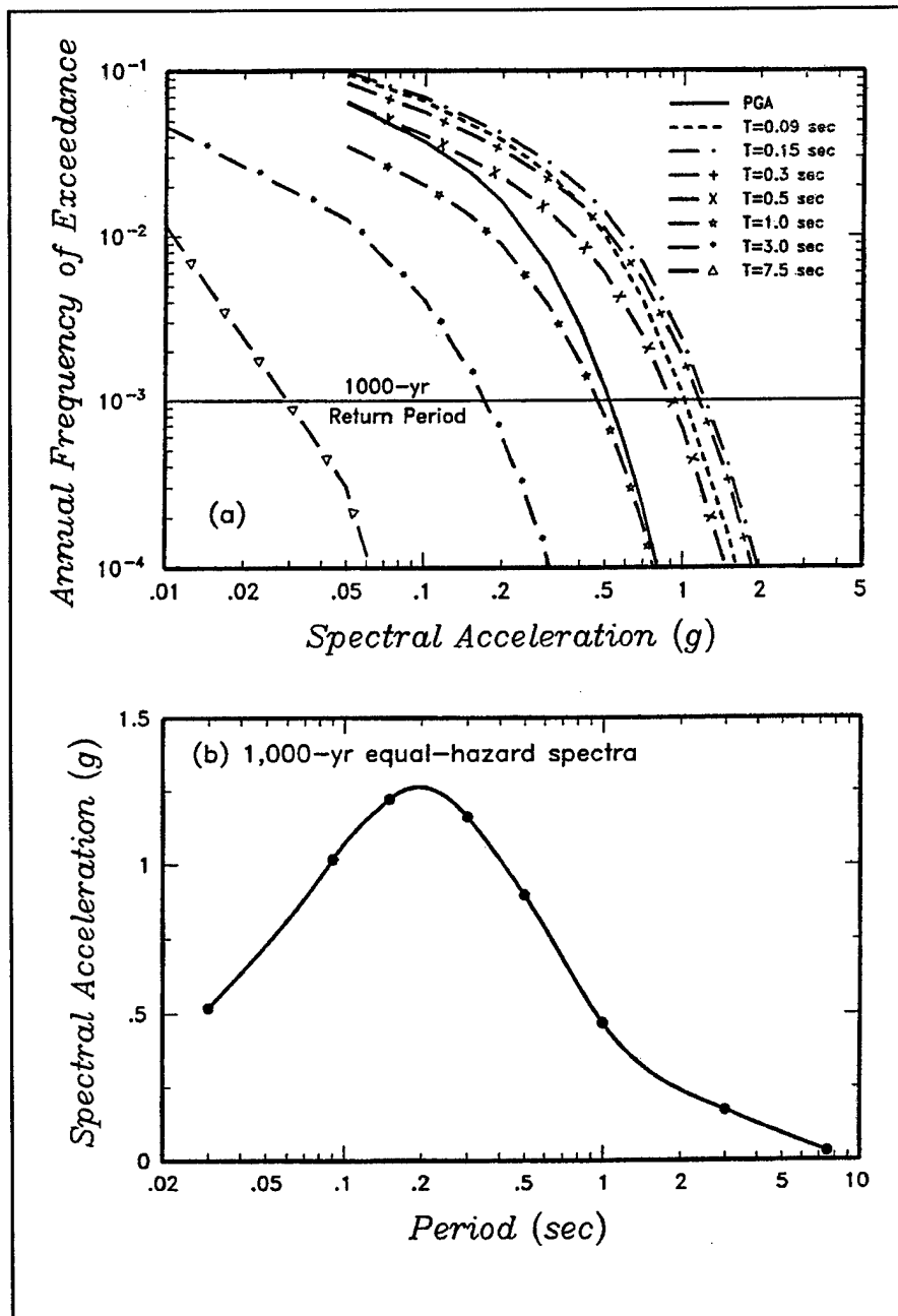
Figure 3-31. Construction of equal-hazard spectra. Top plot (a) shows hazard curves for a range of spectral periods. Bottom plot (b) shows equal hazard spectrum for a period of 1,000 years
