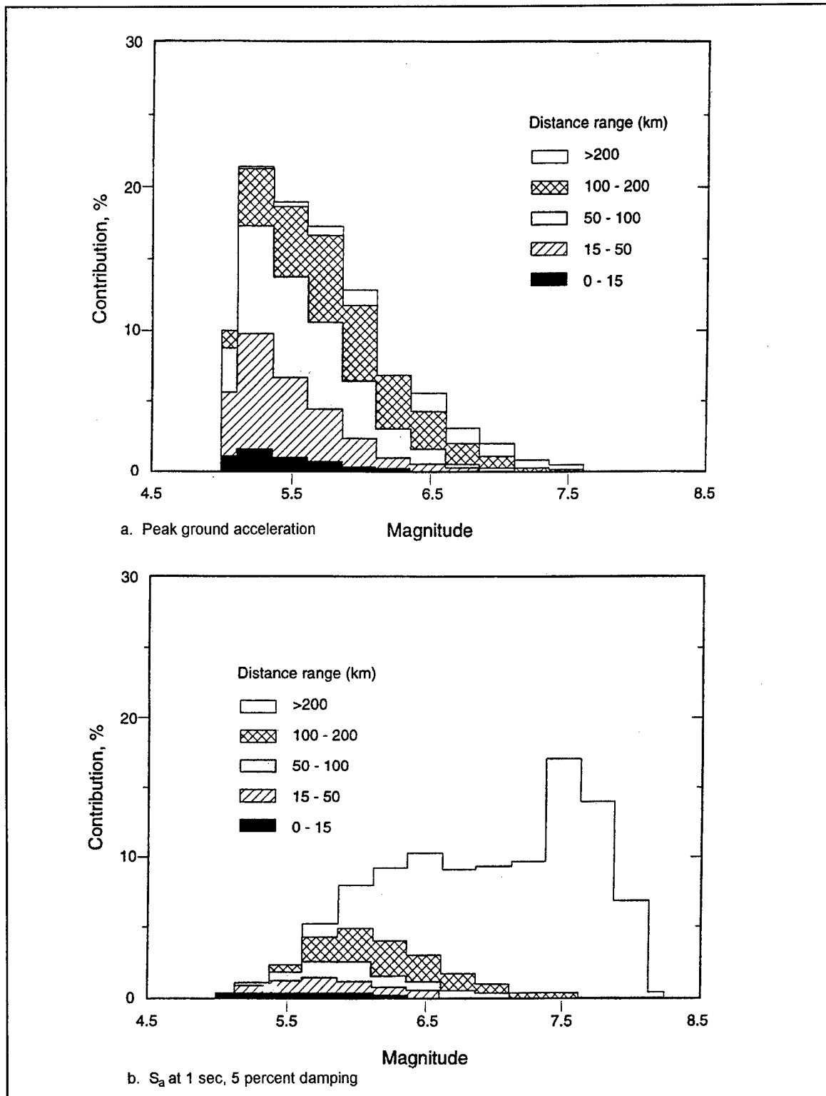
Figure G5-5. Magnitude and distance contributions to hazard for peak ground acceleration and response spectral acceleration at 1.0 sec for 1000-year return period
