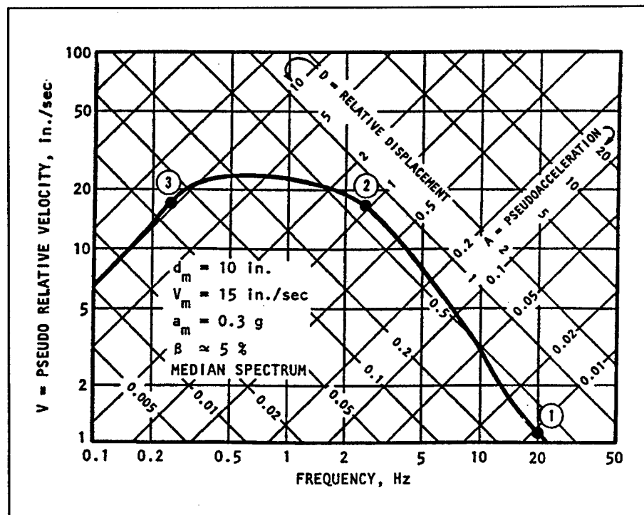
Figure B-1. Typical response spectrum for earthquake motions (Newmark and Hall 1982)
