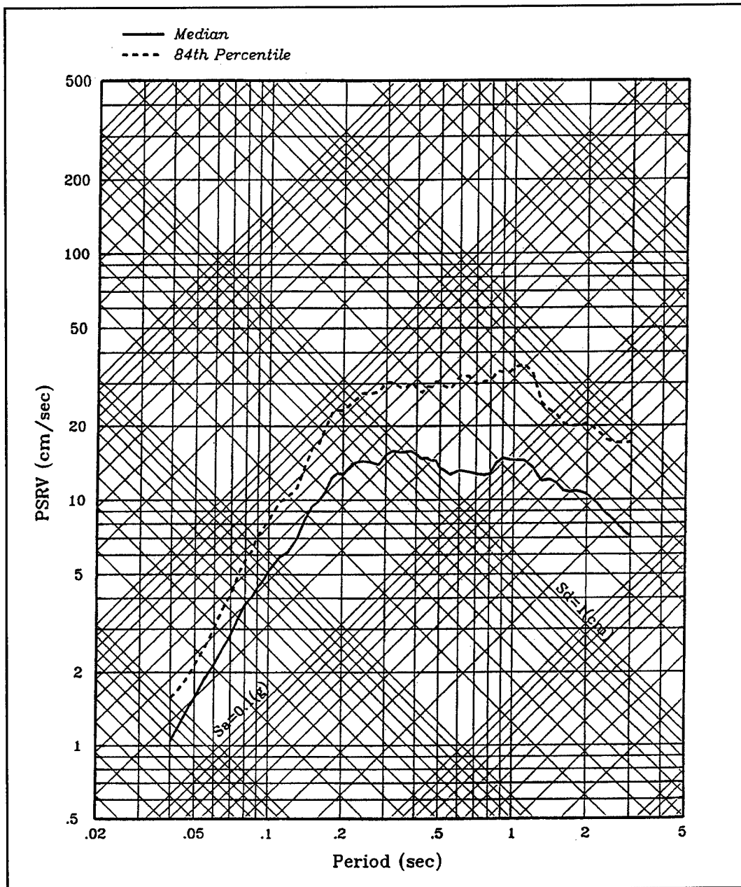
Figure C-1. Median and 84th percentile spectra (5 percent damping) for a magnitude 6.5 strike-slip earthquake at 18 km based on statistics of adjusted rock recordings
