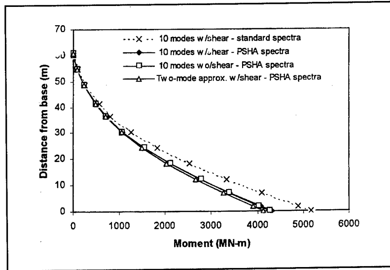
Figure H-12. Maximum moments due to 1000-year San Francisco Bay area response spectra applied along x-axis (transverse direction)
