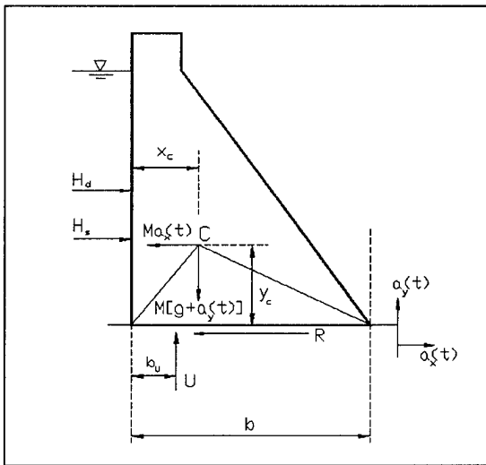
Figure 2-13. Rigid gravity dam on horizontal ground
