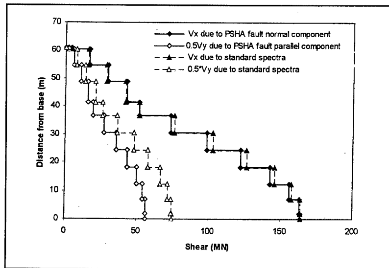
Figure H-15. Combination of shear forces V_x and 0.5V_y for site-specific and standard ground motions
