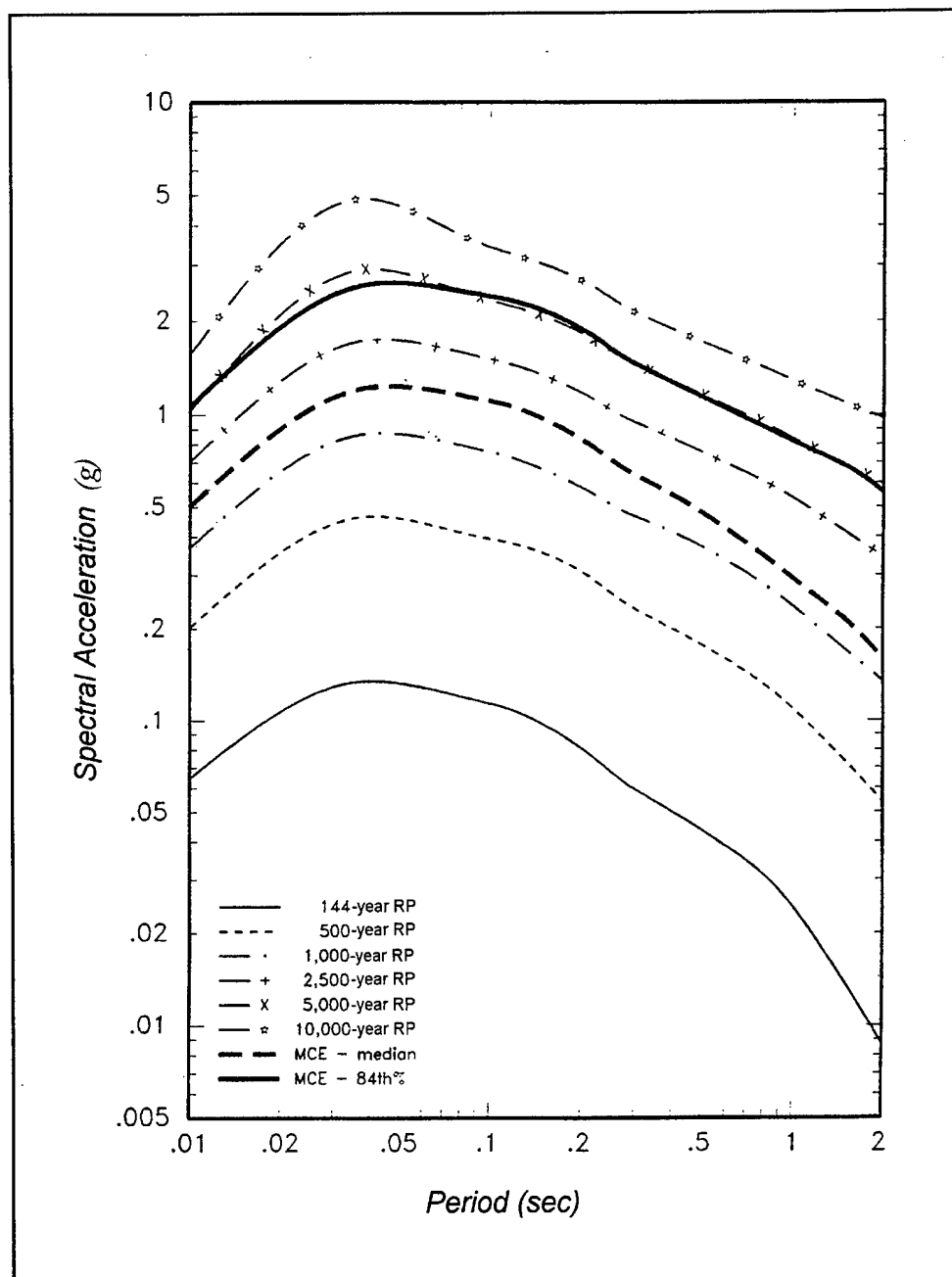
Figure G4-9. Comparison of equal-hazard and deterministic response spectra (5 percent damping)
