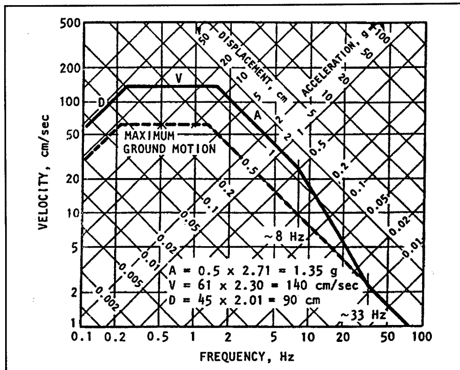
Figure B-2. Elastic design spectrum horizontal motion (0.5 g maximum acceleration, 5 percent damping, one sigma cumulative probability) (Newmark and Hall 1982)
