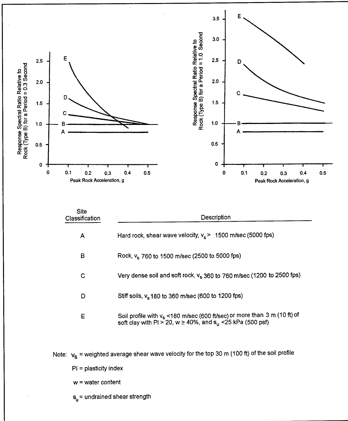
Figure 3-9. Response spectral ratios relative to rock for different site classifications and ground motion levels (BSSC 1994)
