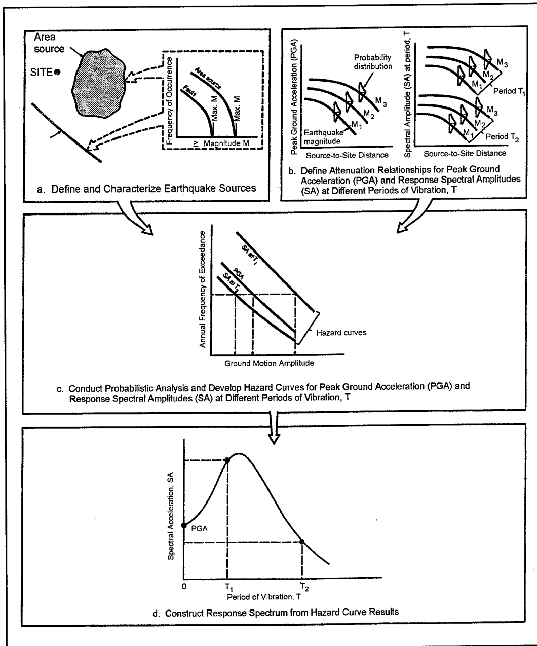
Figure 3-22. Development of equal-hazard response spectrum from probabilistic seismic hazard analysis for response spectral values
