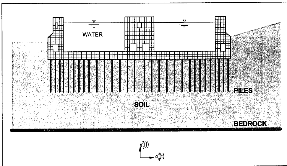
Figure 2-5. 2-D model of W-frame lock
