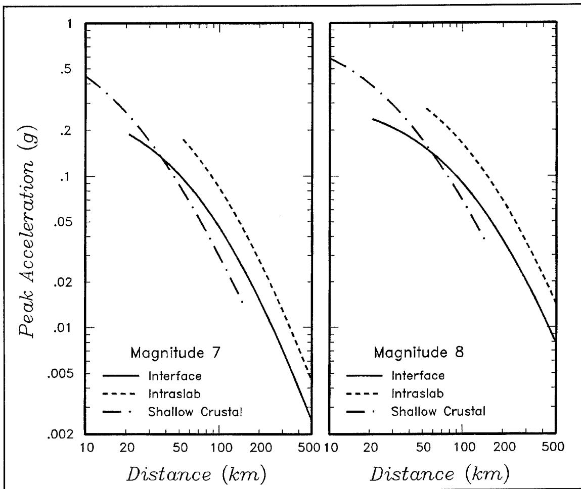
Figure 3-14. Comparison of median peak accelerations on rock from subduction zone earthquakes with peak accelerations from WUS shallow crustal earthquakes
