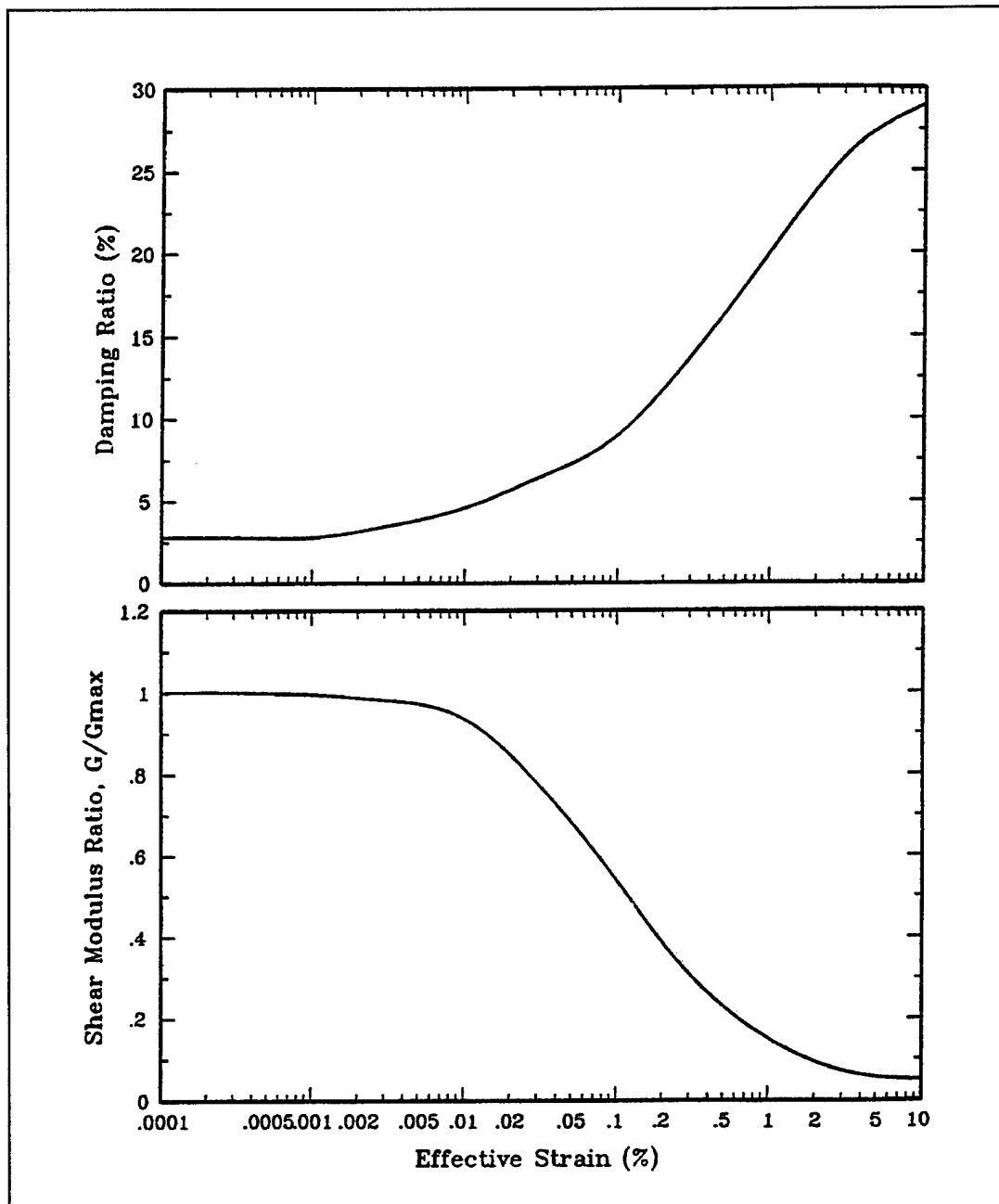
Figure E-2. Variation of shear modulus and damping ratio with shear strain for clays (Seed and Sun 1989, courtesy of Earthquake Engineering Research Center, University of California at Berkeley)
