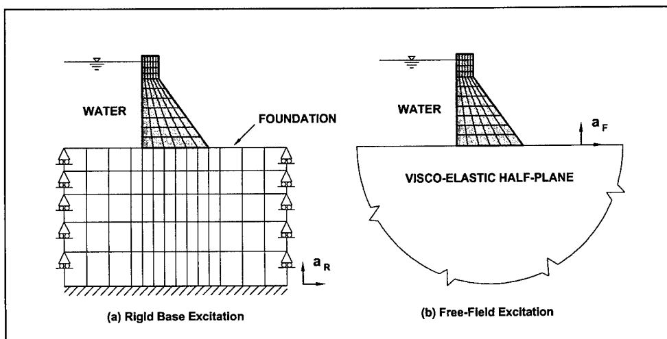
Figure 2-6. Earthquake excitation for rock or firm soil sites
