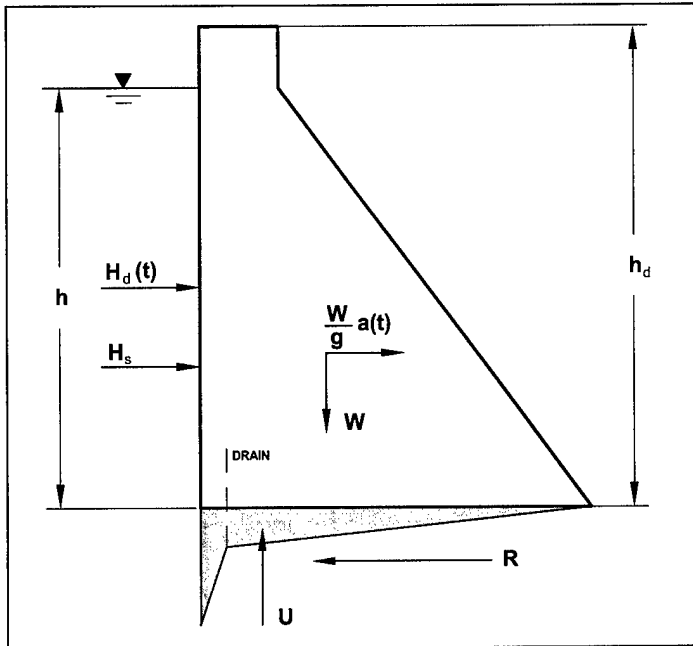
Figure 2-10. Forces acting on gravity dam monolith
