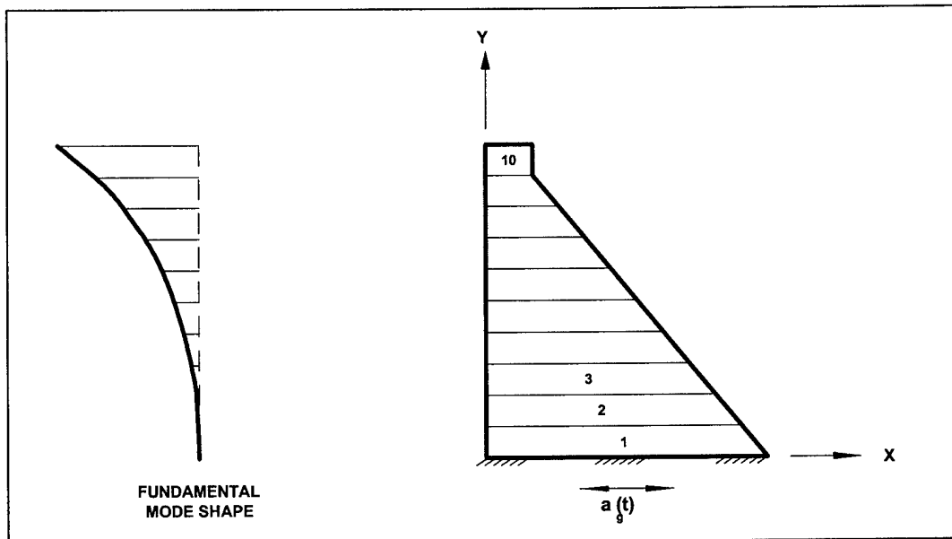
Figure 2-4. Simplified model of gravity dam monolith (Fenves and Chopra (1986), courtesy of Earthquake Engineering Research Center, University of California at Berkeley)
