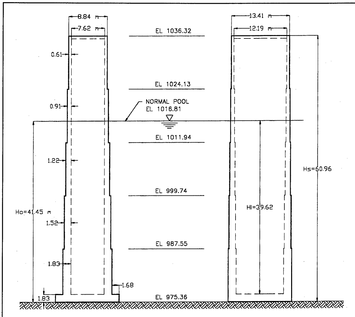
Figure H-1. Geometry of example intake tower
