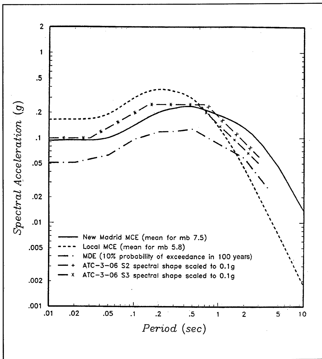
Figure G3-14. MDE spectra (5 percent damping)
