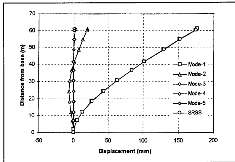
Figure H-10. Modal and SRSS displacements due to 1000-year San Francisco Bay area response spectra motion applied along x-axis (transverse direction)
