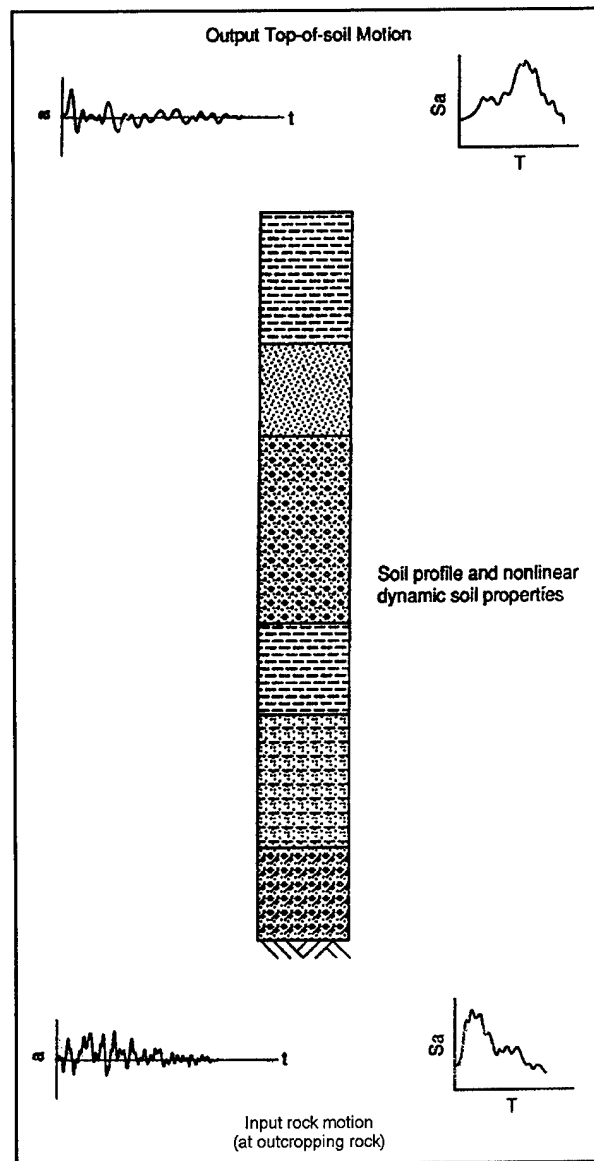
Figure 3-19. Schematic of one-dimensional site response analysis
