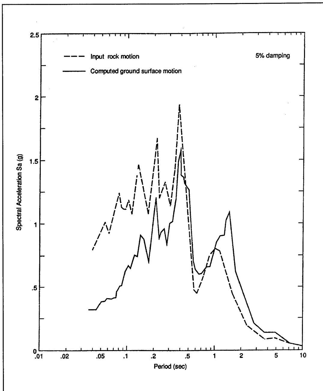
Figure E-4. Comparison of response spectra of computed ground surface motion with input rock motion, average soil properties
