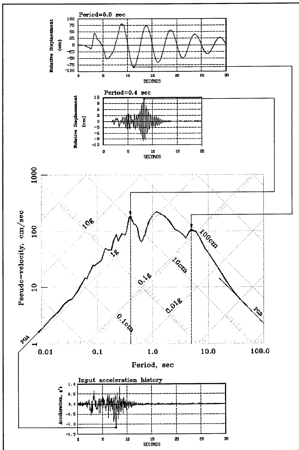
Figure 2-2. Construction of tripartite elastic design response spectrum
