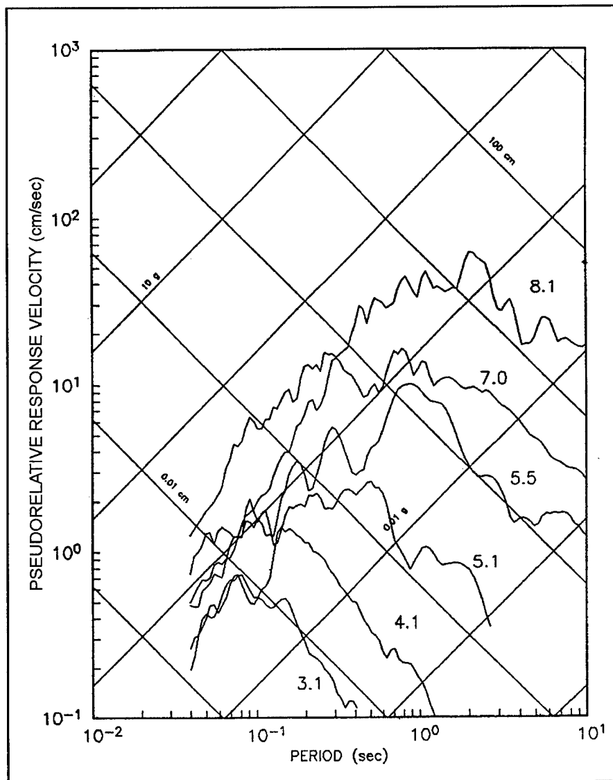
Figure 3-2. Response spectra (5 percent damped, pseudo-relative velocity) corresponding to the acceleration traces in Figure 3-1 (Anderson and Quaes (1988), courtesy of Earthquake Engineering Research Institute, Oakland, CA)
