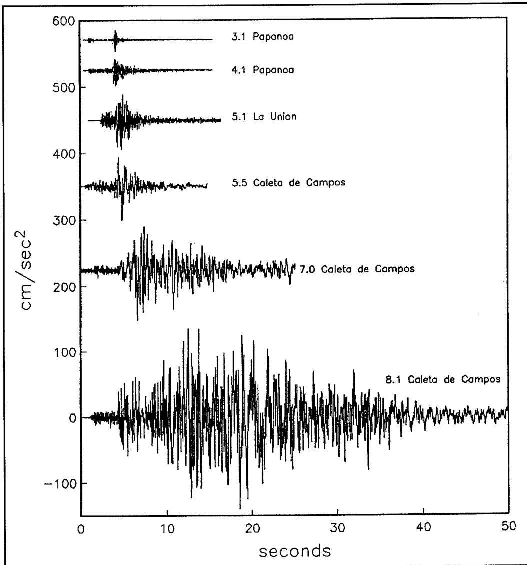
Figure 3-1. An example of accelerograms recorded in 1985 and 1986 on the Guerrero accelerograph array (Anderson and Quaa (1988), courtesy of Earthquake Engineering Research Institute, Oakland, CA)
