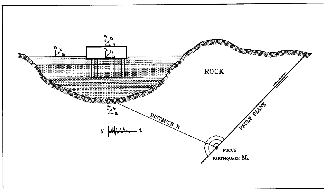
Figure 2-1. Factors affecting seismic input motion for a structure founded on soil-pile foundation
