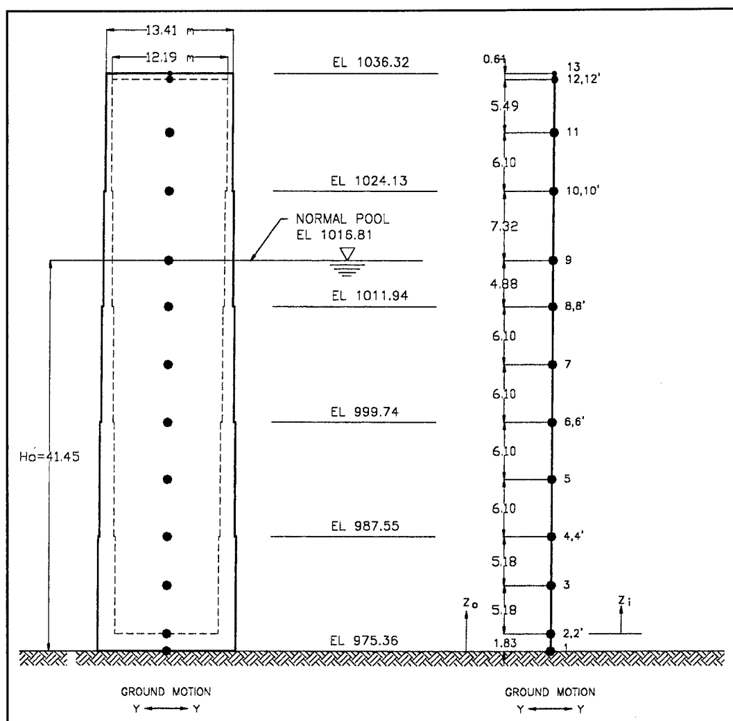
Figure H-4. Structural idealization for excitation along longitudinal axis (y-axis)
