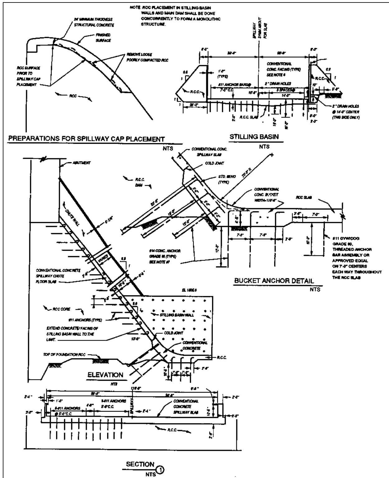
Figure 1-16. Conventional concrete overlays may be required to resist erosion
