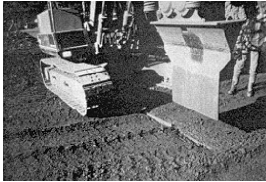
Figure 1-7. Contraction joint installation
