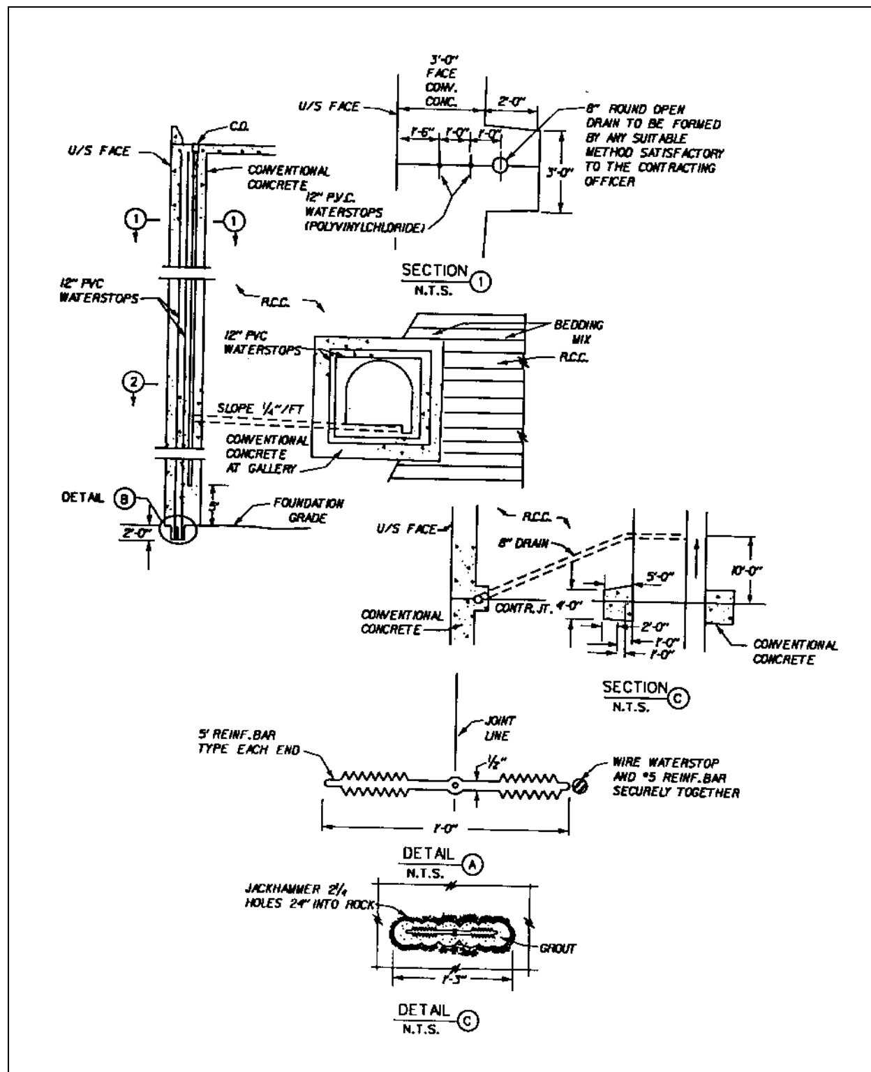
Figure 1-21. Waterstop details
