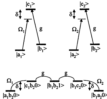
Figure 1: Illustration of the excitation scheme needed to implement a cavity dark state. As shown in the top diagram, the classical laser beams are detuned, while the cavity is kept on resonance. The bottom diagram shows the same situation in the rotating wave frame. The state |b_1b_20\rangle (not shown) is still the trivial dark state.
