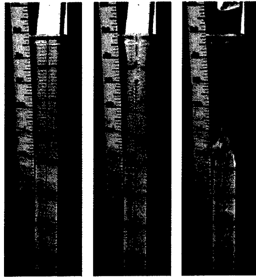
Figure 23. High-speed video of an AbsorbEdge static line during rupture.
