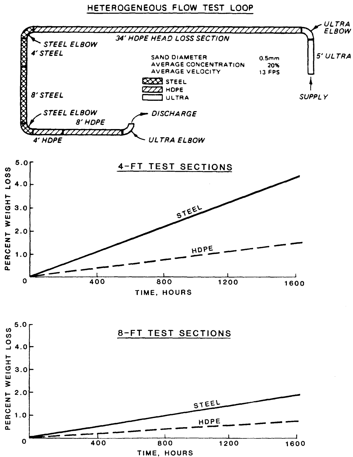
FIG. 2.--Heterogeneous test loop and data
