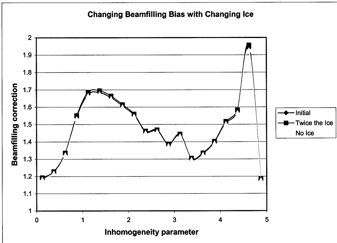
Figure 5.1: Beam-filling correction to inhomogeneity parameter relationship, with changing ice content
