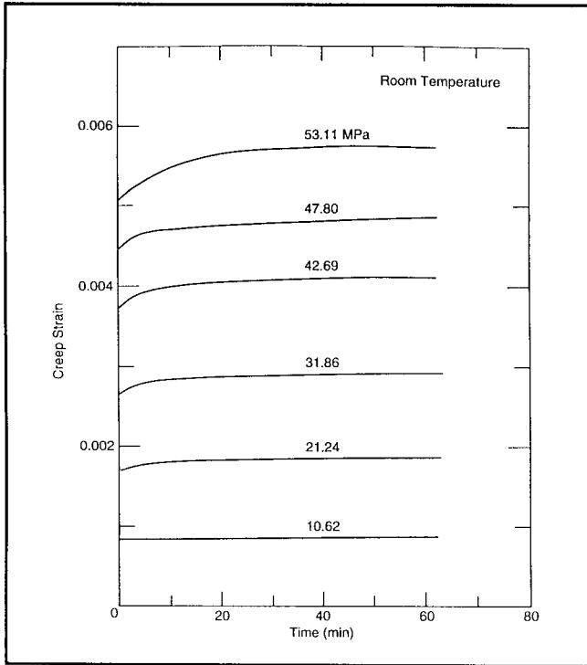
Figure 6-4. Tensile creep curves for a vinyl-ester/glass composite at various stress levels (after Mallick 1988)
