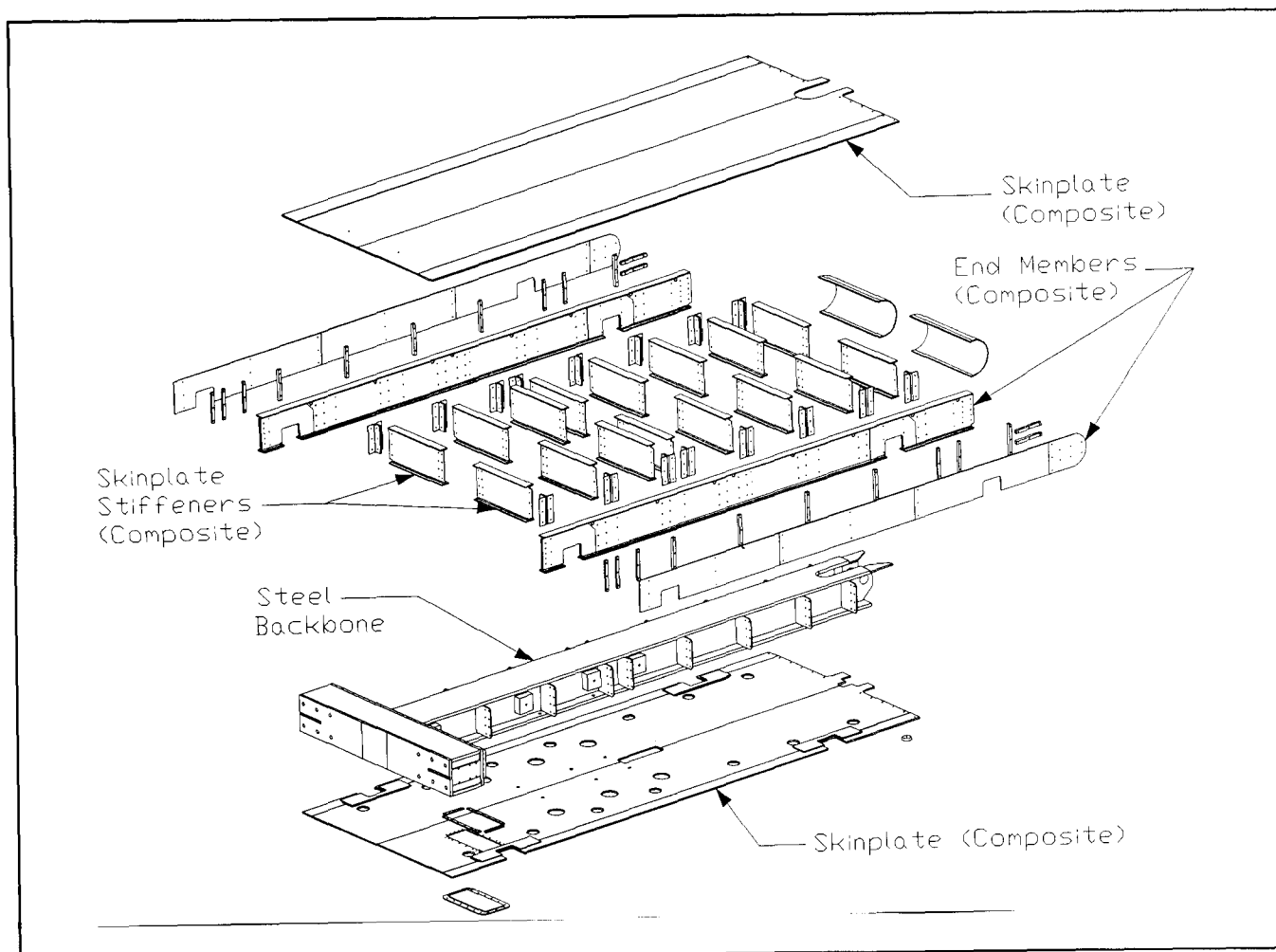
Figure B-4. Exploded view of composite wicket gate
