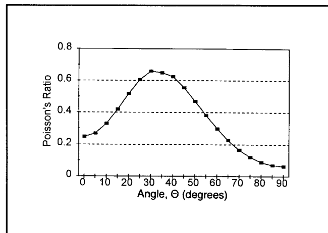
Figure 5-3. Poisson's ratio as a function of fiber orientation for a typical glass/polyester composite. Lay-up is of the form [\Theta(1)/-\Theta(2)/\Theta(1)] , where \Theta is the angle in degrees
