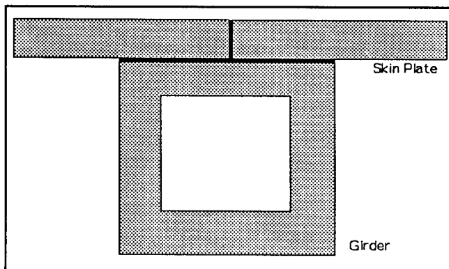
Figure 7-7. Example of an adhesive joint that is a partially lapped joint and a partially strapped joint
