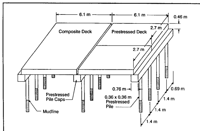
Figure B-5. Diagram of demonstration pier construction
