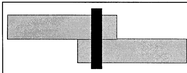
Figure 7-1. Single lap bolted joint
