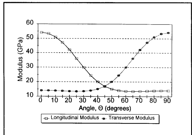
Figure 5-1. Modulus as a function of fiber orientation for a typical glass/polyester composite. Lay-up is of the form [\Theta(1)/-\Theta(2)/\Theta(1)] , where \Theta is the angle in degrees
