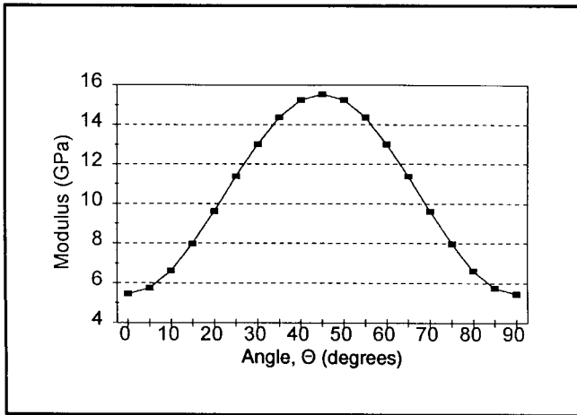
Figure 5-2. Shear modulus as a function of fiber orientation for a typical glass/polyester composite. Lay-up is of the form [\Theta(1)/-\Theta(2)/\Theta(1)] , where \Theta is the angle in degrees
