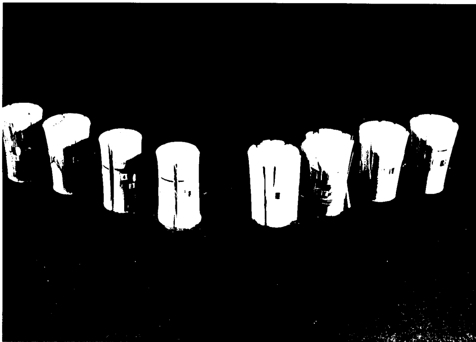
Figure 6-2. Composites failures are more violent at low temperature (right) than at room temperature (left)
