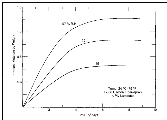
Figure 6-1. Water absorption behavior of polymer composites
