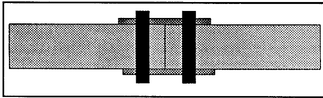
Figure 7-3. Strapped bolted joint
