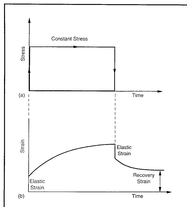
Figure 6-3. Schematic of the creep behavior of polymer composites
