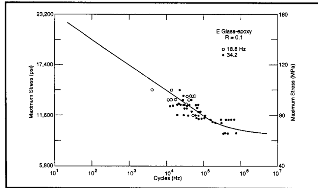
Figure 6-5. A typical fatigue behavior of an E-glass-epoxy composite
