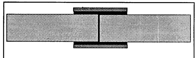
Figure 7-6. Strapped bonded joint
