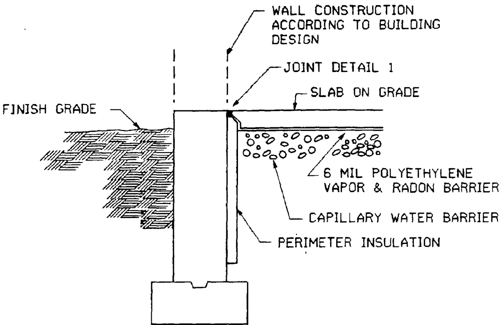
DETAIL 13 EXTERIOR WALL WITH PERIMETER INSULATION
