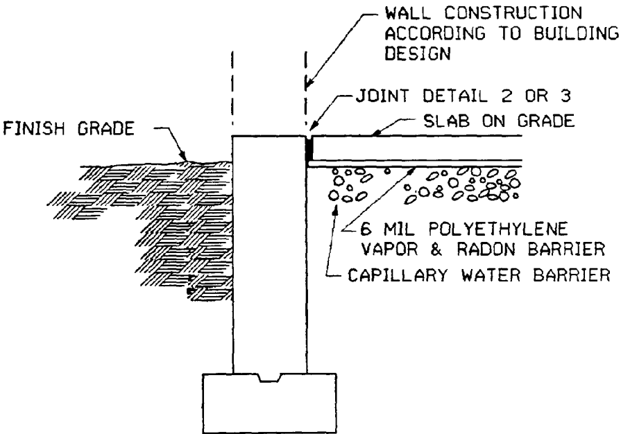
DETAIL 14 EXTERIOR WALL UNINSULATED
