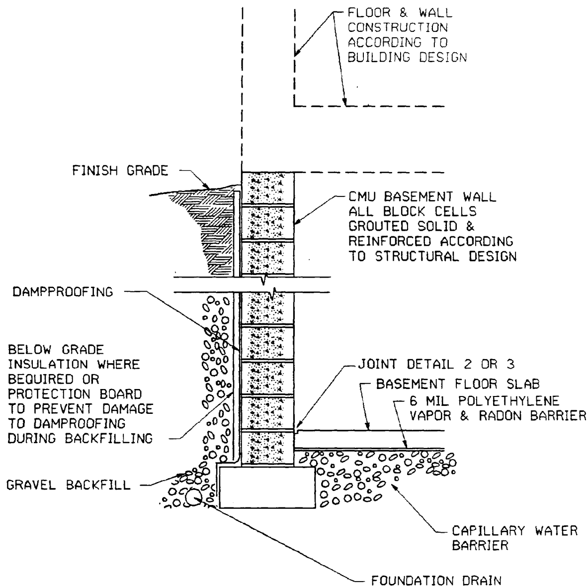
DETAIL 19 EXTERIOR BASEMENT WALL CODE A
