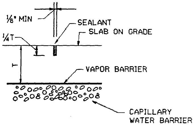
JOINT DETAIL CONTROL JOINT CODE A 5
