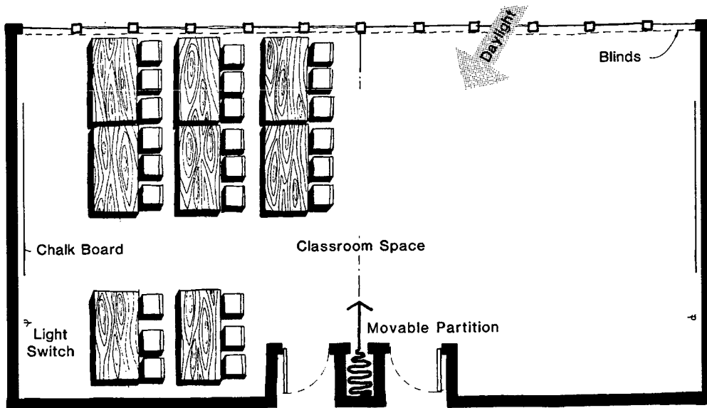
Figure 3-21. Classroom plan.
