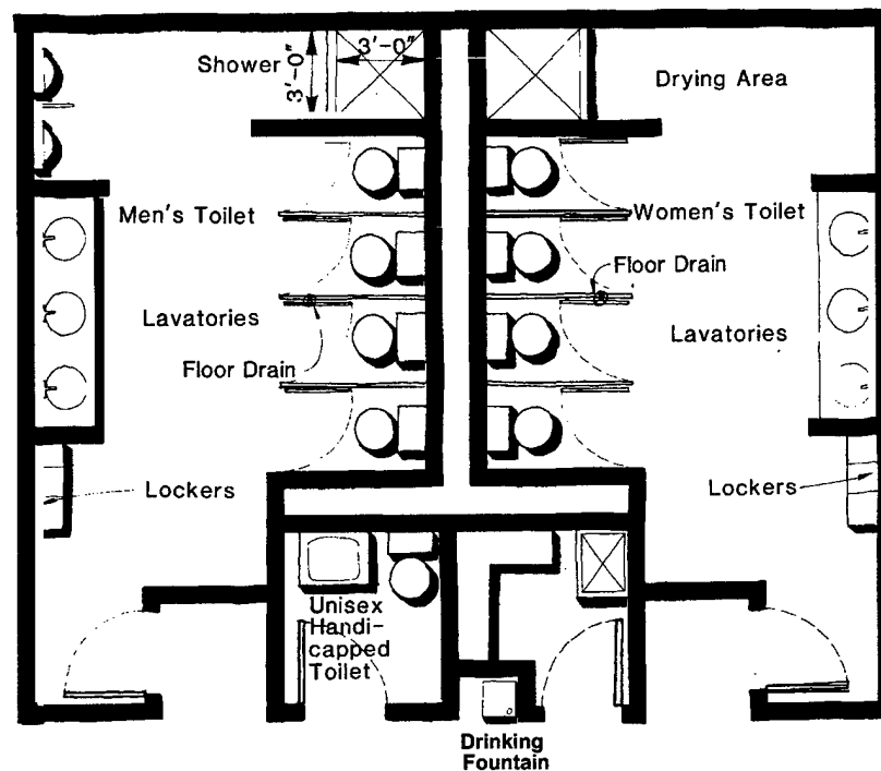
Figure 3-32. Toilet plan.
