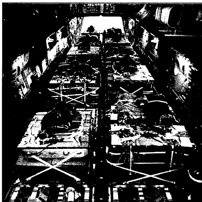
Figure 3. C-17 Dual-Row Airdrop
