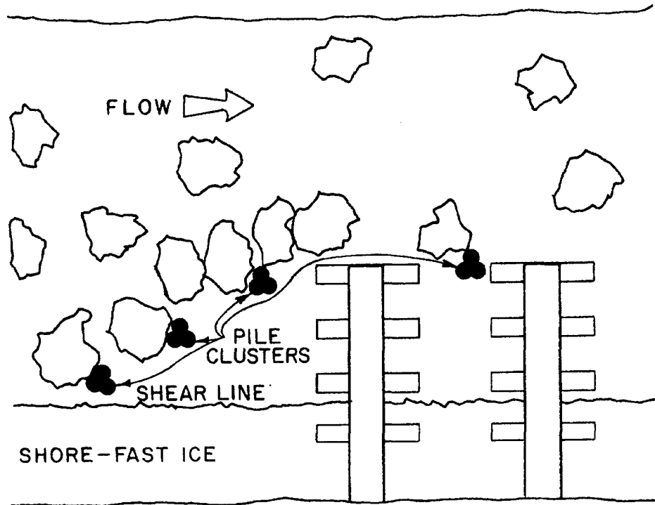
Figure 3-16. Controlling ice flows with pile clusters.
