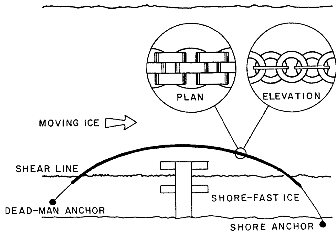
Figure 3-17. Controlling ice flows with a floating tire breakwater.
