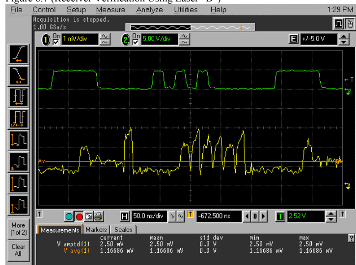
Figure 6.7 (Receiver Verification Using Laser “B”)
