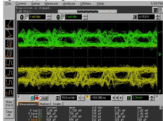
Figure B.1 (Q 1 Eye Diagram)
