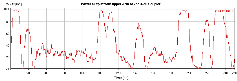
Figure 5.11c (-198 Degree Phase Shift)
