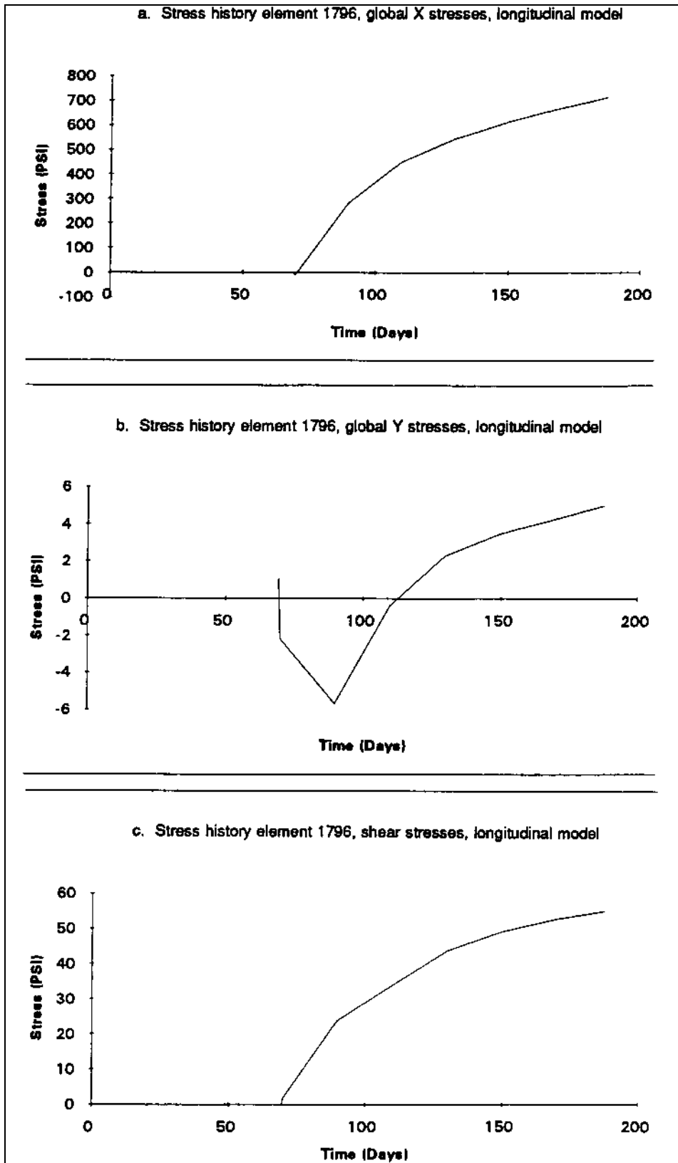
Figure A-40. Stress Histories for Element 1796
