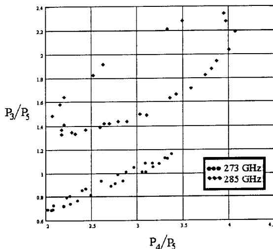
Fig. 6. Measured "calibration ellipses" for the sampled-line reflectometer at 273 GHz ( \bullet ) and 285 GHz ( \diamond ). A least-squares fit to the data provides the calibration coefficients for the six-port to four-port conversion.
