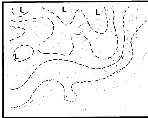
Figure 4-65. 500-mb Analysis, 0000Z/25 June 1979. 12 hours after Figure 4-63. Weak thermal trough where thunderstorm line developed.
