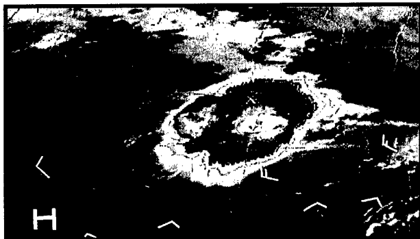
Figure 4-20. Infrared (MB), 1500Z 22 June 1981. Developed MCC over the central Great Plains.
