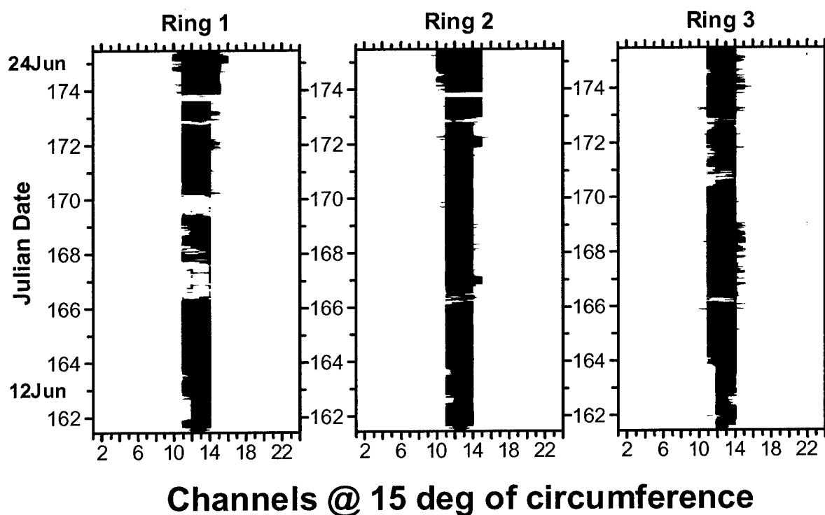
Figure 3. Mine burial measured at a shallow water (7 m) site 150 m off the beach at Panama City, Florida. The shaded areas represent a blocked passage of light between pairs of optical sensors that are located every 15^\circ on three rings around the instrumented mine (see Figure 2).
