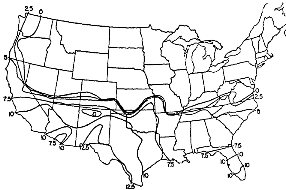
Figure H-11. Average pan evaporation, in centimetres, for the continental United States for the month of November based on data taken from 1931 to 1960
