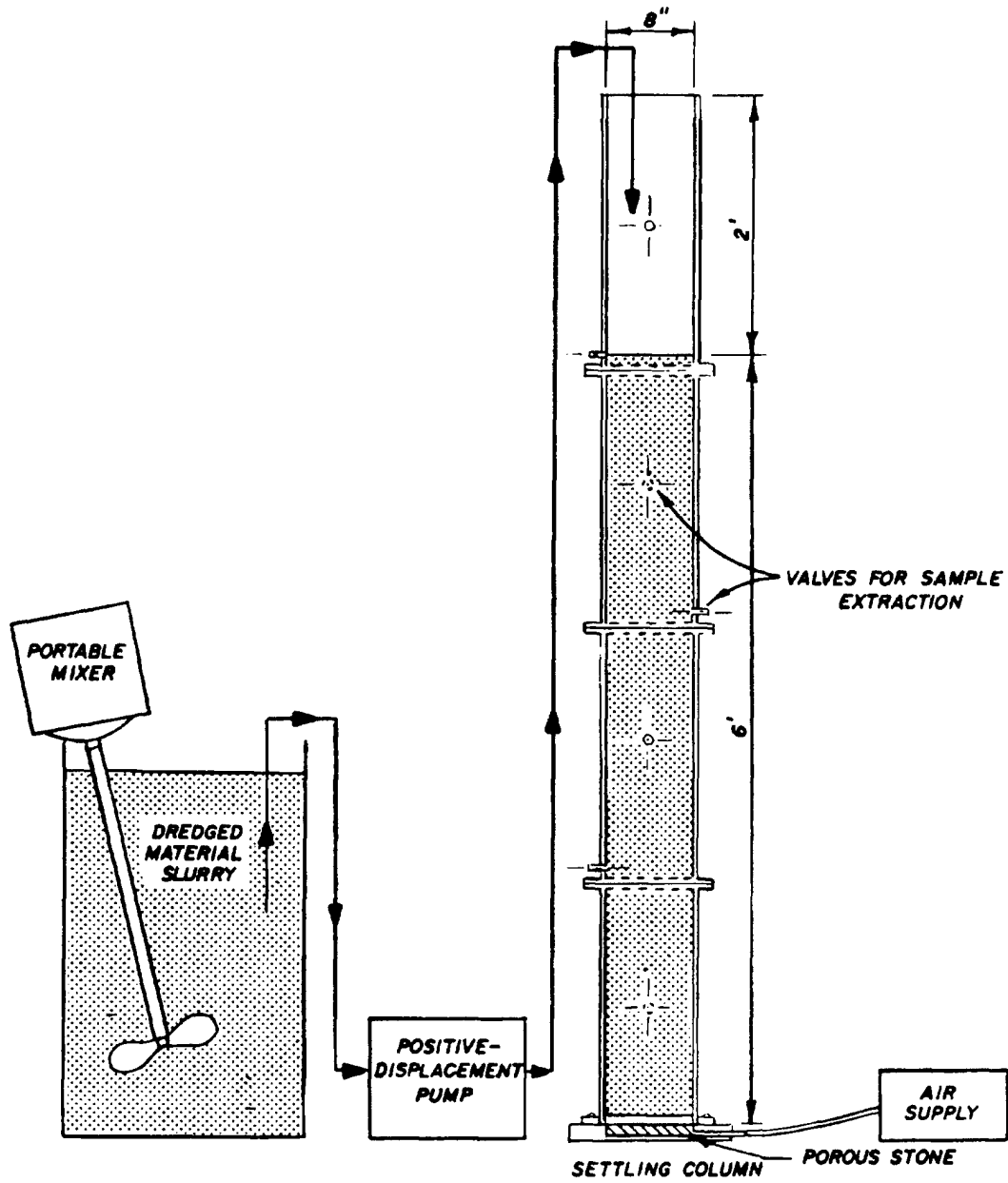
Figure 3-3. Schematic of apparatus for settling tests
