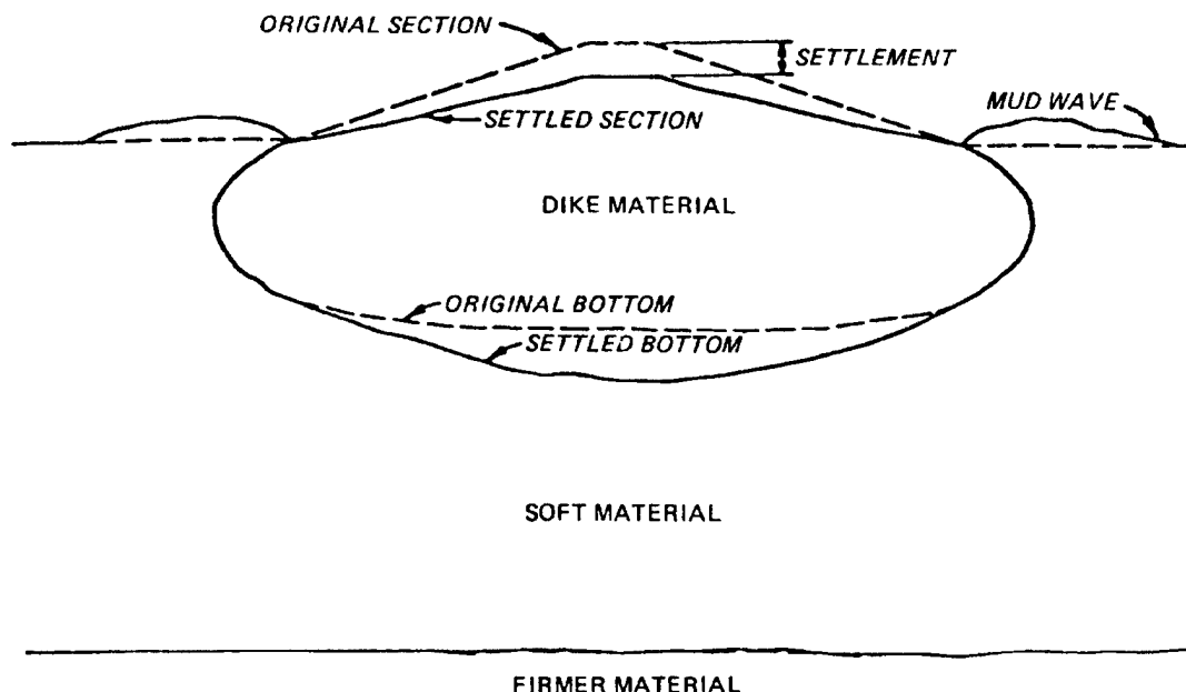
Figure 6-9. Example of excessive uniform settlement
