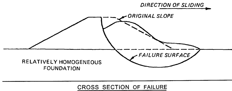
Figure 6-4. Rotational failure in both dike and foundation
