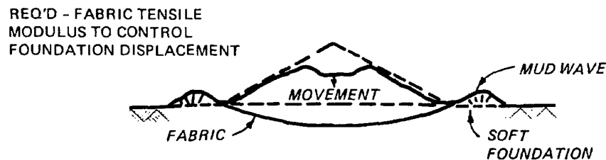
C. POTENTIAL EMBANKMENT FAILURE FROM EXCESSIVE DISPLACEMENT
