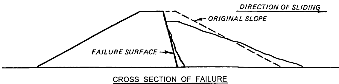
Figure 6-3. Translatory failure in dike
