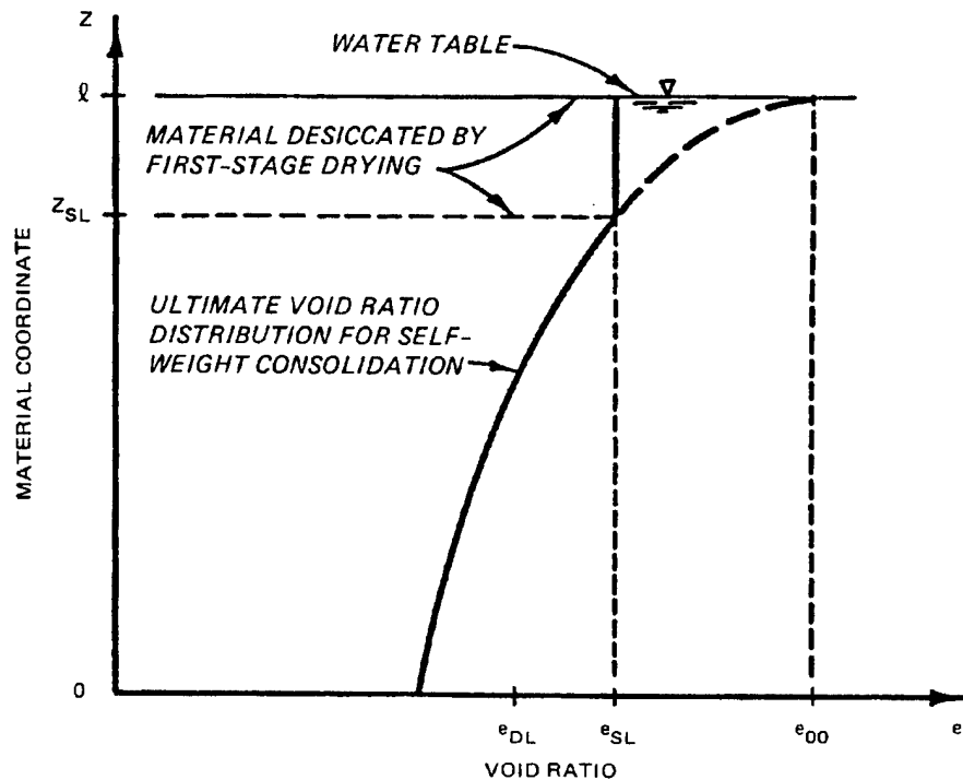
Figure F-7. Maximum depth of material desiccated by first-stage drying
