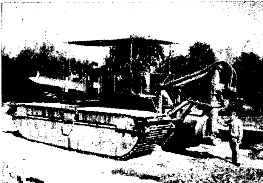
Figure 5-16. Track-mounted rotary trencher used in mosquito control activities
