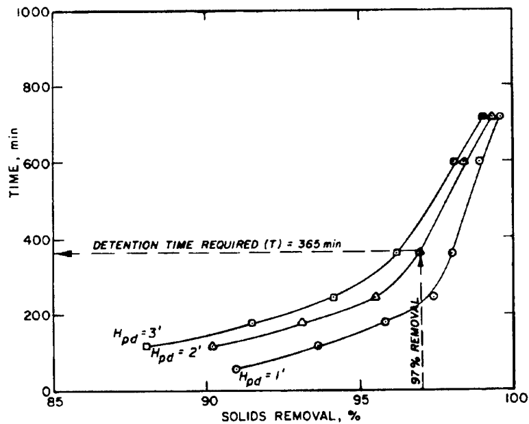
Figure C-3. Solids removal versus time
