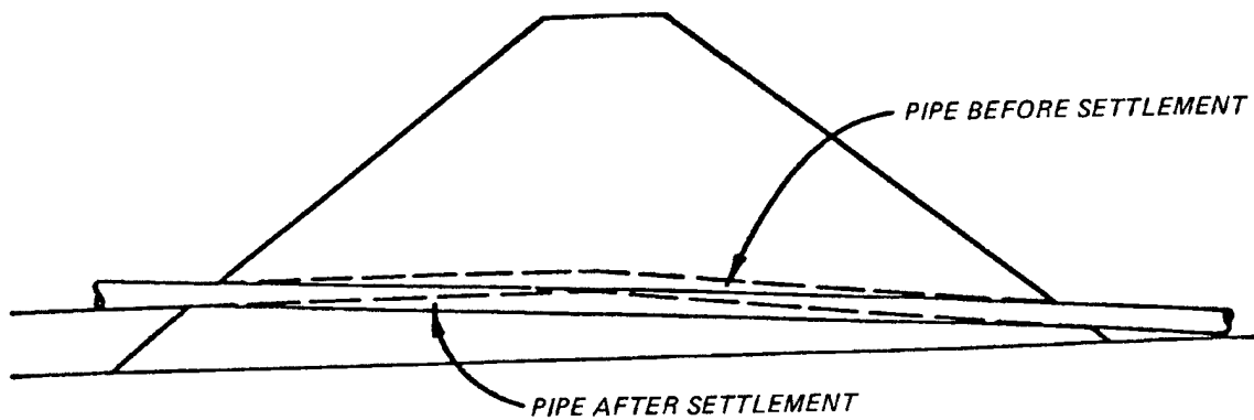
Figure 6-16. Cambered and raised pipe beneath dike
