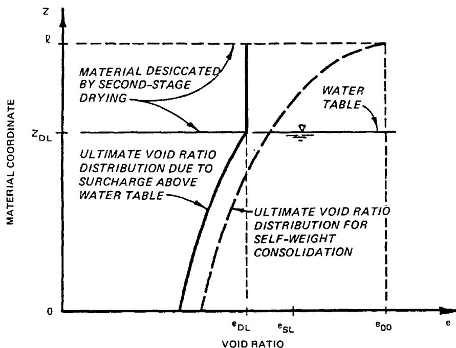
Figure F-8. Maximum depth of material desiccated by second-stage drying
