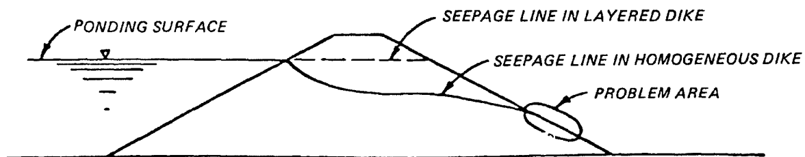
Figure 6-7. Seepage lines through dike
