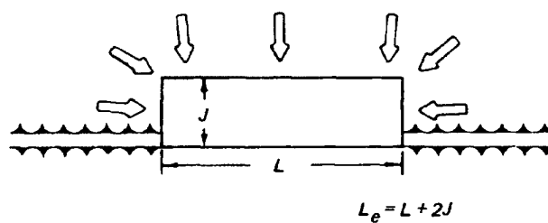
b. JUTTING RECTANGULAR WEIR
