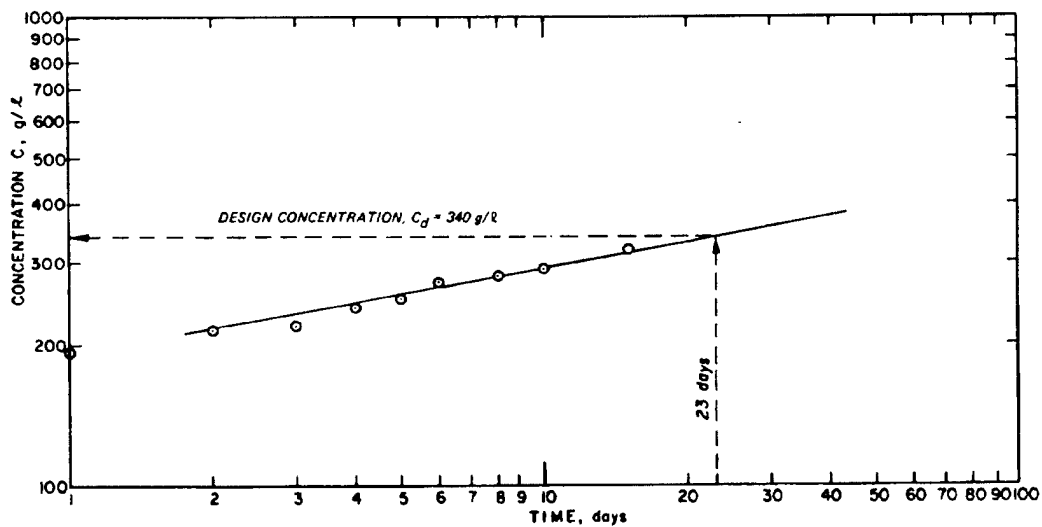
Figure C-4. Concentration of settled solids versus time
