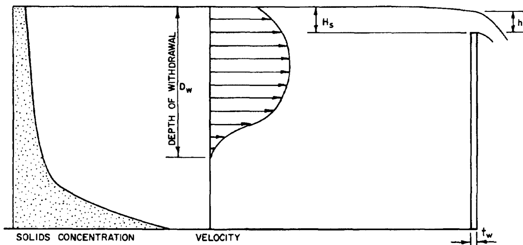
Figure 4-6. Conceptual illustration of withdrawal depth and velocity profile
