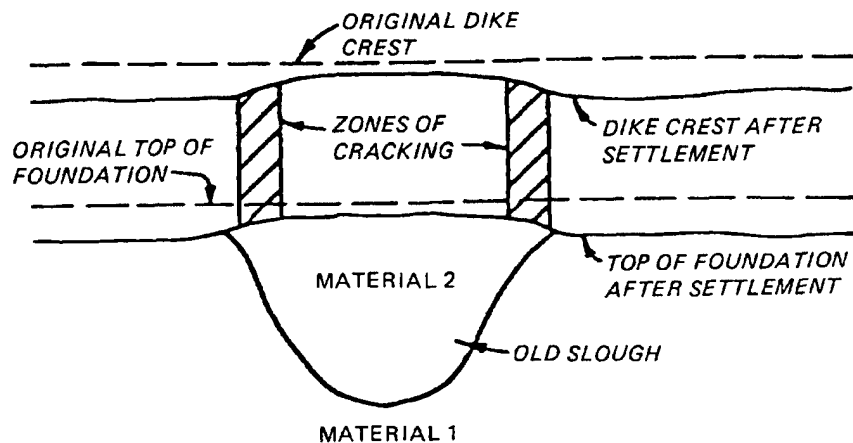
b. COMPRESSIBILITY OF MATERIAL 2 << MATERIAL 1
