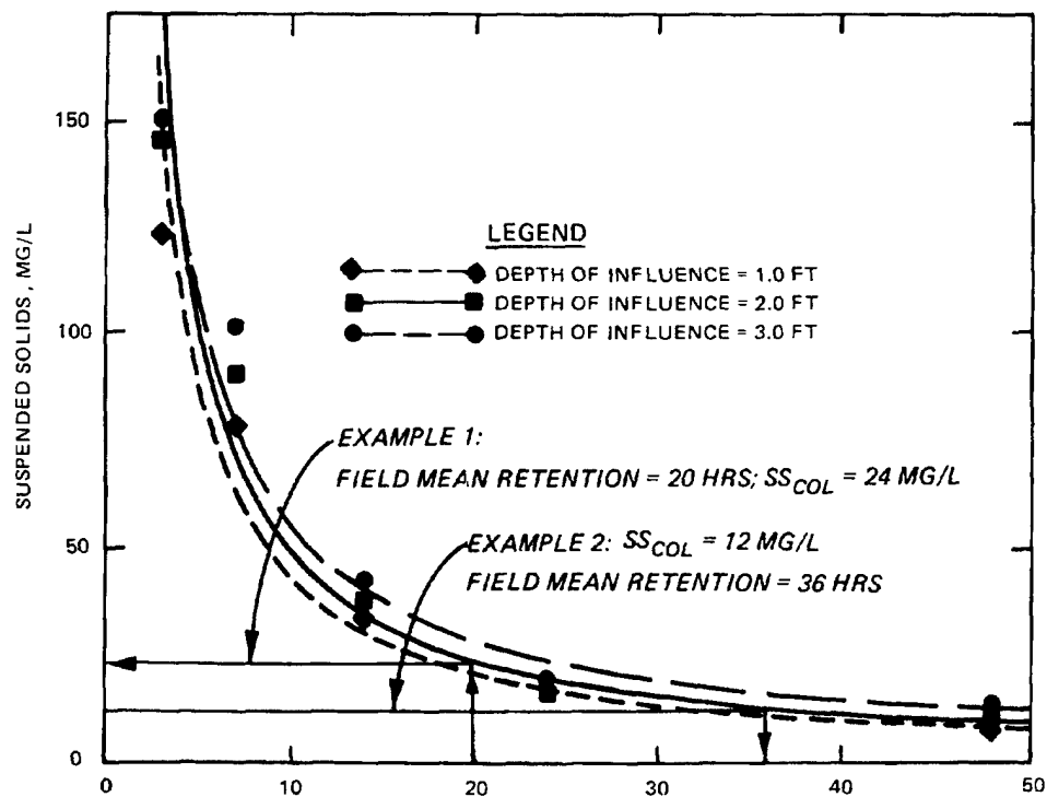
Figure C-6. Plot of supernatant suspended solids concentration versus time from column settling tests
