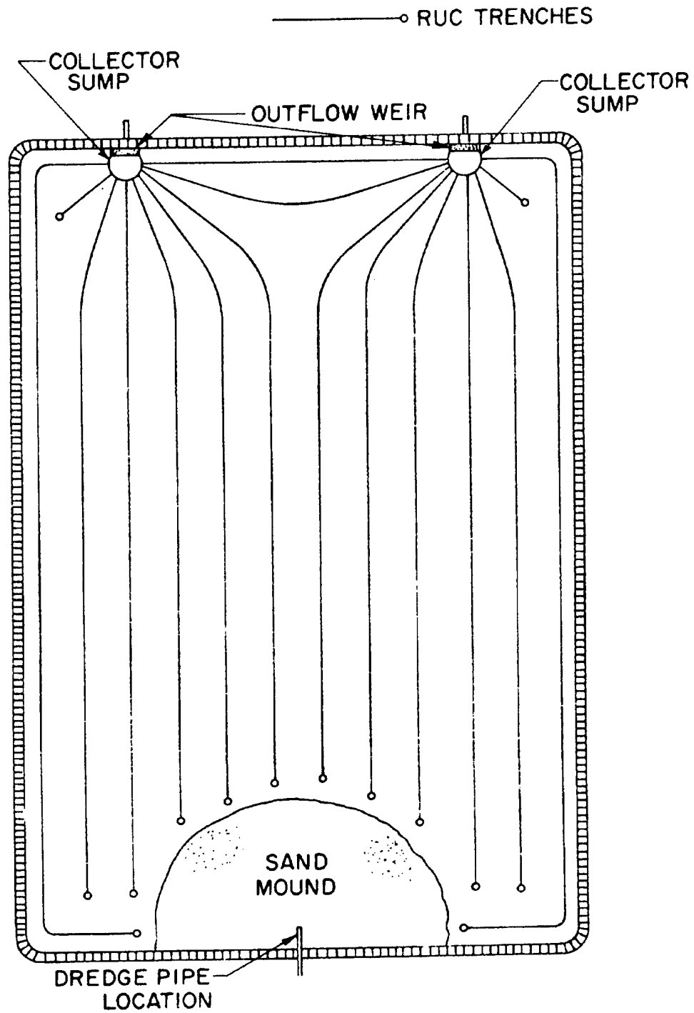
Figure 5-23. Combination radial-parallel trenching scheme
