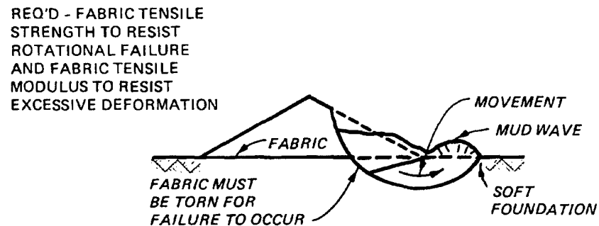
B. POTENTIAL EMBANKMENT ROTATIONAL SLOPE/FOUNDATION FAILURE
