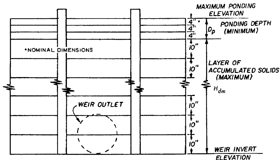
Figure 4-9. Recommended boarding configuration
