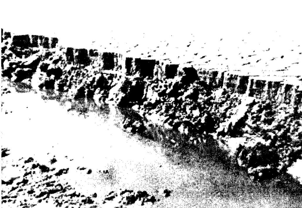
Figure 5-12. Desiccation crust adjacent to perimeter 3- to 5-foot-deep drainage trench
