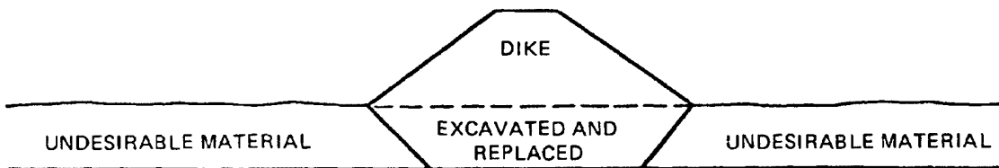
c. SECTION FORMED BY EXCAVATION AND REPLACEMENT
