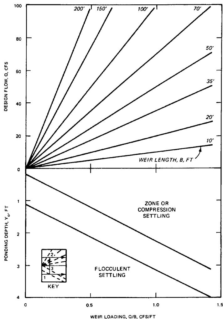
Figure 4-7. Weir design nomograph
