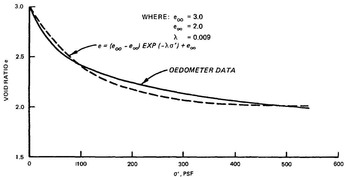
b. FOUNDATION
