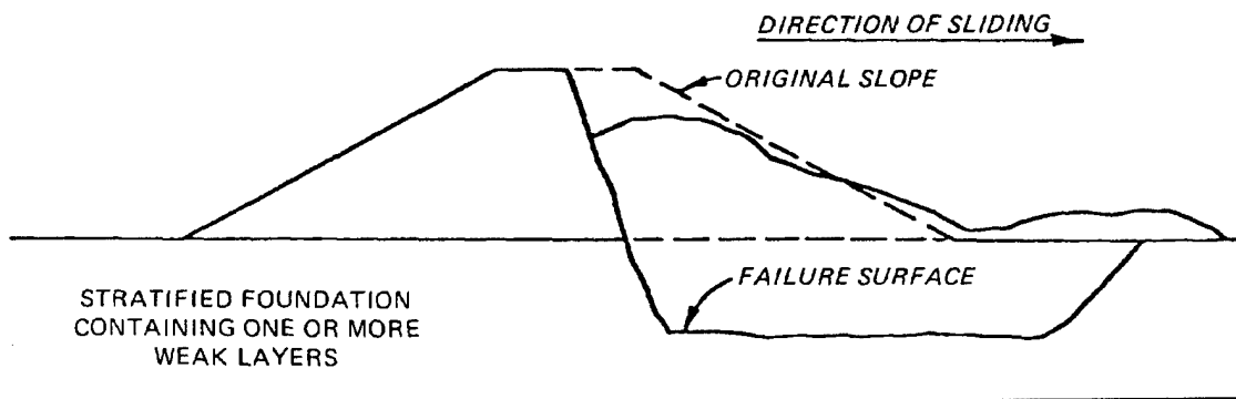
Figure 6-5. Translatory failure in both dike and foundation
