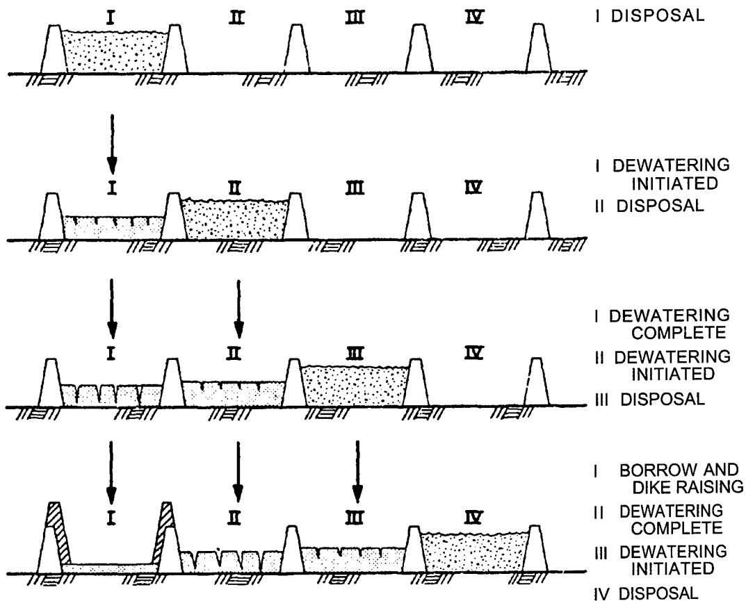
Figure 7-2. Conceptual illustration of sequential dewatering operations
