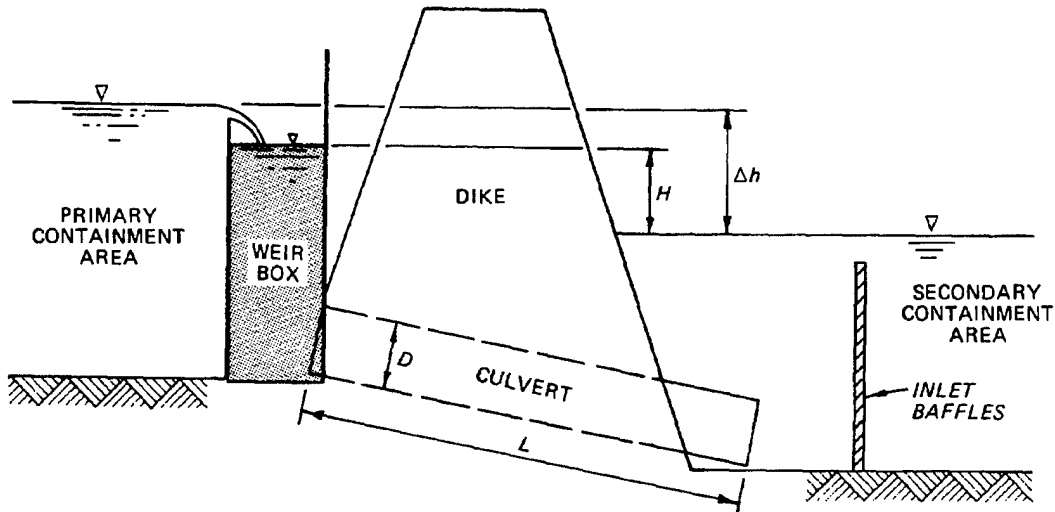
Figure G-5. Example weir mixing system
