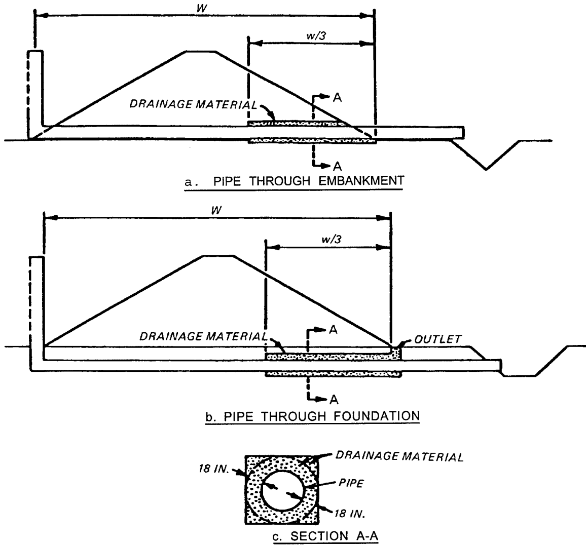
Figure 6-17. Annular drainage material around outlet one third of pipe
