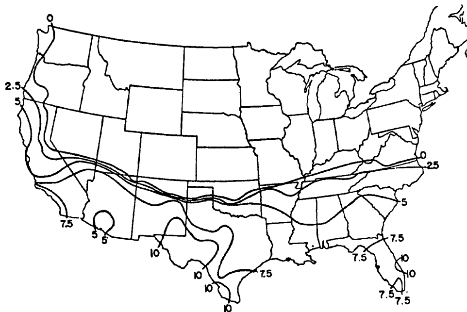
Figure H-1. Average pan evaporation, in centimetres, for the continental United States for the month of January based on data taken from 1931 to 1960
