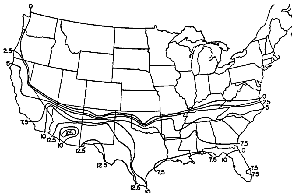
Figure H-2. Average pan evaporation, in centimetres, for the continental United States for the month of February based on data taken from 1931 to 1960
