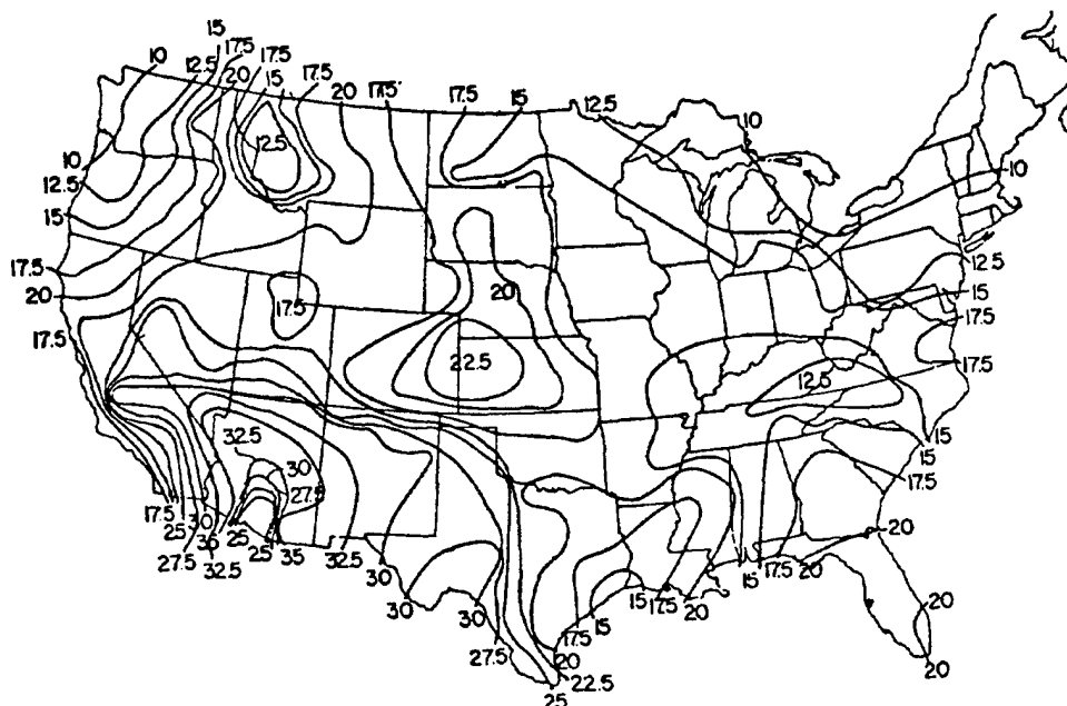
Figure H-5. Average pan evaporation, in centimetres, for the continental United States for the month of May based on data taken from 1931 to 1960
