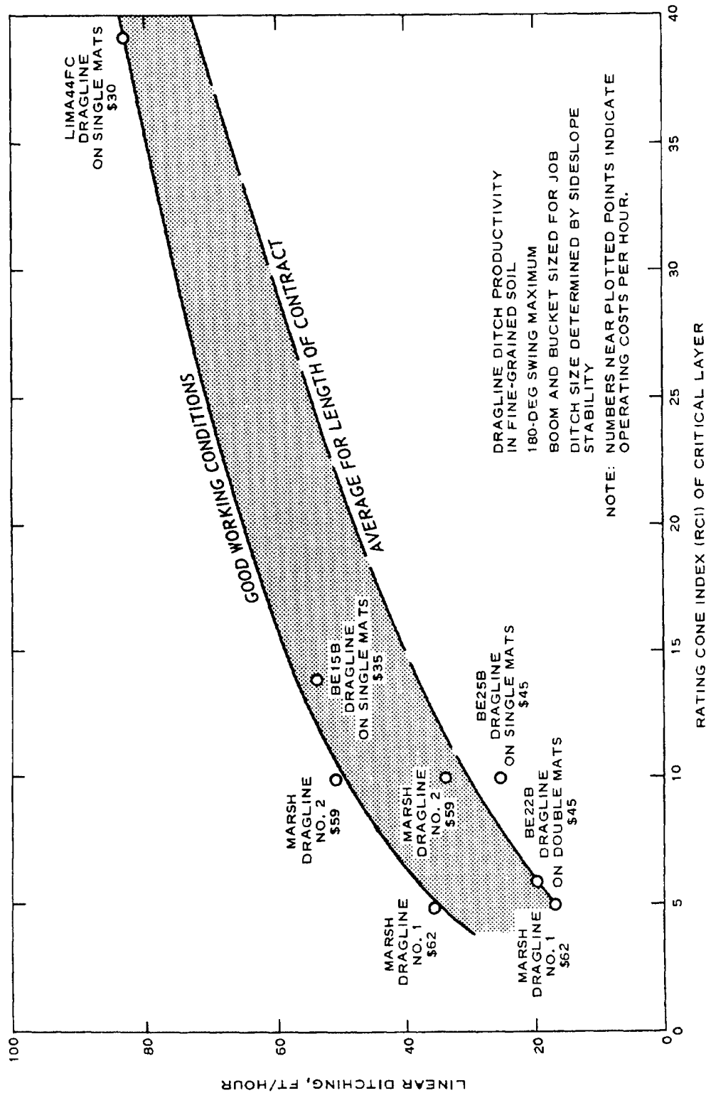
Figure I-2. Relationship between RCI of confined disposal area surface crust and linear trenching rate obtainable by dragline equipment
