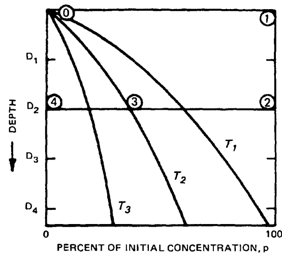
Figure 3-5. Conceptual concentration profile diagram
