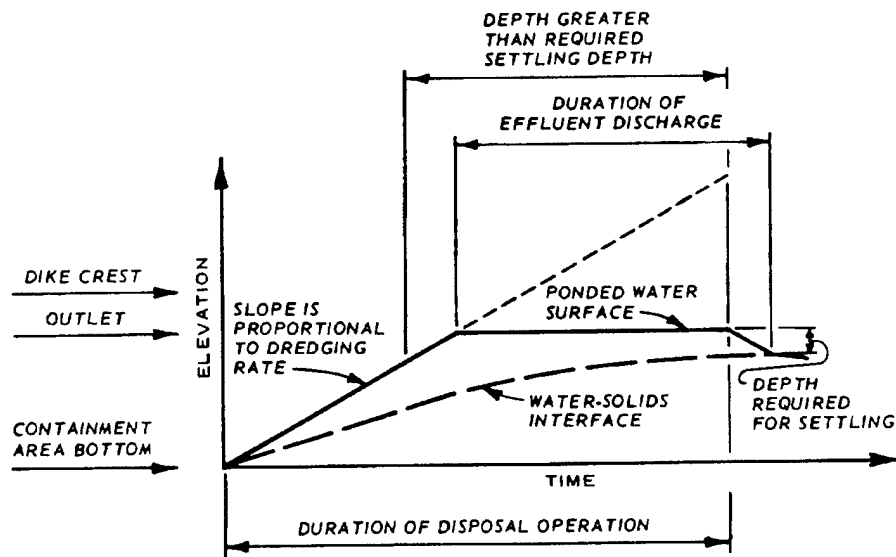
Figure 7-4. Surface water management
