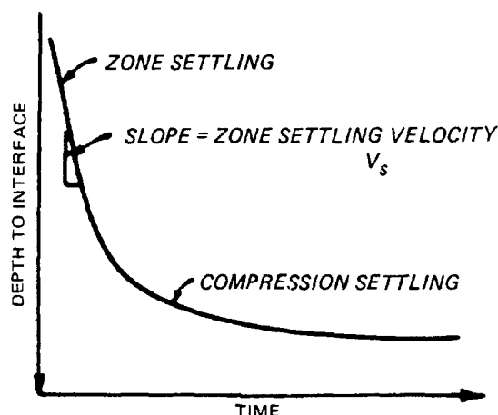
Figure 3-4. Conceptual plot of interface height versus time
