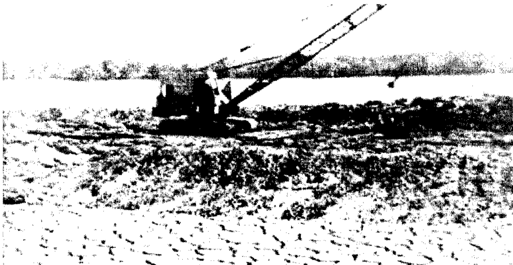
Figure 5-10. Small dragline on mats working on berm deepens shallow perimeter drainage trench
