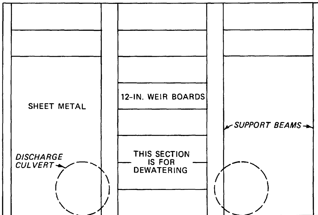
Figure G-4. Frontal view of a weir
