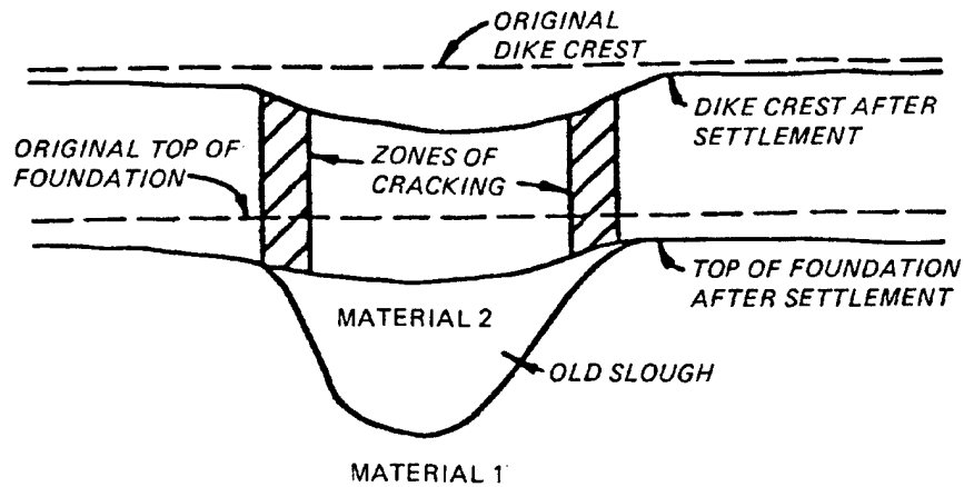
a. COMPRESSIBILITY OF MATERIAL 2 >> MATERIAL 1
