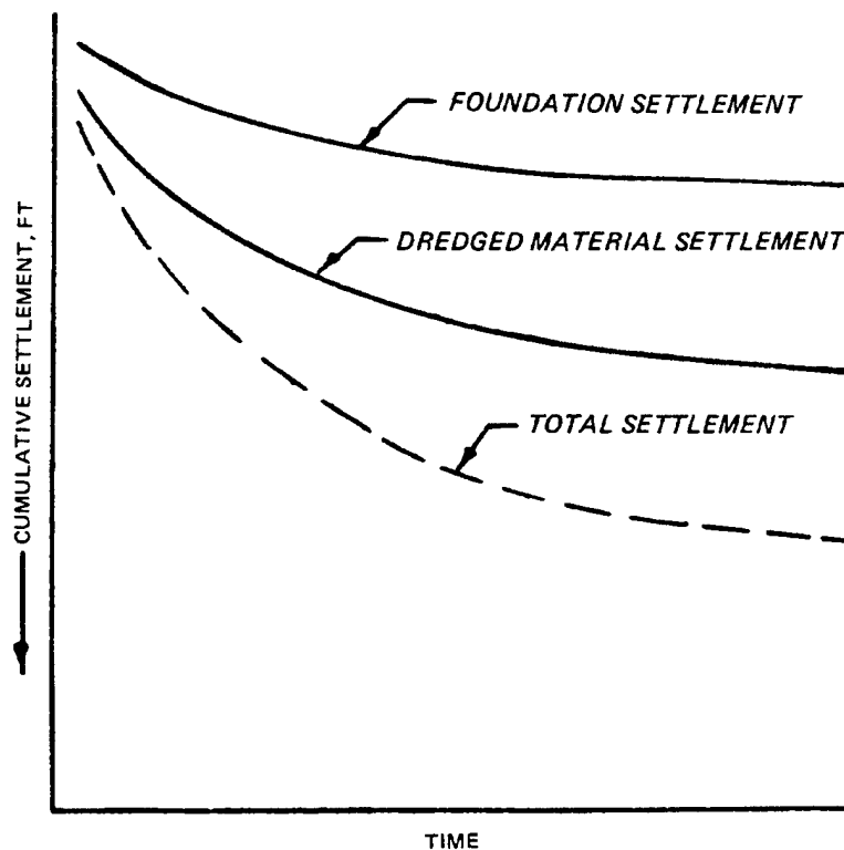
Figure 5-3. Illustrative time-consolidation relationships
