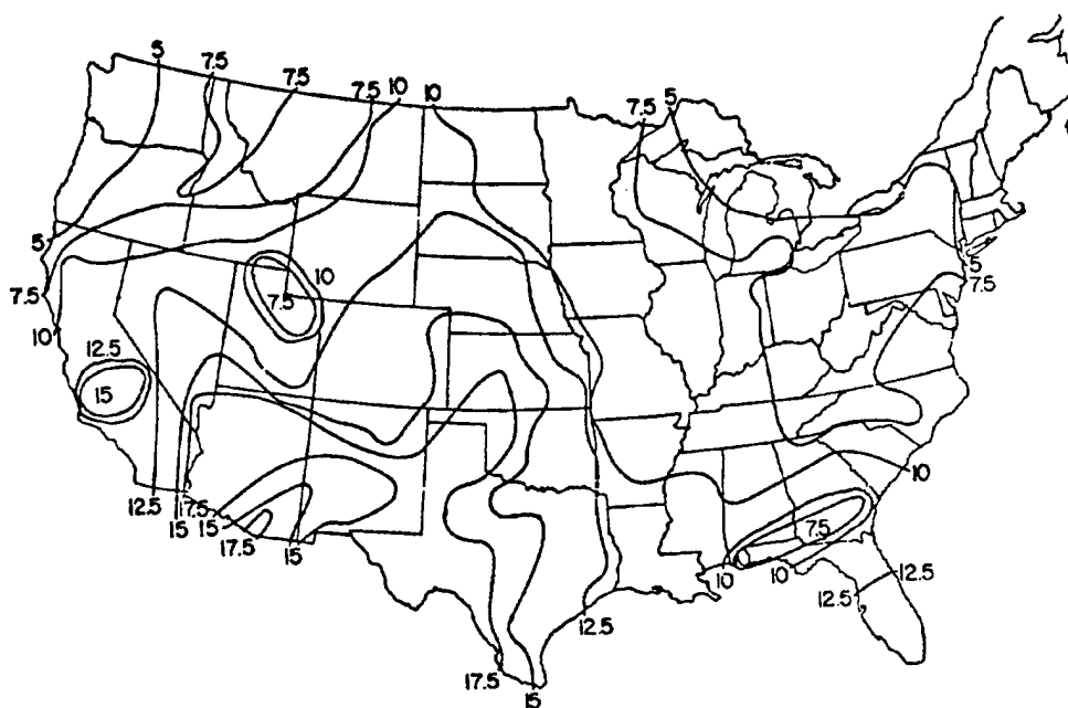
Figure H-10. Average pan evaporation, in centimetres, for the continental United States for the month of October based on data taken from 1931 to 1960
