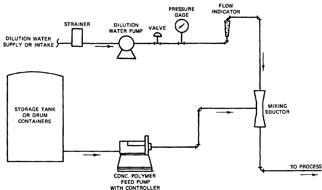
Figure G-1. Schematic of a simple liquid polymer feed system
