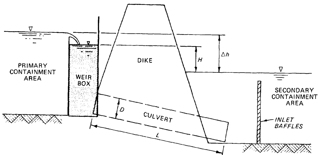
Figure E-1. Example weir mixing system
