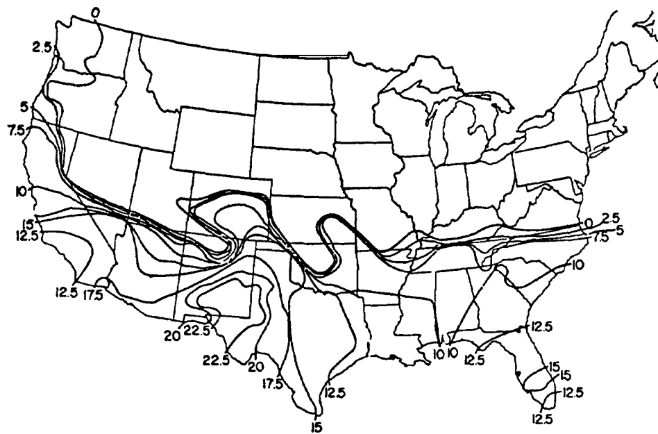
Figure H-3. Average pan evaporation, in centimetres, for the continental United States for the month of March based on data taken from 1931 to 1960
