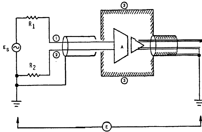
Figure 9-3. A Single Amplifier to Reject Signal E
