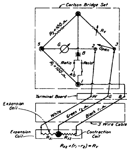
RESISTANCE MEASUREMENT CONTRACTION COIL
