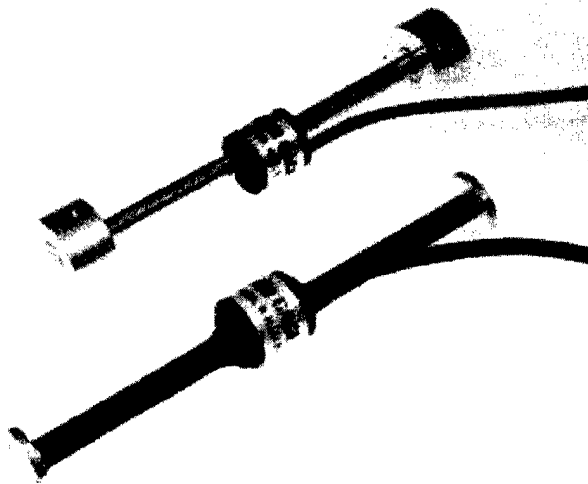
Figure 2-24. Vibrating Wire Strain Gages (Courtesy of Irad Gage, Inc.).
