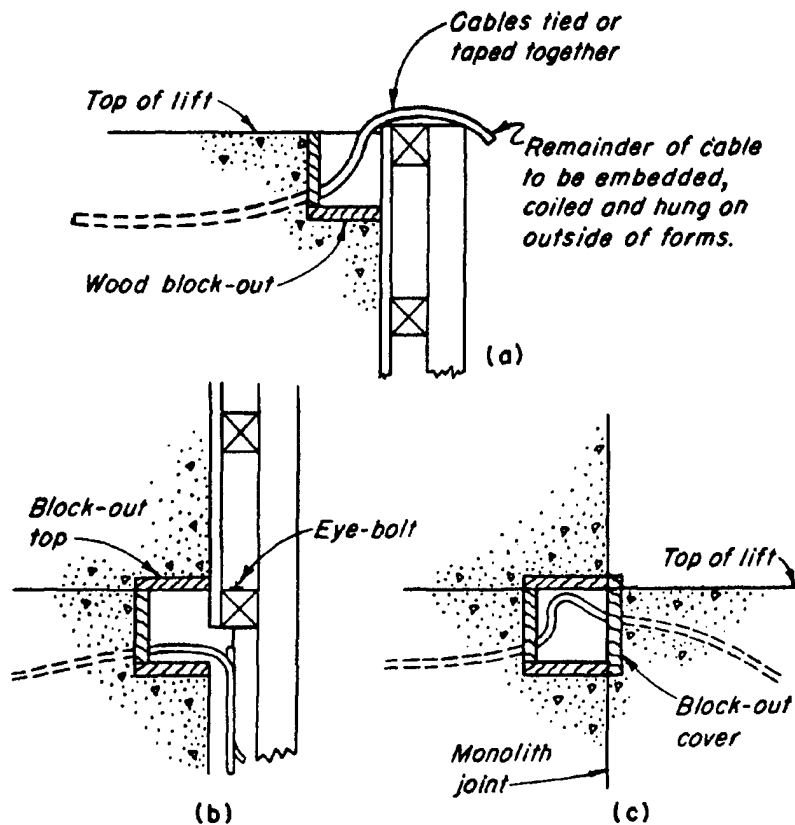
Figure 2-17. Slack Cable Recess. (Prepared by WES)
