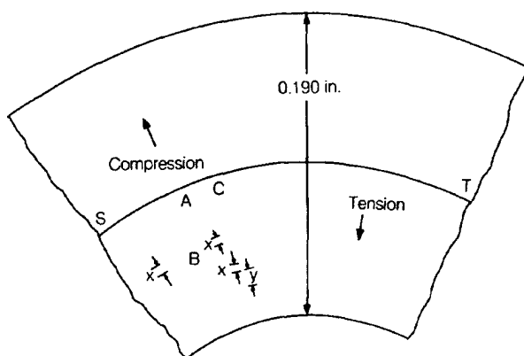
Figure 2-22. Typical Scratch Representation (Courtesy of Prewitt Associates).
