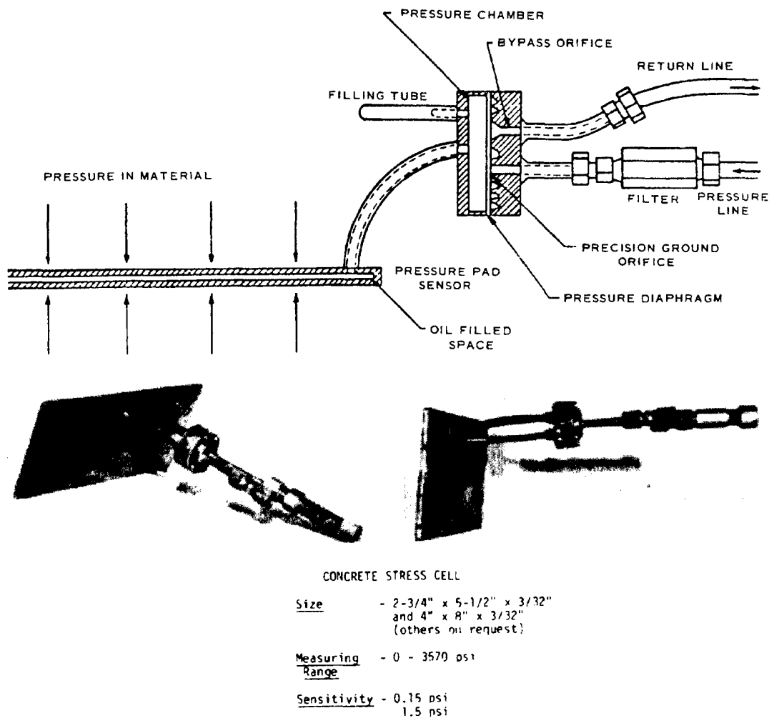
Figure 2-28. Gloetzel Pressure Cell. (by WES, after Terrametrics)
