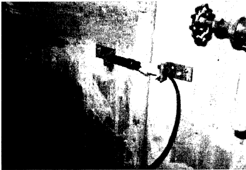
Figure 5-6. Carlson Joint Meter. (Photo by WES)
