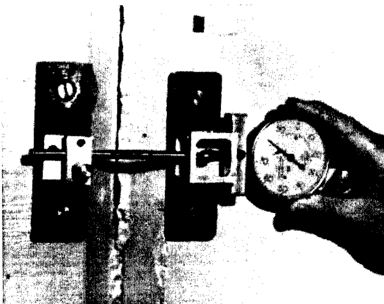
Figure 5-2, Ball-N-Box Gage. (Photo by WES)
