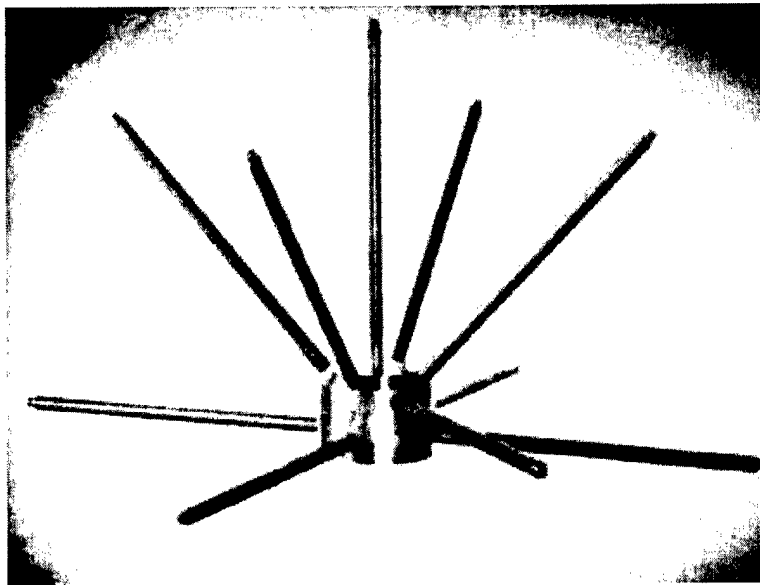
Figure C-2. Carlson Strain Meter Spider. From "Measurement of Structural Action in Dams" by J. M. Raphael and R. W. Carlson.
