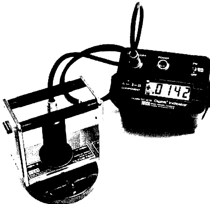
Figure 4-17. Portable Horizontal-Vertical Tiltmeter Sensor in Reading Position on Ceramic Tilt Plate
