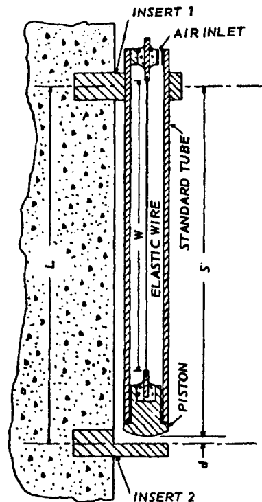
Figure 2-25. Monfore Standardizing Strain Gage. (Prepared by WES)
