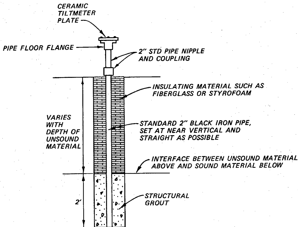
Figure 4-18. Drilled-in Installation of Tiltmeter
