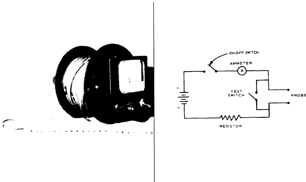
b. Simplified Circuit
