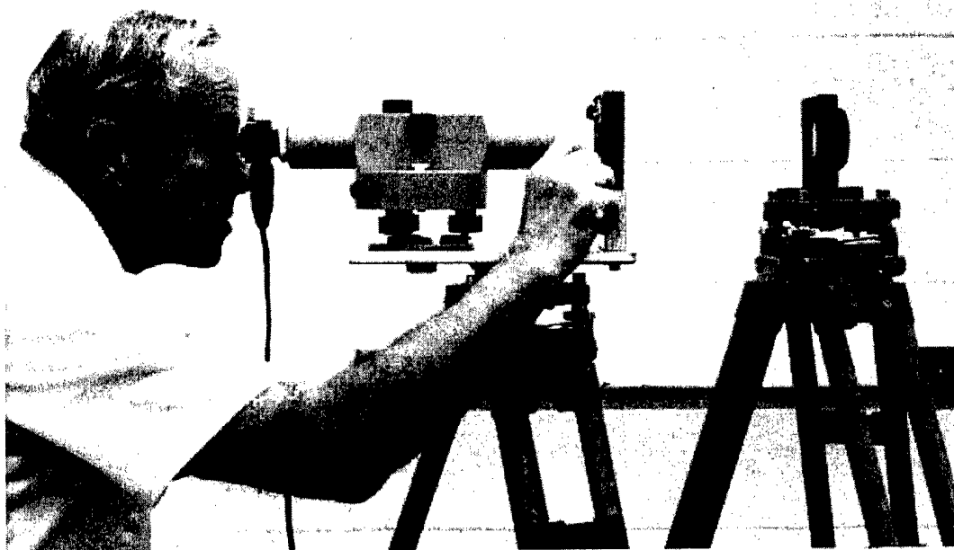
Figure 4-21. Terzaghi Water Level Gage (Courtesy of Soiltest Inc.)
