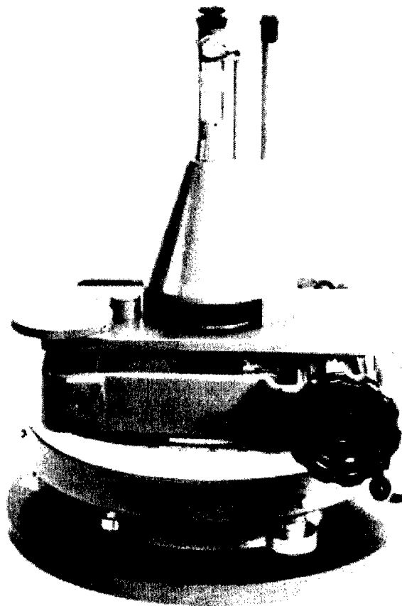
Figure 4-5. Wild GLQ Precision Nadir Plummet (Courtesy of Wild Heerbrugg Ltd.).
