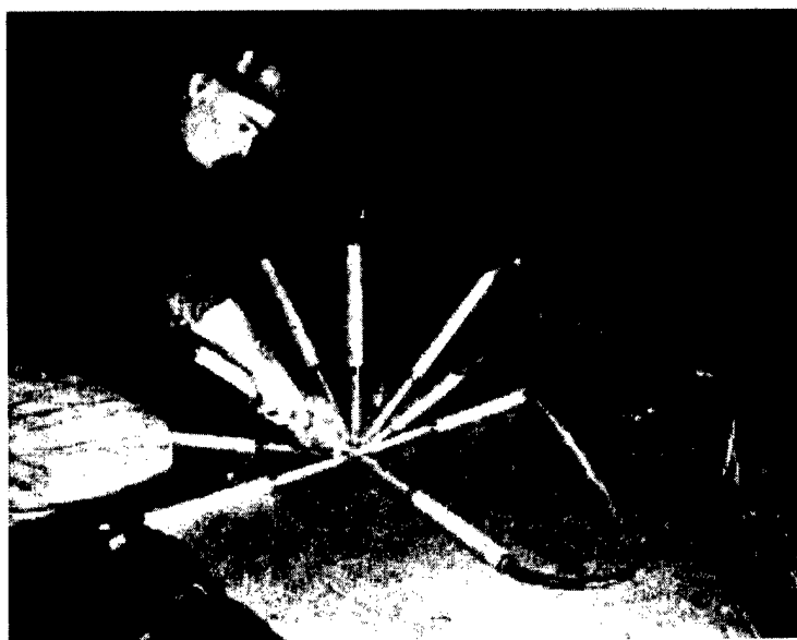
Figure C-3. Strain Meters Mounted on Spider (courtesy of the Bureau of Reclamation).
