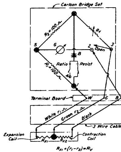
RESISTANCE MEASUREMENT EXPANSION COIL
