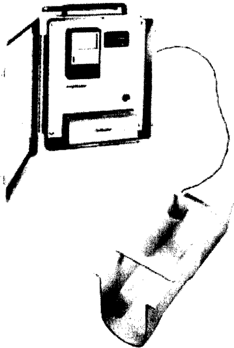
Figure 3-5. Neptune UES Critical Depth Meter (Courtesy of Neptune UES, Inc.).
