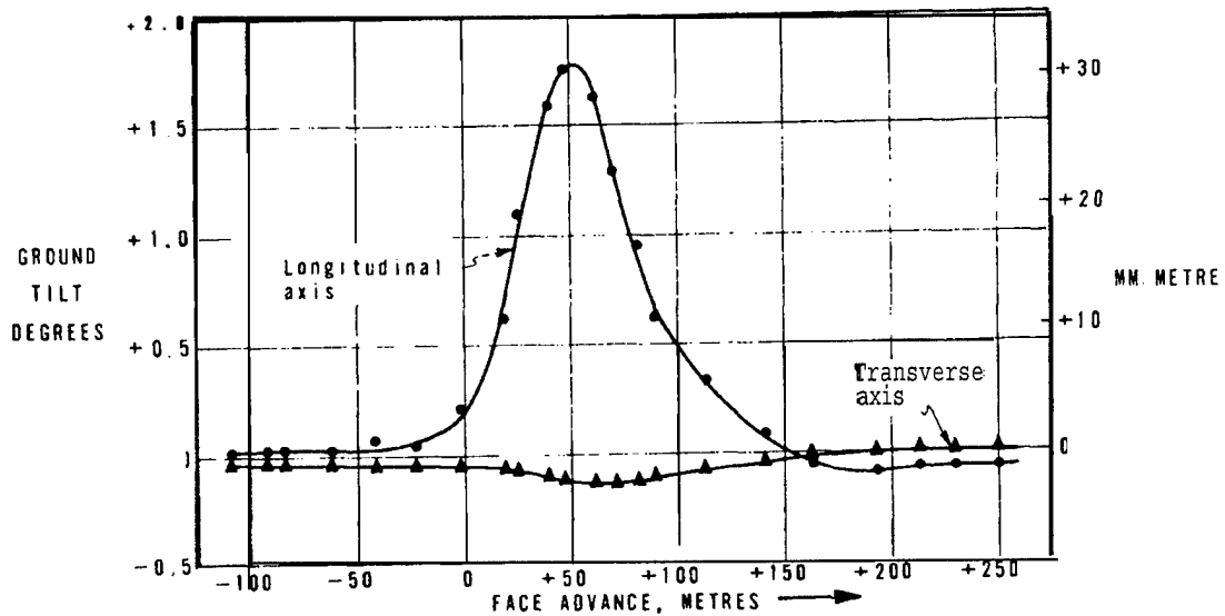
Figure 4-19. Typical Graph of Horizontal-Vertical Tiltmeter Data
