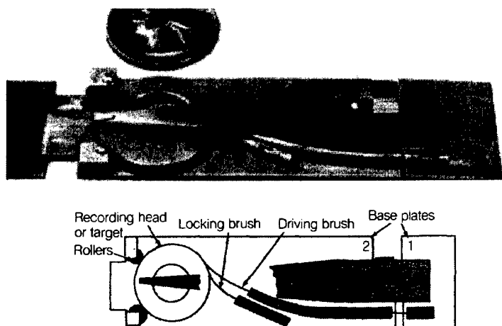
Figure 2-21. Mechanical Scratch Gage (Courtesy of Prewitt Associates).
