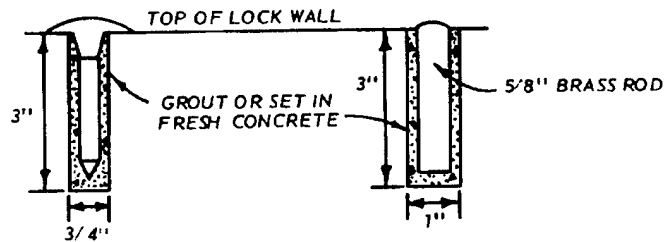
Figure 6-8. Monolith Alignment Markers. (Prepared by WES)
