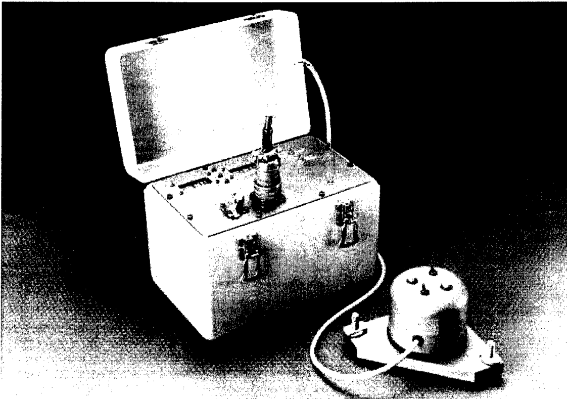
* Figure 4-15. Applied Geomechanics AGI 700 Surface Mount Tiltmeter with Read-Out Box
