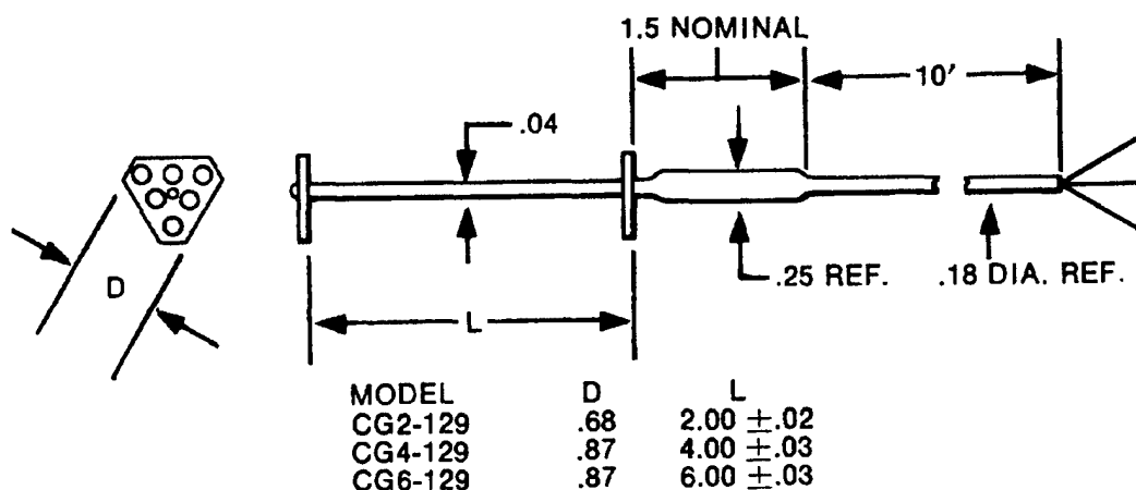
Figure 2-23. Ailtech Embedable Strain Gages (Courtesy of Ailtech).
