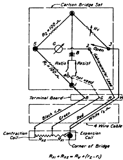
RESISTANCE MEASUREMENT
