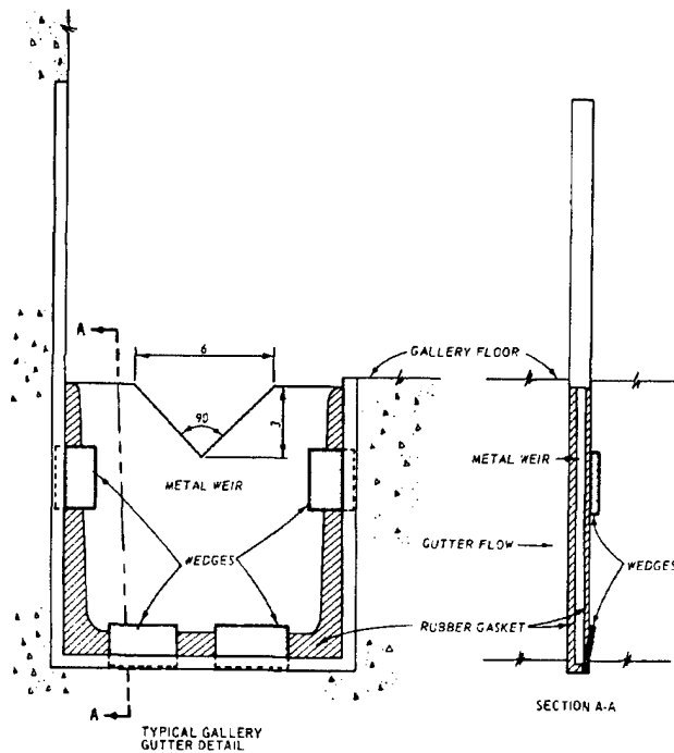
Figure 3-4. Vee-Notch Weir. (Prepared by WES)
