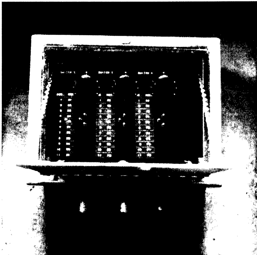
Figure 2-15. Surface-Mounted Terminal Station with Multiple Position Terminal Switches Showing Conduit Fed in from Bottom. (Photo by CE-WES)
