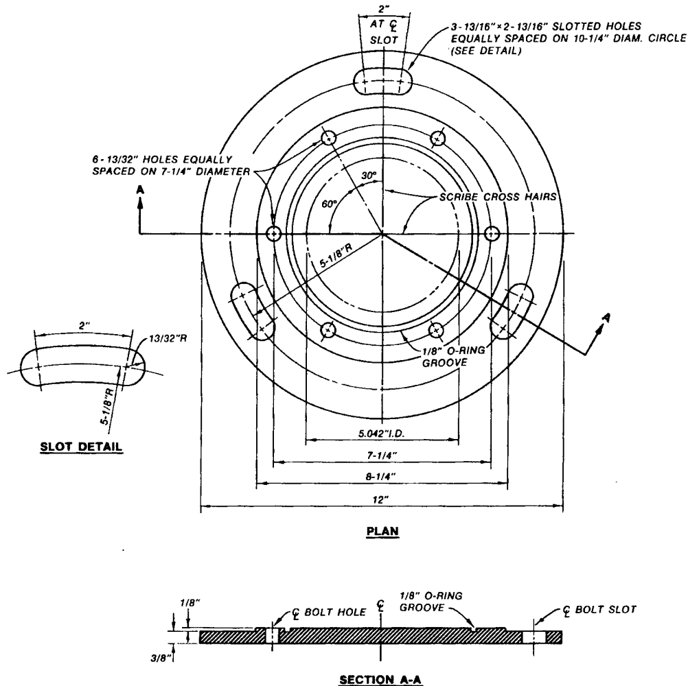
* Figure 4-9. Base Plate of the Wall Deflection Pipe
