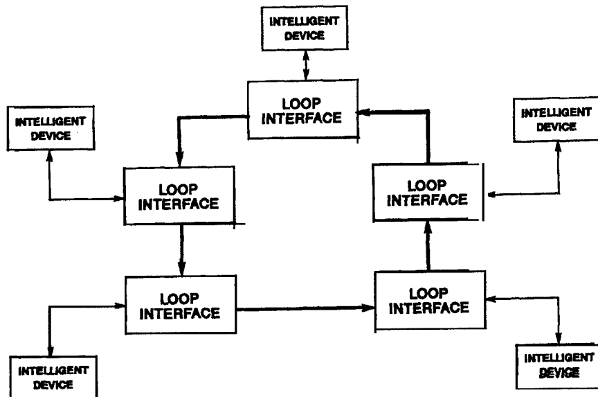
Figure 9-6. Loop Configuration
