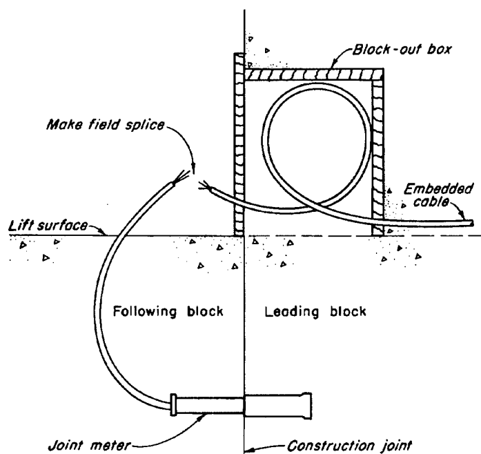
Figure C-15. Joint Meter in Following Block, Cable in Leading Block. (Prepared by WES)
