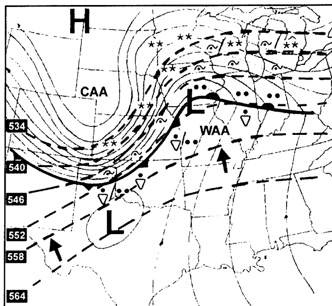
Figure 4-171. Undercutting Freezing Precipitation
