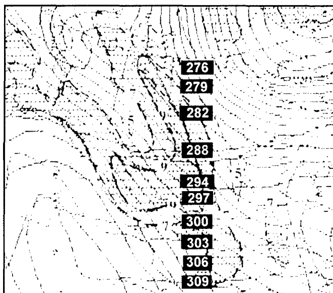
Figure 3-63. 12HR 700 mb HEIGHT/REL HUMIDITY, 1200Z/5 January 1999
