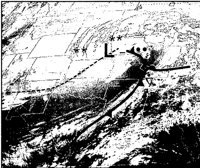
Figure 4-136. GOES-E IR, 0030Z/ 19 February 1984
