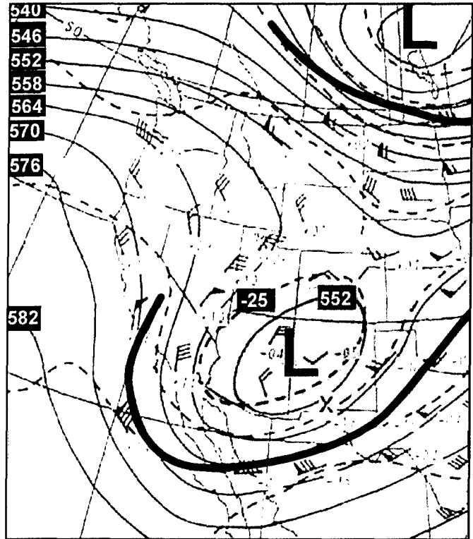
Figure 3-40. 500 mb, 0000Z/30 January 1982
