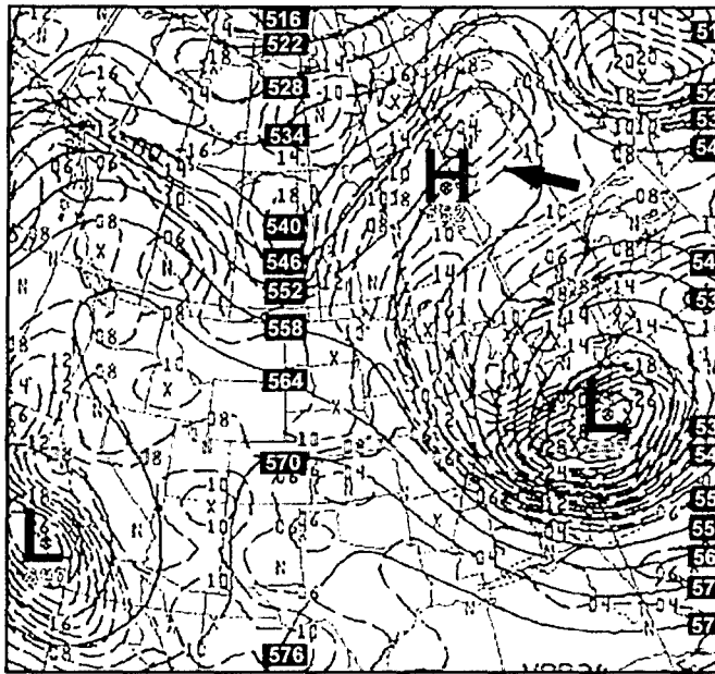
Figure 2-16. 500 mb 36HR FCST HEIGHTS/ VORTICITY, 1200Z/6 March 2001
