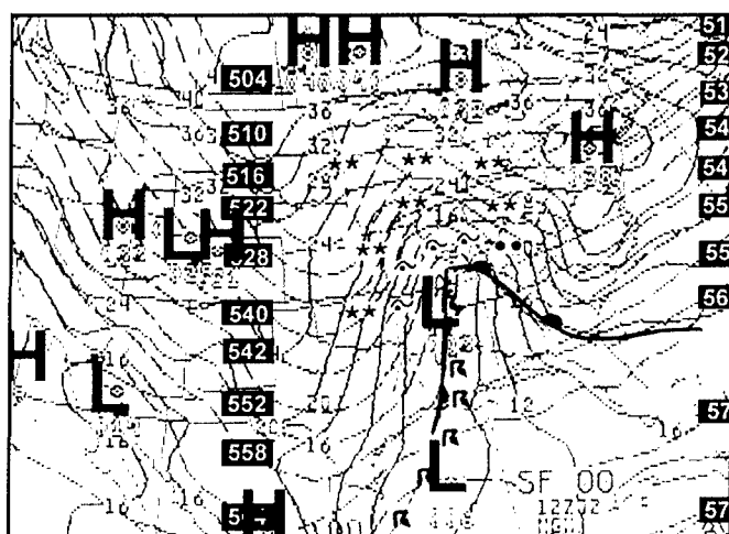
Figure 6-43. 00HR MSL PRES/1000-500 mb THKNS, 1200Z/2 January 1999
