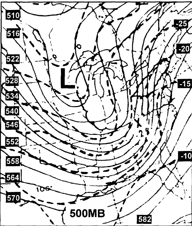
Figure 6-27. 500 mb, 1200Z/10 January 1977
