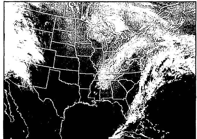
Figure 2-18. GOES-E IR, 0015Z/5 March 2001 Image same valid time as Figures 2-14 and 2-15.
