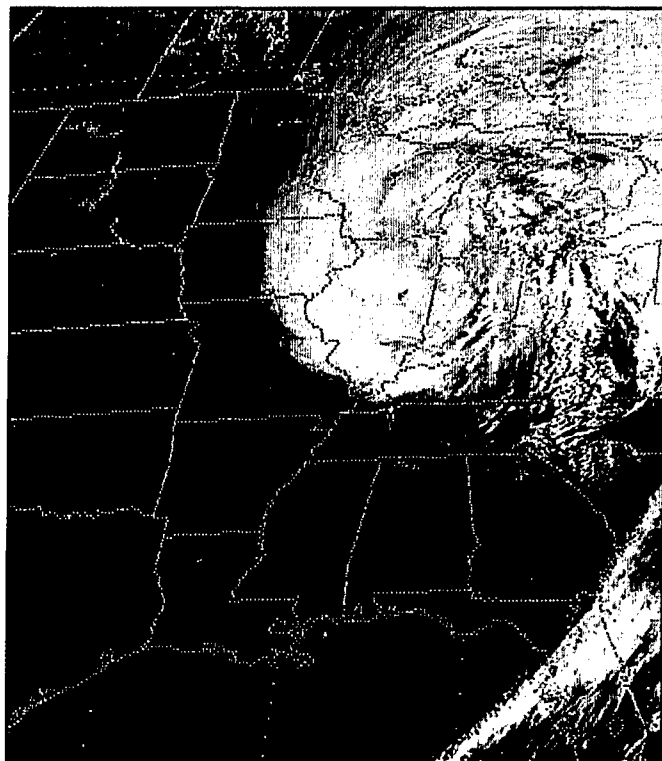
Figure 5-62. GOES-E VIS, 1630Z/ 23 February 1981
