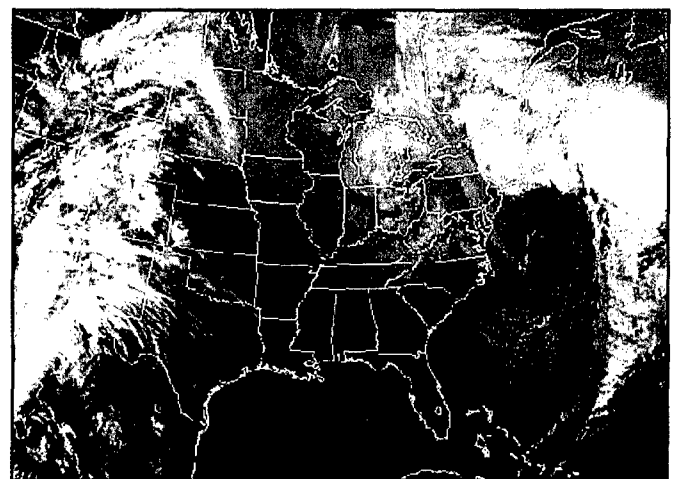
Figure 2-19. GOES-E IR, 0015Z/6 March 2001 Twenty-fours later than Figure 2-18.
