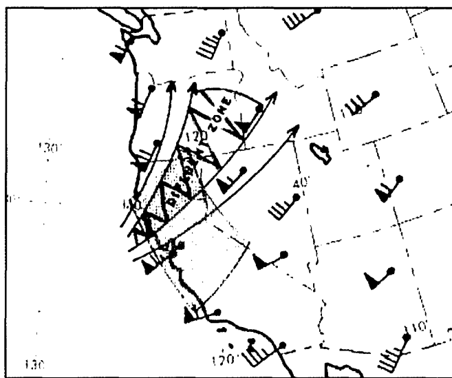
Figure 3-80. Frisco Box Mid-Level Maximum Winds
