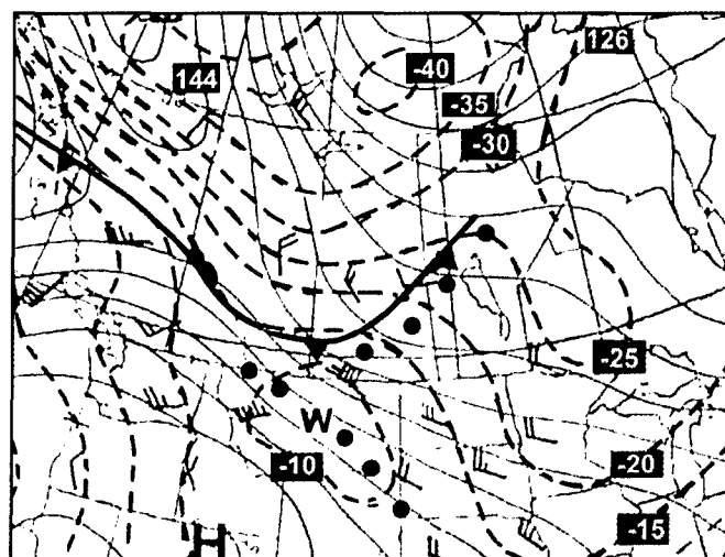
Canadian air masses that are on the move southward may be detected at the 850 mb level. Note that a cold front can be placed in the thermal ridge.
