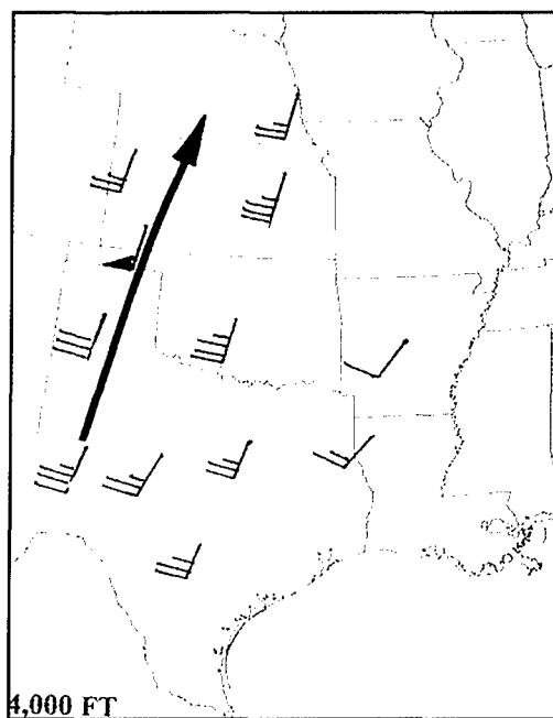
Figure 4-30a. Ideal Gulf Stratus Advection Case - 0600Z
