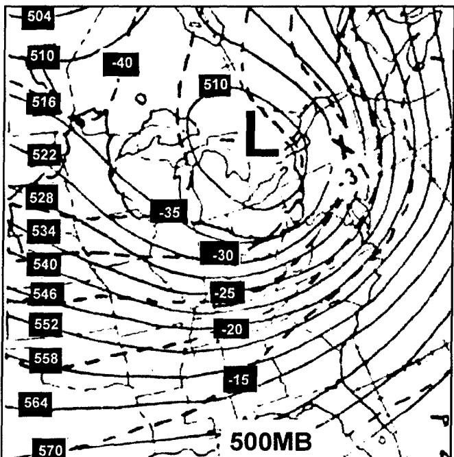
Figure 6-29. 500 mb, 0000Z/11 January 1777
