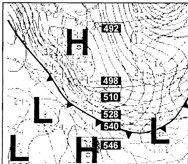
Figure 3-62. Surface, 1200Z/5 January 1999
