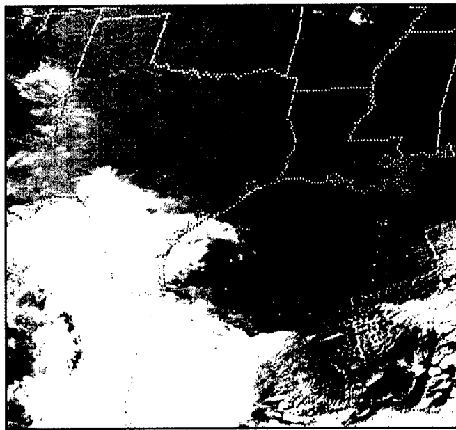
Figure 4-57. GOES-E VIS, 1740Z/ 3 February 1981
