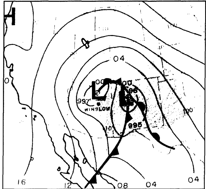
Figure 4-150. Dusty Box Surface
