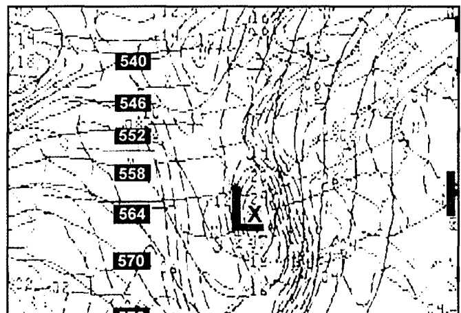
Figure 5-56. 24HR 500 mb HEIGHTS/VORTICITY, 1200Z/23 January 1999
