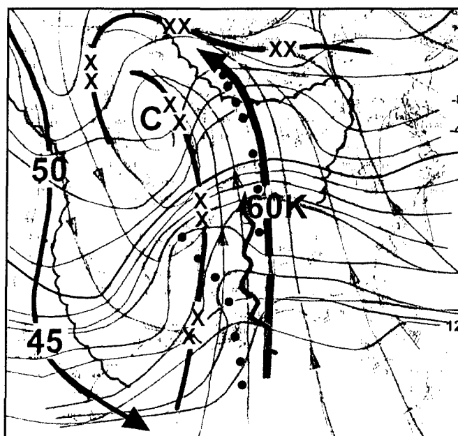
Figure 6-45. 850 mb Analysis, 1200Z/2 January 1999
