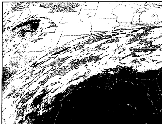
Figure 4-94. GOES-E IR, 0900Z/21 January 1982 Extensive jet stream cirrus shown over the southern CONUS. Short wave comma cloud system shown over the western CONUS.
