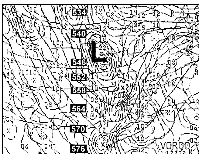
Figure 6-42. 00HR 500 mb HEIGHTS/VORTICITY, 1200Z/2 January 1999
