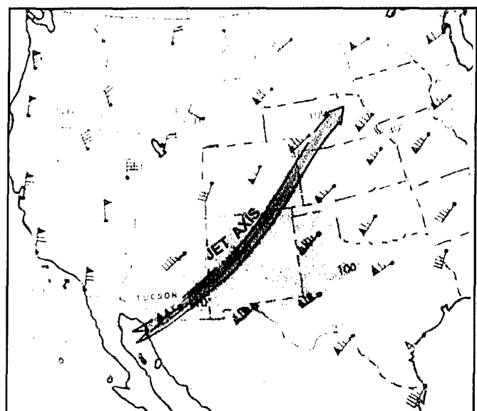
Figure 4-151. Dusty Box Mid-Level Maximum Winds
