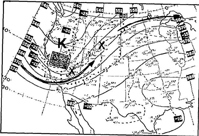
Figure 2-5. 500 mb, 0000Z/2 December 1973
