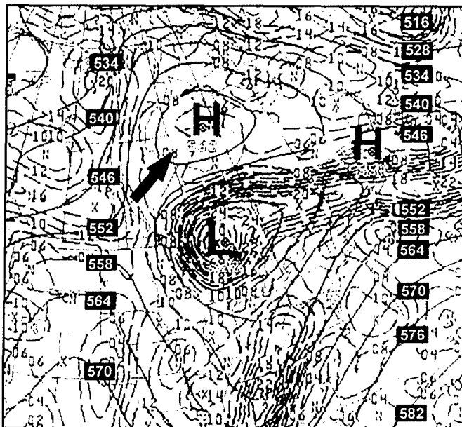
Figure 2-14. 500 mb ANALYSIS HEIGHTS/VORTICITY, 0000Z/5 March 2001 Black arrow notes building high pressure system.
