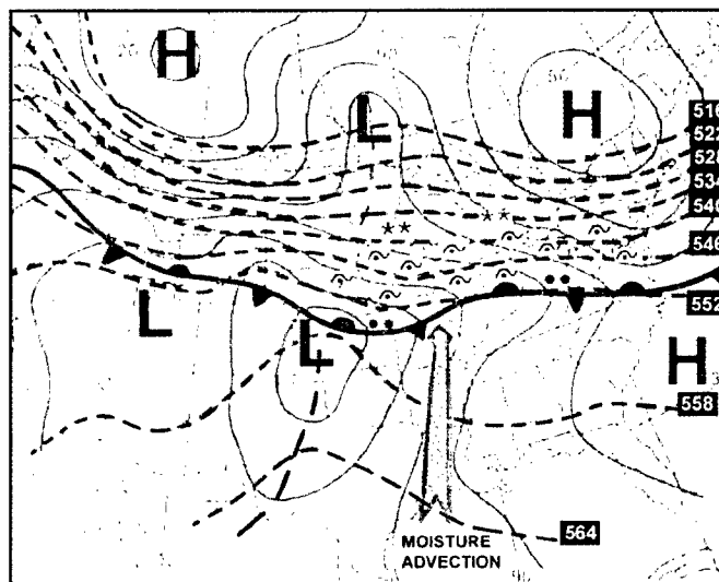
Figure 4-178. 00HR MSL PRES/1000-500 mb THKNS, 0000Z/27 February 1995
