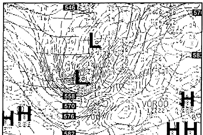
Figure 5-52. 00HR 500 mb HEIGHTS/VORTICITY, 1200Z/22 January 1999
