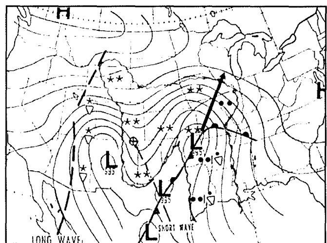
Figure 4-103. Day 2 Surface, 1200Z/ 2 January 1971
