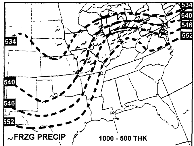
Figure 4-159. Thickness Ridge and 6-Hour Observed Freezing Precipitation, 1200Z/ 11 January 1991
