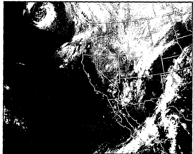
Figure 3-19. GOES-W IR, 1200Z/ 8 February 2001
