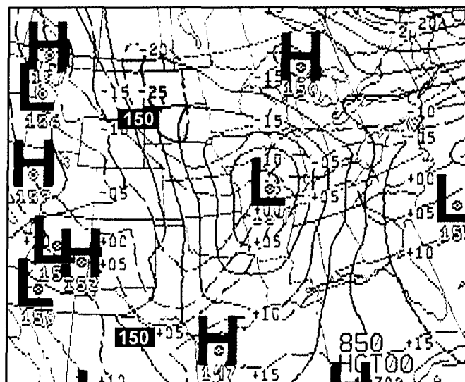
Figure 6-44. 00HR 850 mb HEIGHTS/TEMPS, 1200Z/2 January 1999
