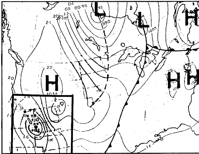
Figure 4-145. Northern Plains Box, Secondary Troughs Example
