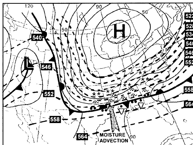
Figure 4-177. Typical Overrunning Situation
