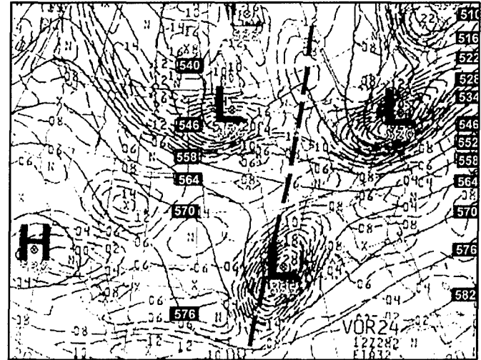
Figure 2-10. 24HR FCST 500 mb HEIGHTS/VORTICITY, 1200Z/28 December 2000 Long wave (dashed line) was located over the central CONUS during most of December. Short waves were moving through the long wave.
