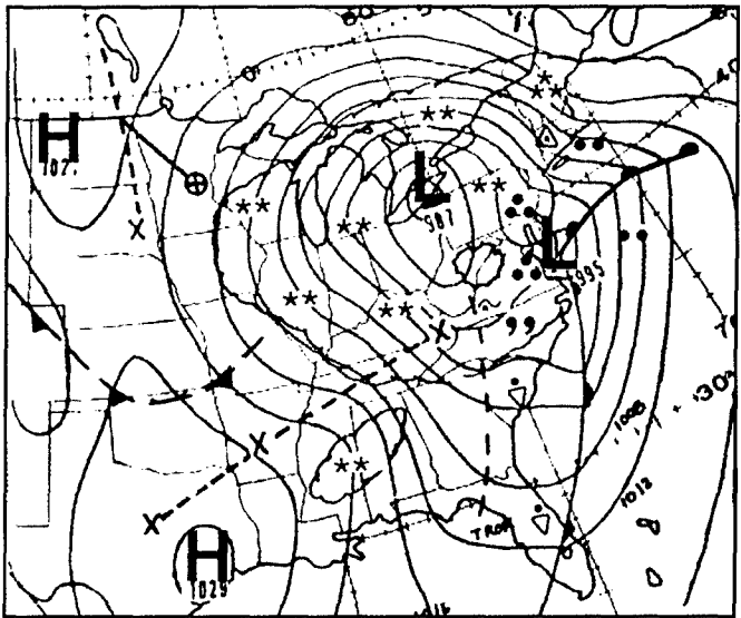
Figure 6-28. Surface, 1200Z/10 January 1977
