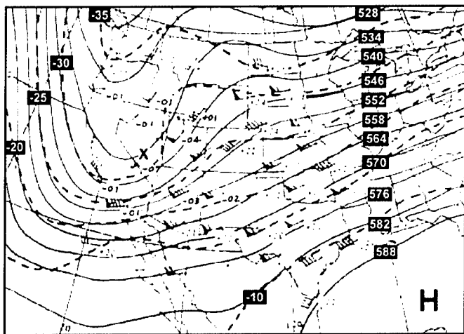
Figure 4-92. 500 mb, 1200Z/21 January 1982 90 knot jet max at the base of West Coast trough. Wide spacing of contours over northern California and Nevada suggest cyclogenesis.
