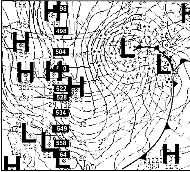
Figure 6-51. 00HR MSL PRES/1000-500 mb THKNS, 1200Z/3 January 1999
