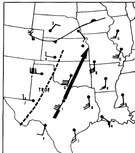
Figure 4-24. Low-Level Jet Formation Model
