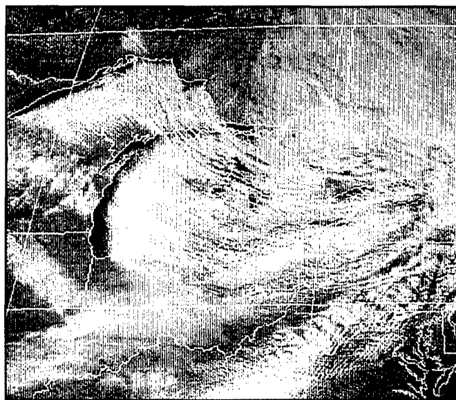
Figure 5-103. GOES-E VIS, 1855Z/ 5 December 2000
