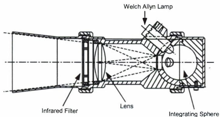
Figure 8. EO-1 ALI internal reference source.
