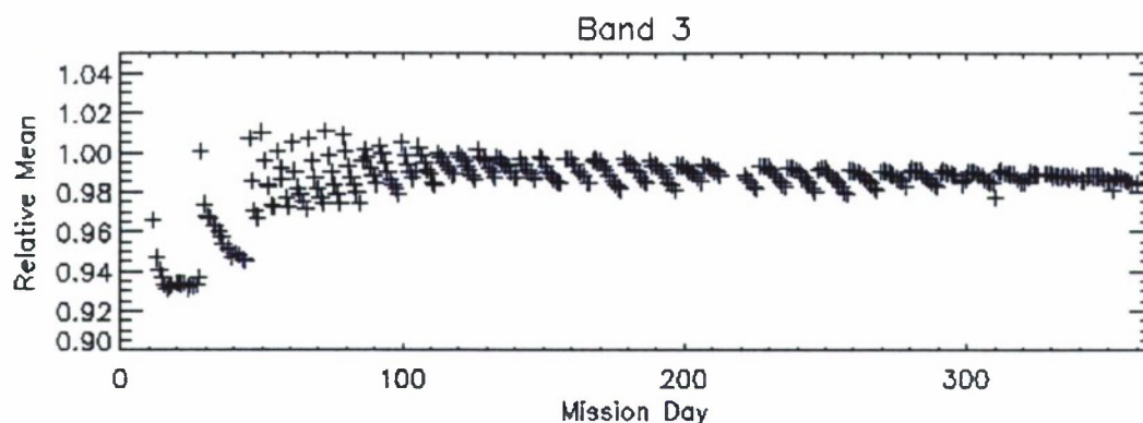
Figure 11. Effects of contamination on Band 3 data. Each point is derived from internal lamp data that has been ratioed to data obtained on Day 5 of the mission.
