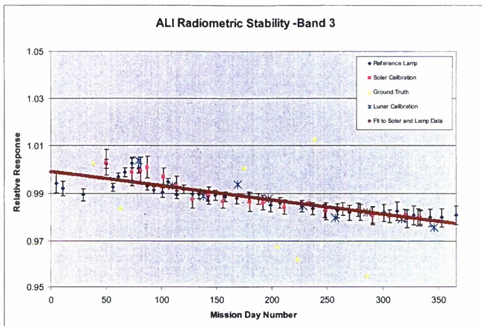
Figure 22. Trending of ALI radiometric calibration data for Band 3.
