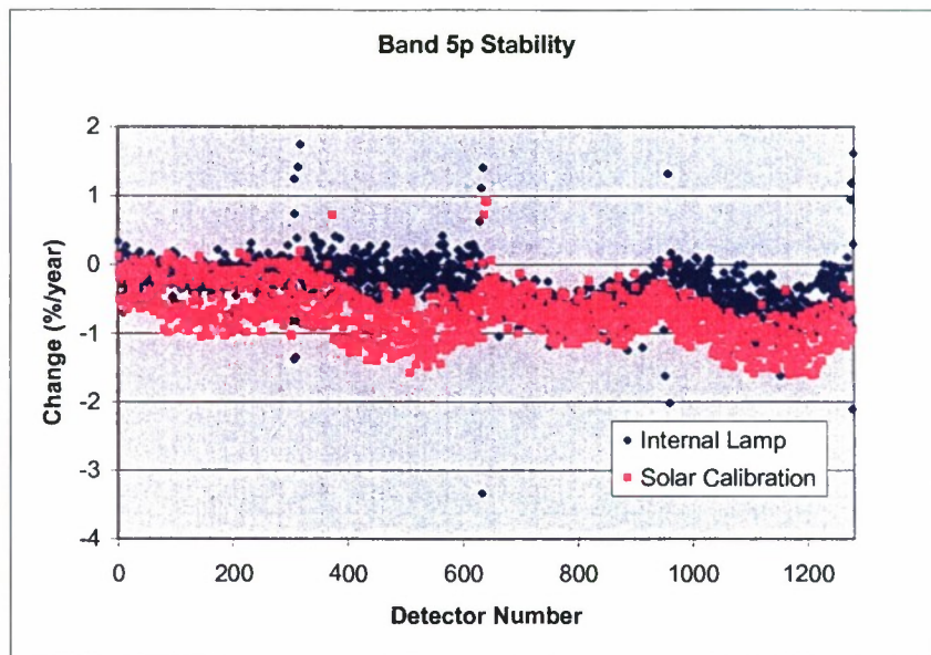
Figure 35. Radiometric stability of detectors for Band 5p as determined by internal lamp and solar calibration data collected during the first year on orbit.
