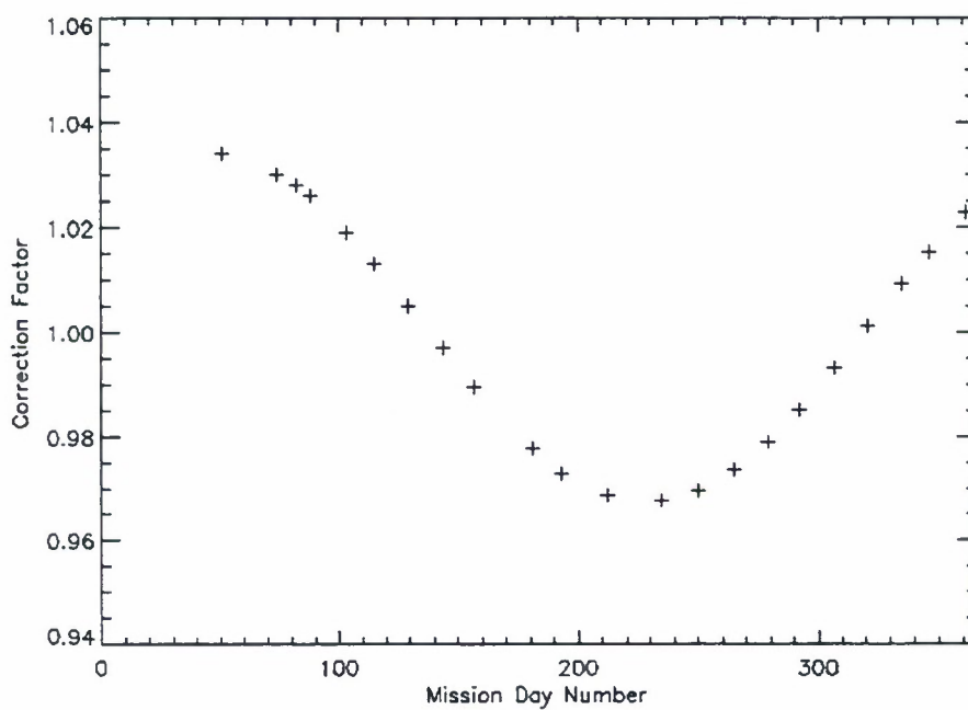
Figure 12. Solar calibration correction factors.
