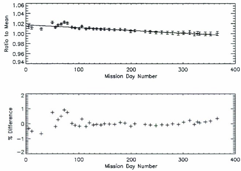
Figure 17. Band 3 instrument response stability based on internal reference lamp data.
