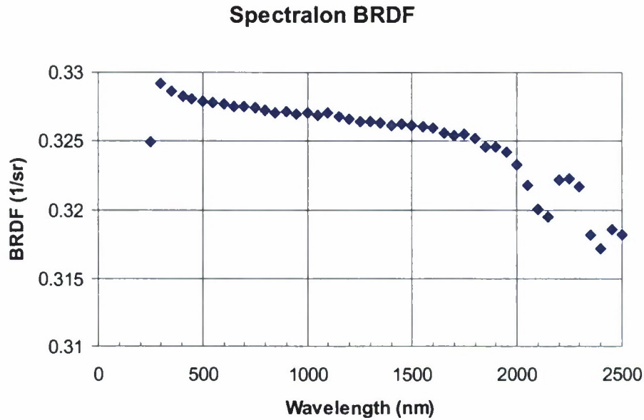
Figure 3. BRDF of diffuser located in front of the ALI secondary mirror used in the solar calibration model.
