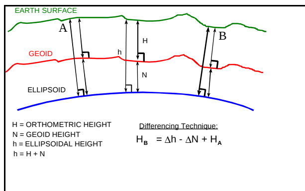
Figure 1. Geoid/Ellipsoid Relationship
