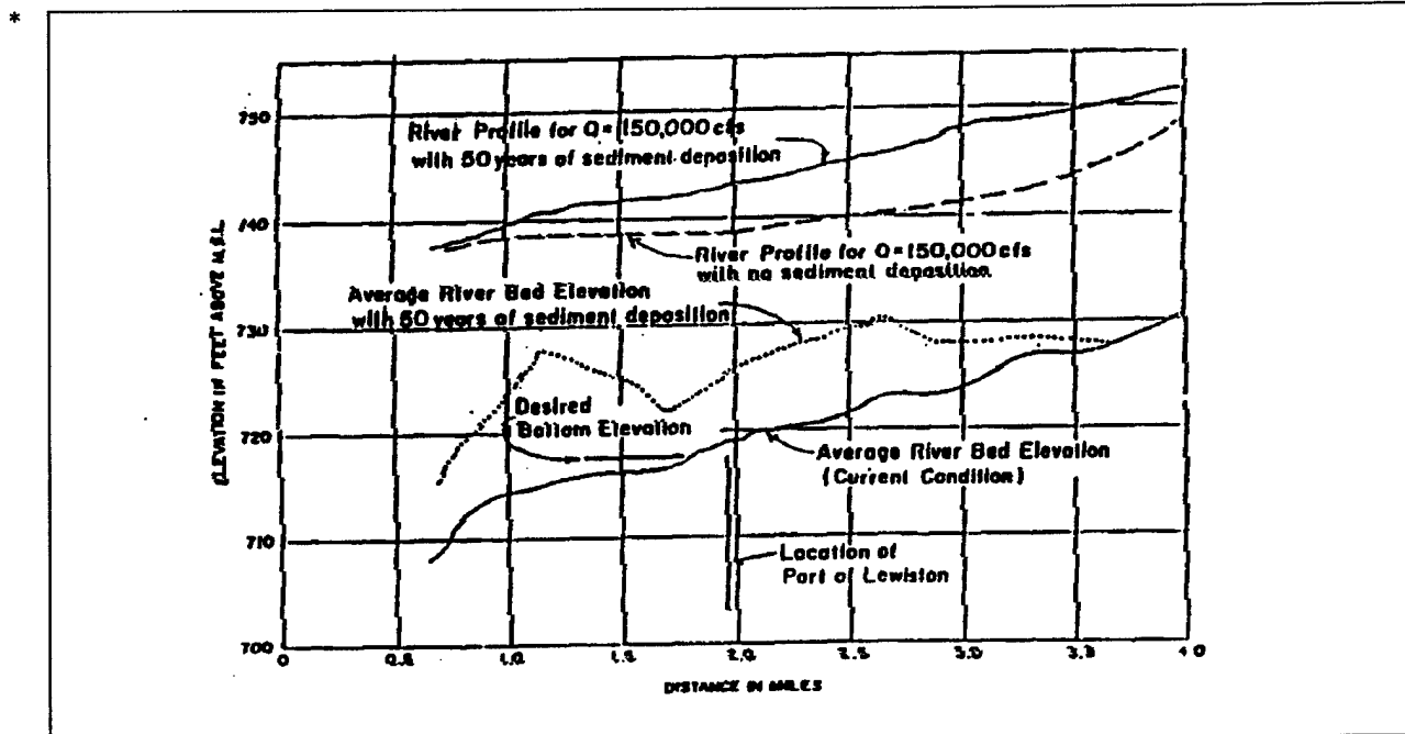
Figure 10-9. Water-surface and bed-surface profiles
