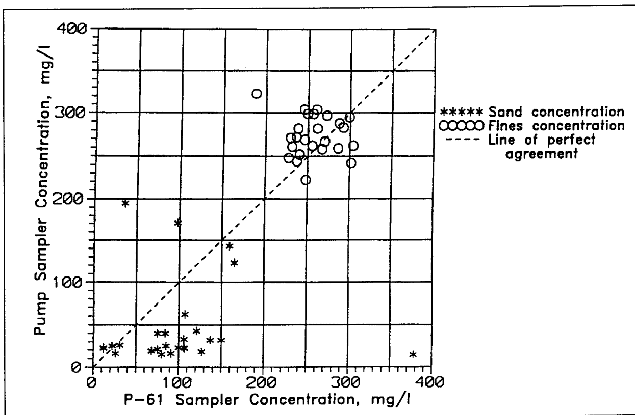
Figure 8-1. Comparison of sediment load measured with pump and US P-61 samplers
