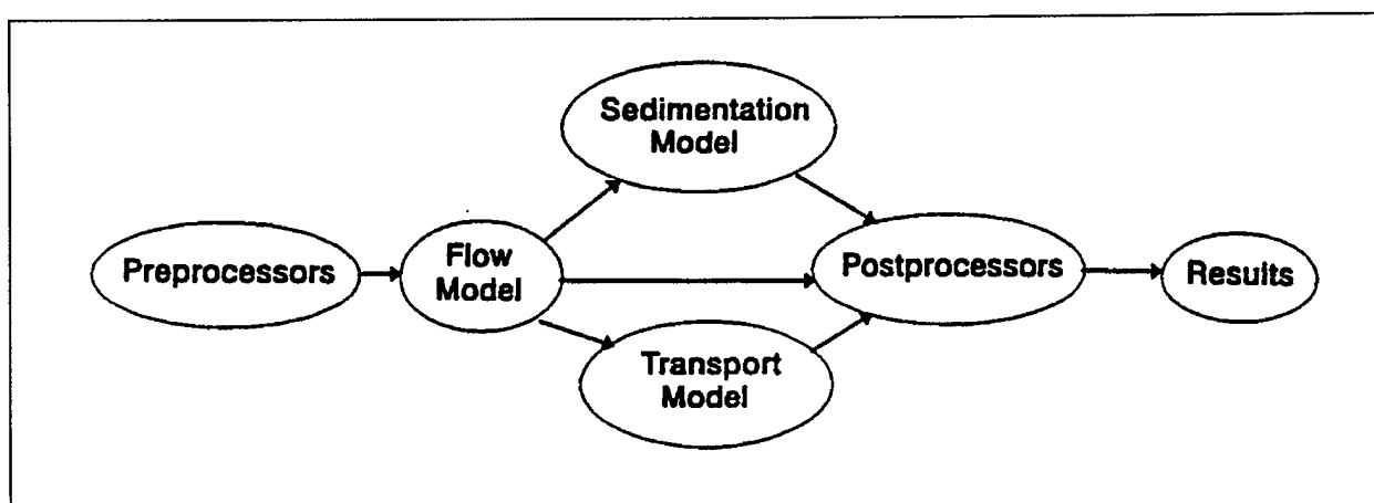
Figure 10-12. TABS-2 schematic
