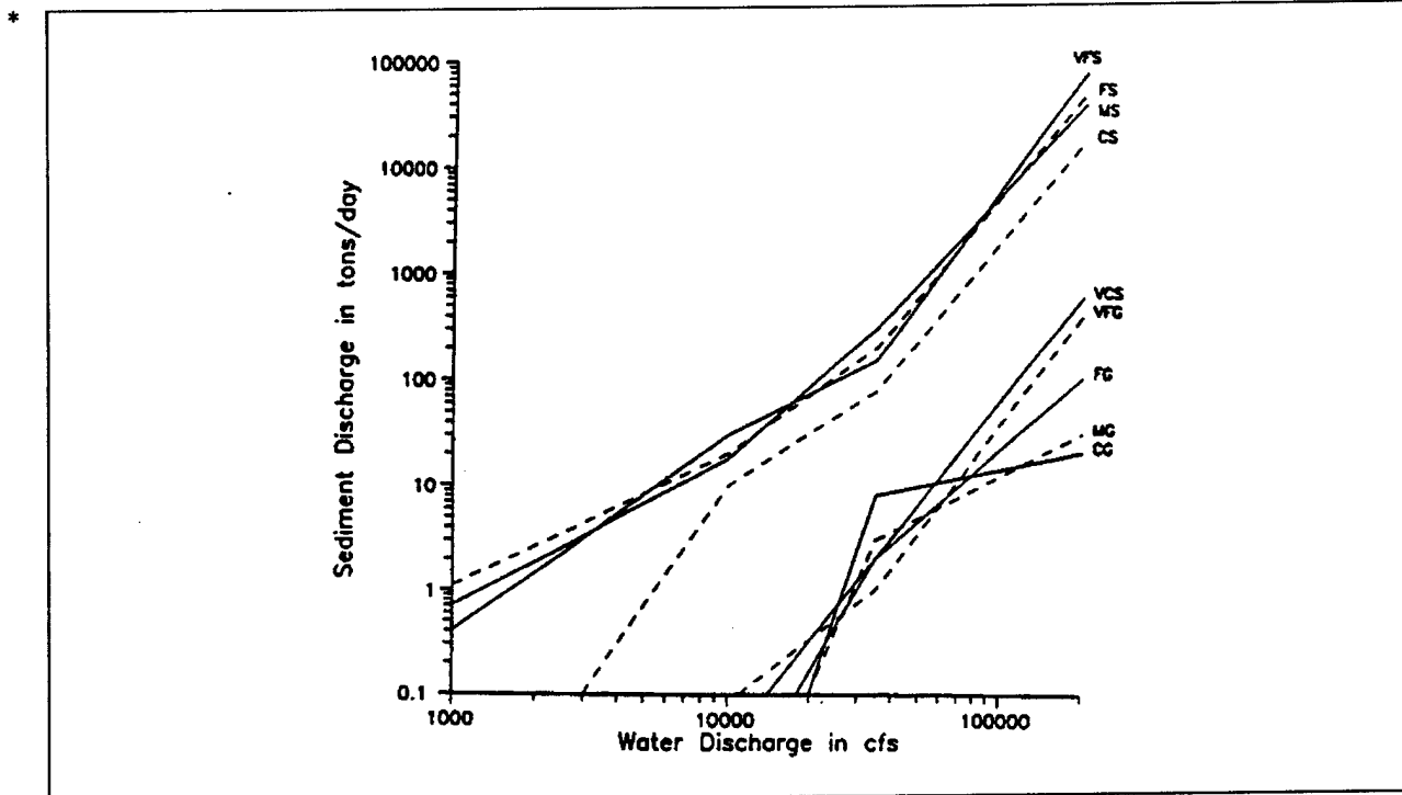
Figure 10-6. Sediment load curves
