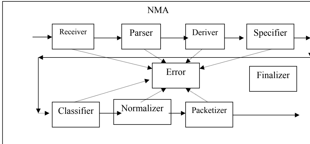
Figure 17 - Internal Box Diagram of NMA Module
