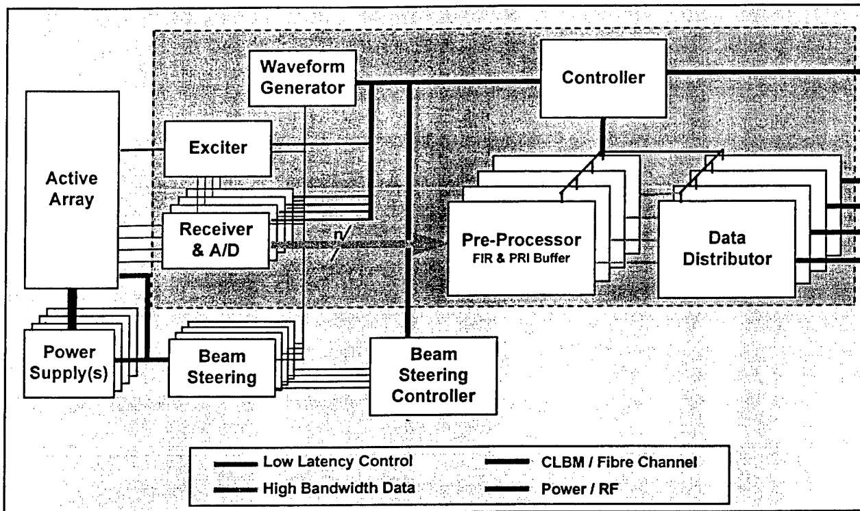
Figure 6.2.1-1. Notional Radar Architecture Featuring A Data Distribution Function
