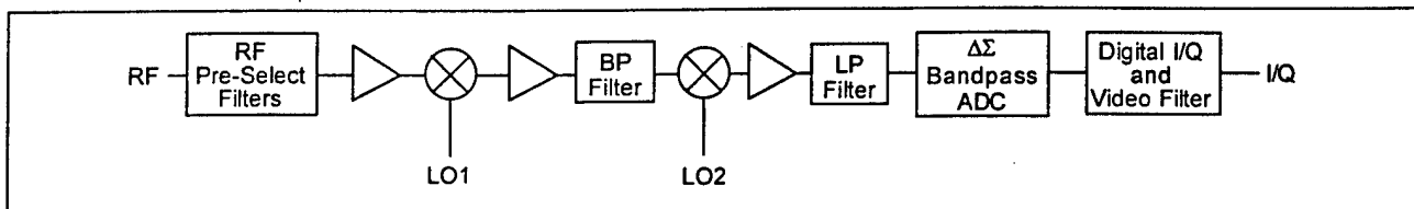
Figure 5.3.1-2. Second IF Sampling Digital I/Q Receiver
