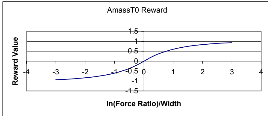
Figure 5. “Smooth Delta Function” of the “Amass” Value Component (From: [Ref 6])
