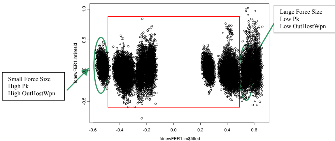
Figure 27. Residual Plot of the FER Model from the Factorial Design
