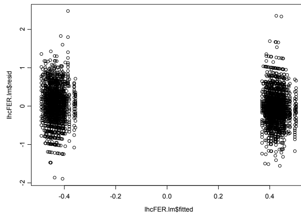
Figure 22. Residual Plot of the FER Model from the Latin Hypercube Design
