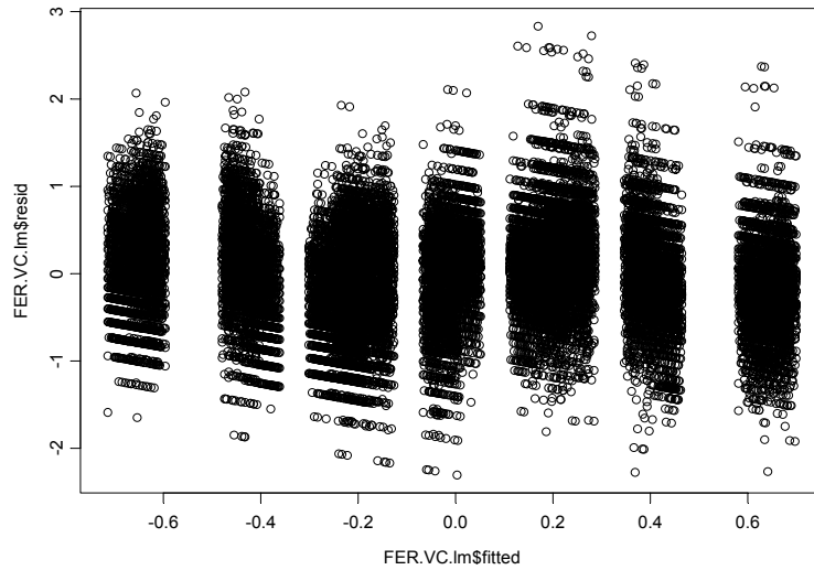
Figure 28. Residual Plot of the FER Model for Small Force Size Scenario from Virginia Cluster's Output
