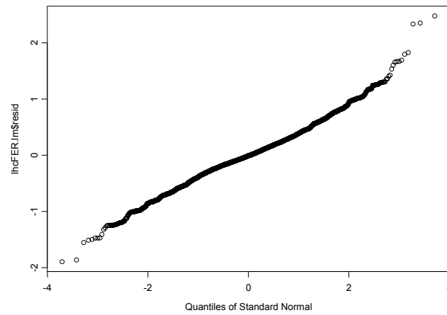
Figure 21. QQ-plot of the FER Model from the Latin Hypercube Design
