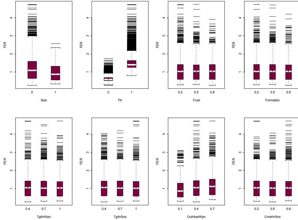
Figure 25. Boxplot of Factors for the FER from the Factorial Design
