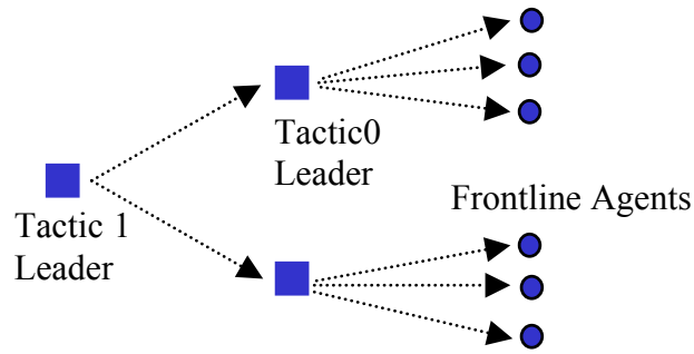
Figure 2. Unit Hierarchy in SOCRATES (From: [Ref 4])
