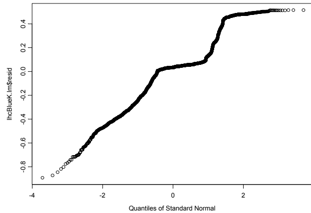
Figure 14. QQ-plot of the PercentBlueKilled Model from the Latin Hypercube Design
