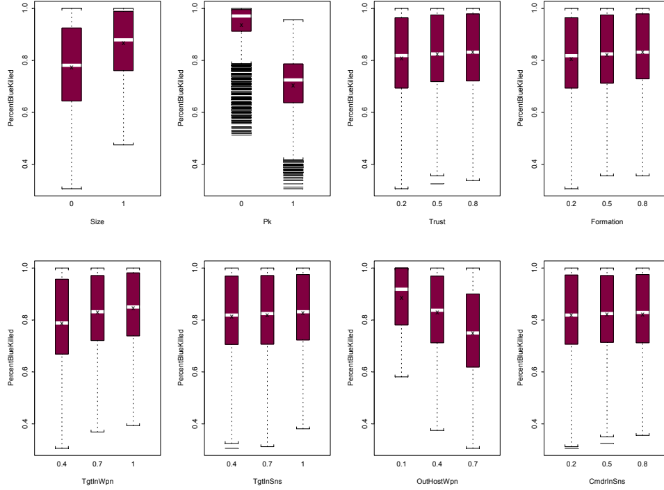
Figure 18. Boxplot of Factors for PercentBlueKilled from the Factorial Design
