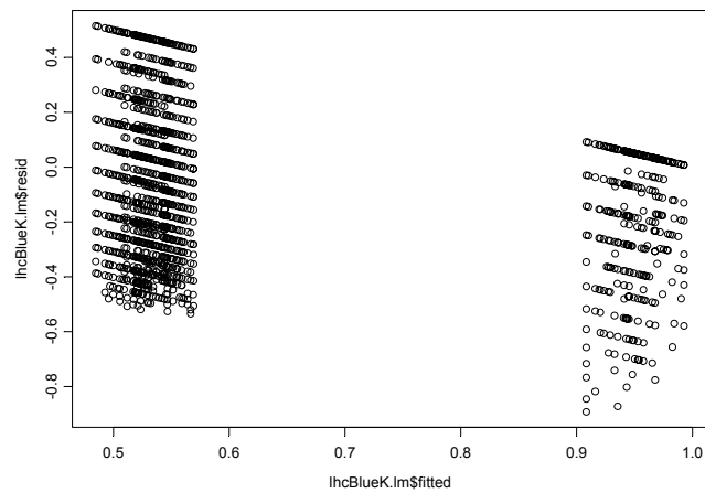
Figure 15. Residual Plot of the PercentBlueKilled Model from the Latin Hypercube Design
