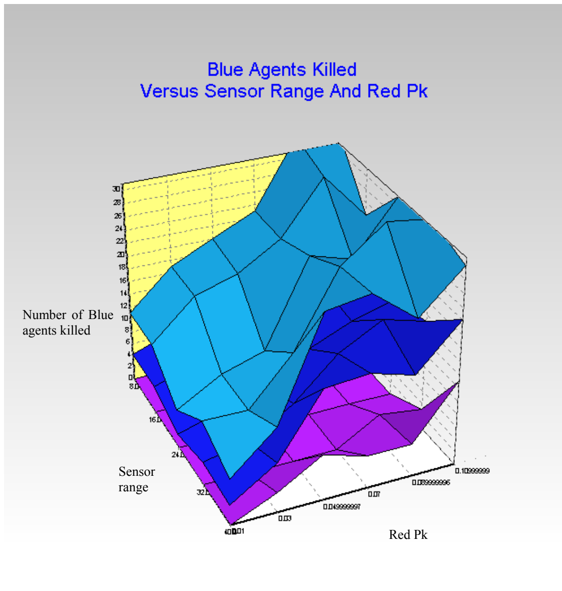
Figure 9. Typical Three-dimensional Graph of a MOE vs Input Variables
