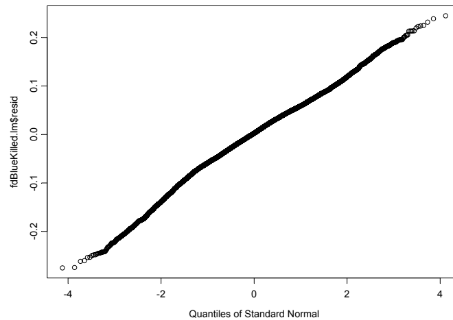
Figure 19. QQ-plot of the PercentBlueKilled Model from the Factorial Design
