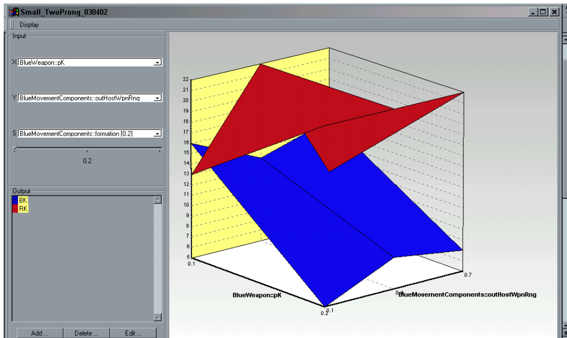
Figure 30. Three-dimensional Plot of the Relationships Between the Pk, Formation (=0.2) and OutHostWpn for Small Total Force Size
