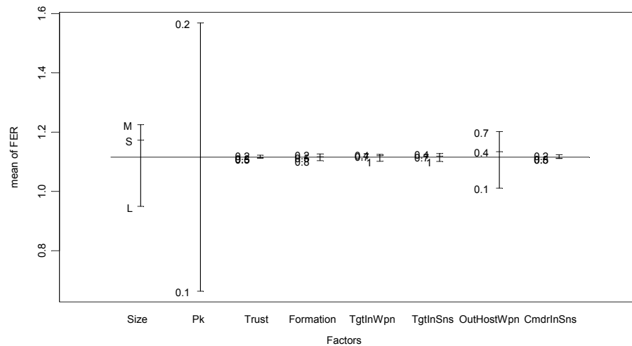
Figure 24. Plot of Treatment Means for FER from the Factorial Design
