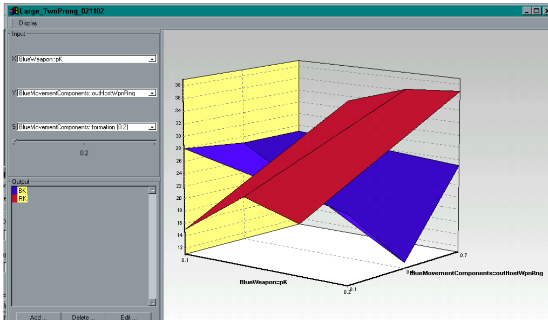
Figure 31. Three-dimensional Plot of the Relationships Between the Pk, Formation (=0.2) and OutHostWpn for Large Total Force Size
