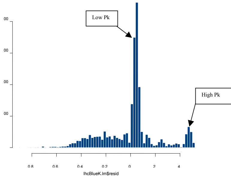
Figure 16. Histogram of the Residuals of the PercentBlueKilled Model from the Latin Hypercube Design
