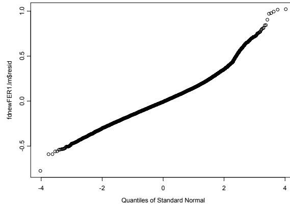
Figure 26. QQ-plot of the FER Model from the Factorial Design
