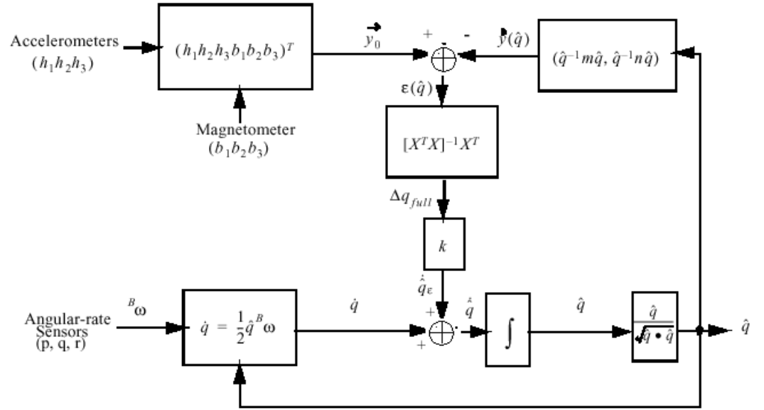
Figure 7. Quaternion based orientation filter.
