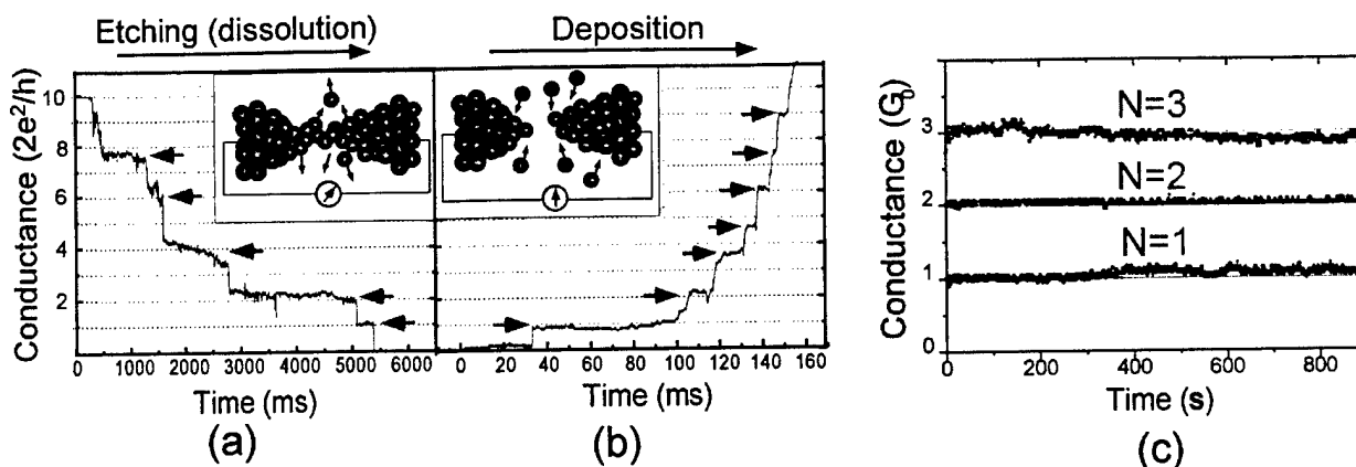
Fig. 2 (a-b) Conductance of a Cu quantum wire during etching (a) and deposition (b). The stepwise change is due to conductance quantization. (c) Stable Cu nanowires with conductance at N=1, 2 and 3 quantum steps.
