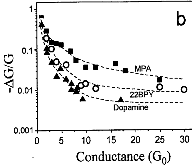
Fig. 3. (a) Conductance change of Cu quantum wires with conductance quantized at 1, 2, 3 and 4G_0 upon MPA adsorption. (b). Comparison of dopamine-, MPA- and 22BPY-induced conductance changes of Cu nanowire with conductance at various quantum steps.
