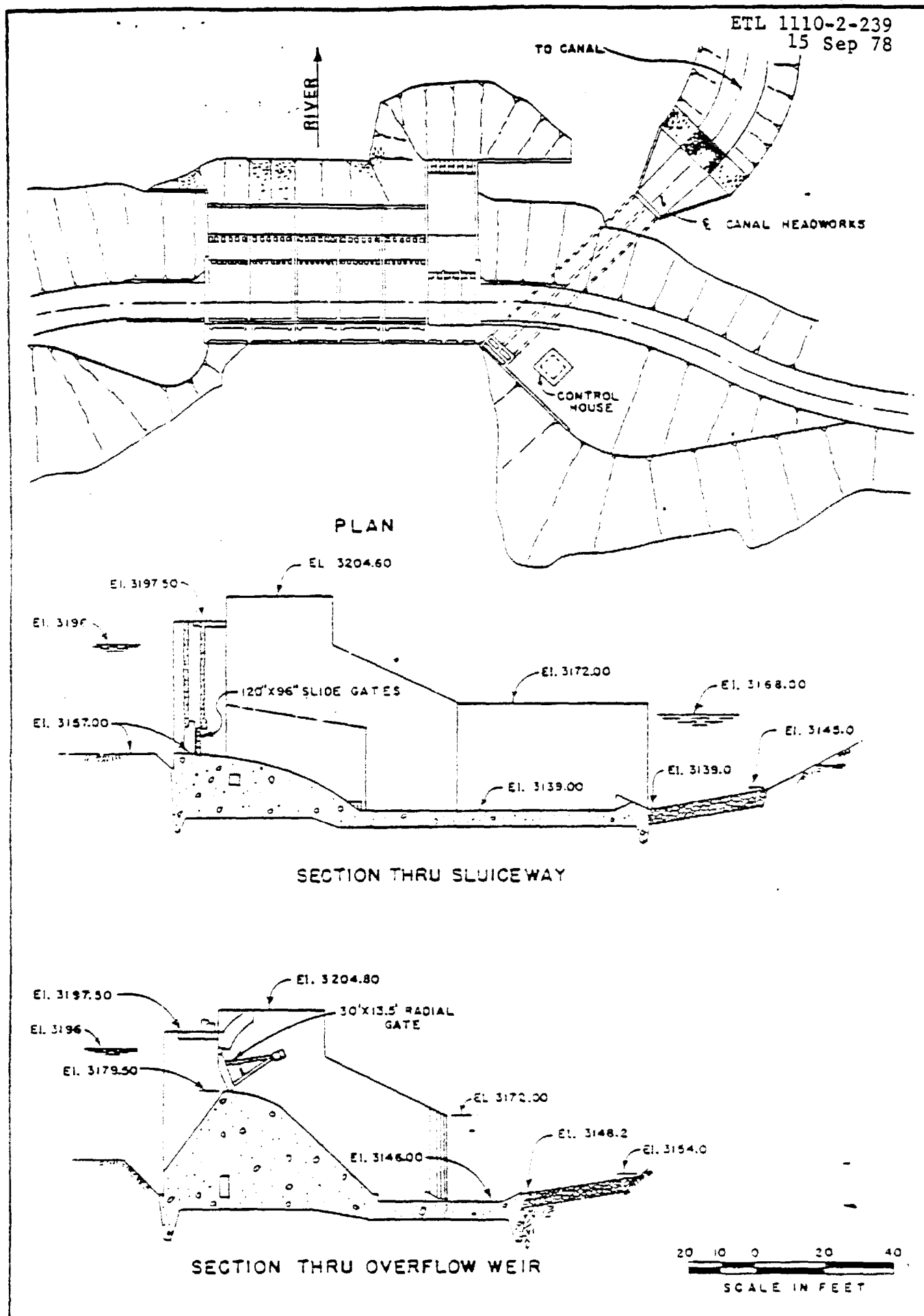
FIGURE 3 - SLUICeway IN EXAMPLE PROBLEM
