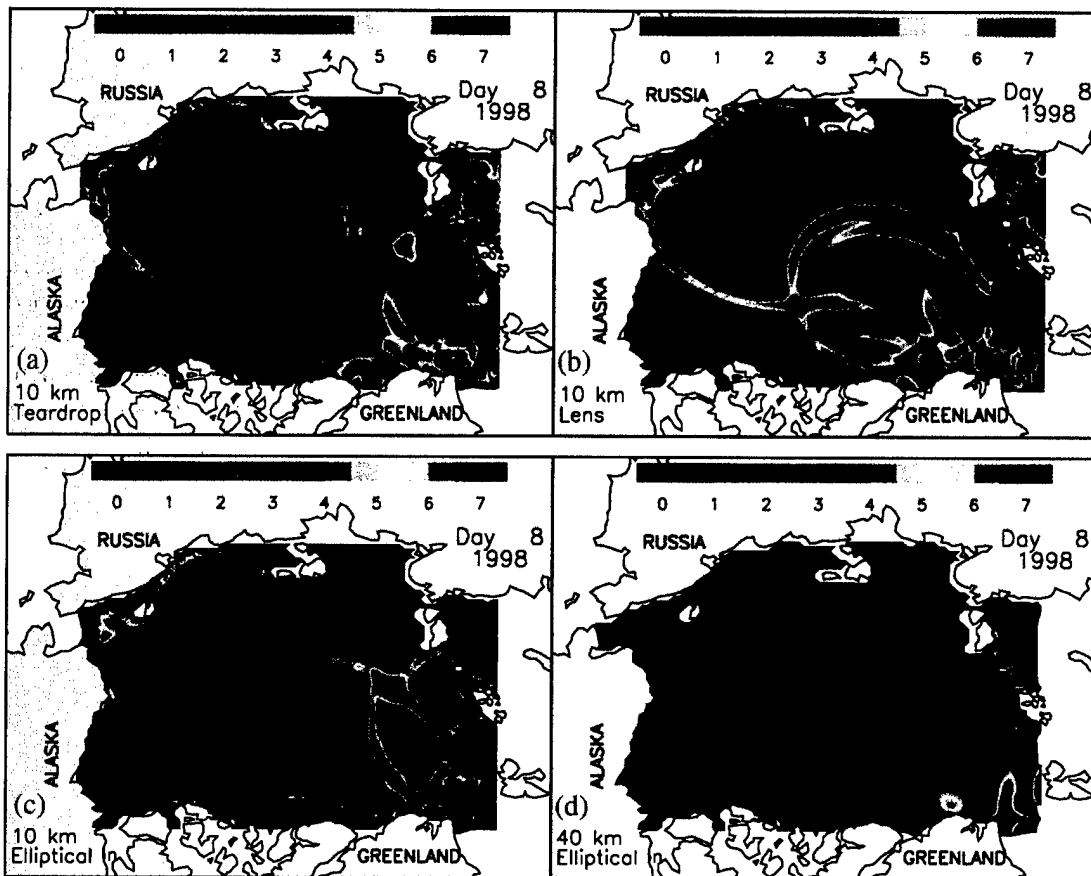
Figure 1. Modeled shear deformation (0.5%/day) of sea ice in the Arctic Ocean for January 8, 1998 using a 10-km resolution TED model with (a) a teardrop yield curve, (b) a lens yield curve, and (c) an elliptical yield curve, and using (d) a 40-km resolution TED model with an elliptical yield curve. The figure shows that the 10-km resolution sea ice model, with various viscous plastic rheologies, creates long shear deformation zones, whereas the 40-km model poorly simulates ice faults. This indicates that high-resolution models may be used to effectively simulate major oriented leads, cracks, or ridges.
