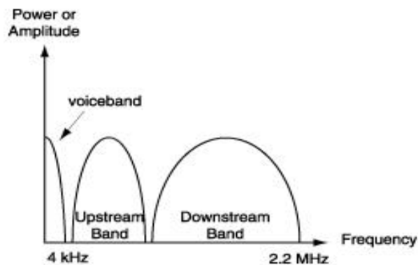
Figure 2. Digital Subscriber Line (DSL) Spectrum [From: DSLR02]
