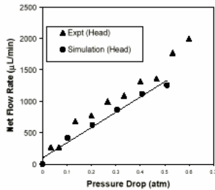
Fig 7 : Net Flow Rate in Tesla-type valve (difference in forward and reverse flow rates) vs. pressure drop. Comparison between experiment and simulation
