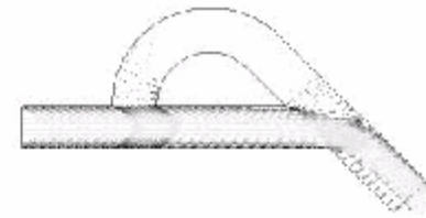
Fig 4 : Pressure on a slice plane through center of valve element. Upper figure is for forward direction flow. Units of pressure are MPa.
