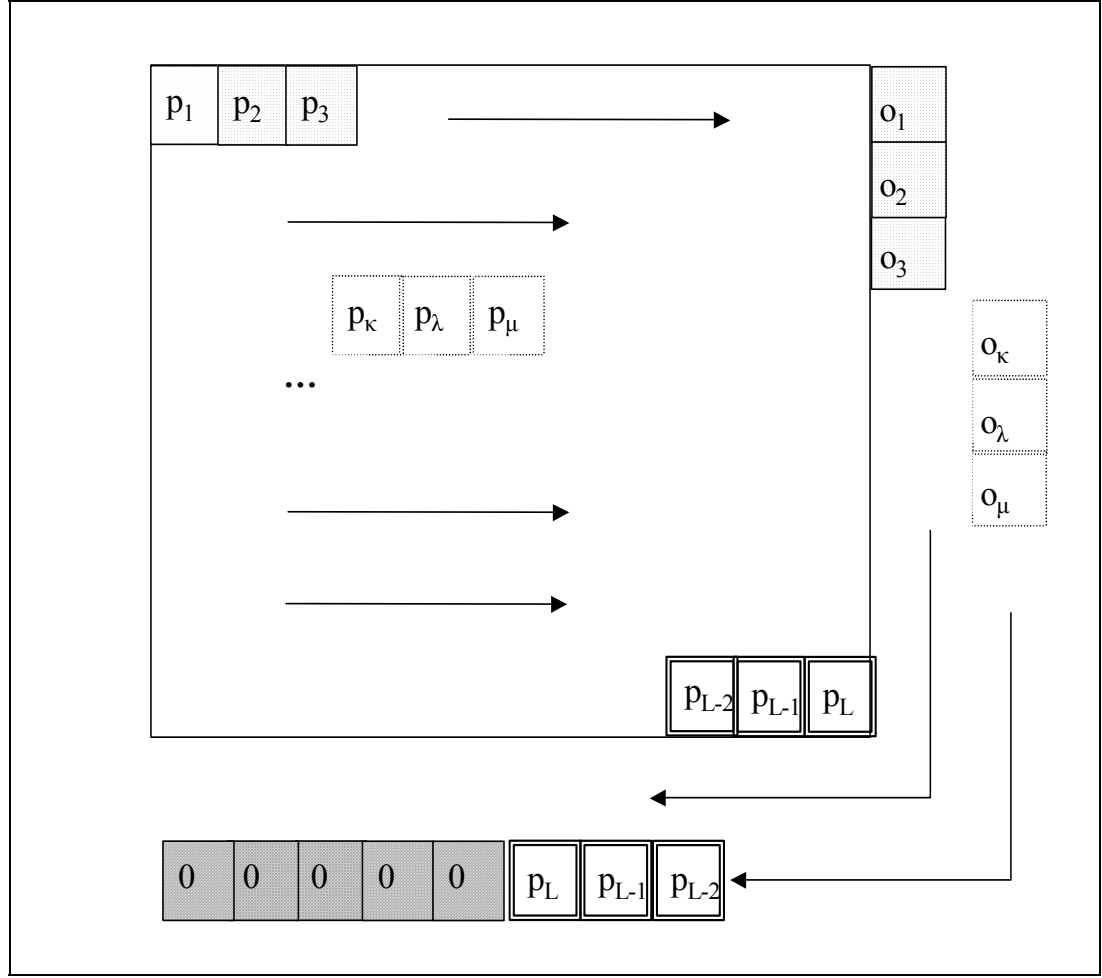
Figure 17. The concept of expanding the watermark after BCH coding, where the pixels p_i of the watermark are numbered from 1 to L , and o are the overhead bits.
