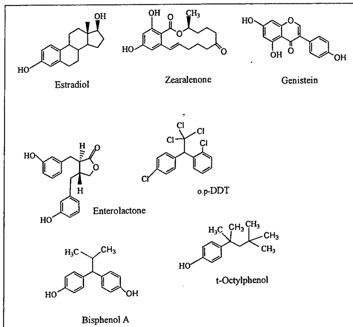
Figure 2. Structure of 17 \beta -estradiol and selected phyto-oestrogens and xeno-oestrogens. The compounds in this figure and/or in the text are:
