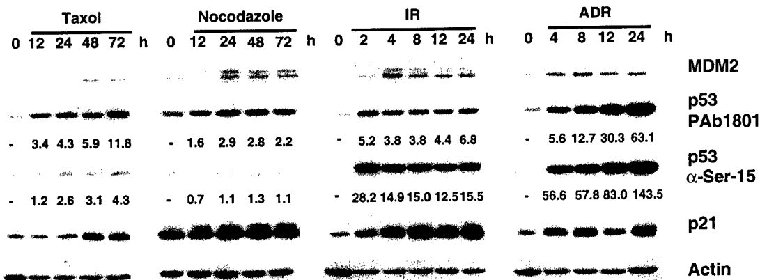
Figure 3 ATM-deficient cells have a delayed increase in p53 protein levels after Taxol treatment. Western analysis of MDM2, total p53 (PAb1801), Ser-15 phosphorylated p53 ( \alpha -Ser-15), p21, and actin protein levels in AT-1 (a) or NHDF (b) cells after treatment with Taxol (100 nM), nocodazole (83 nM), IR (10 Gy), and ADR (350 nM). Results are representative of three independent experiments
