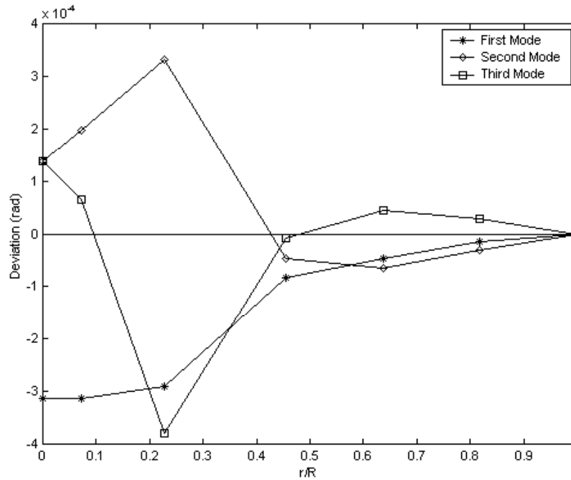
Figure 22. Deviation of Rotating versus Non-Rotating Wing Mode Shapes.
