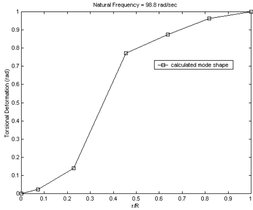
Figure 19. Non-Rotating Wing First Mode Shape.
