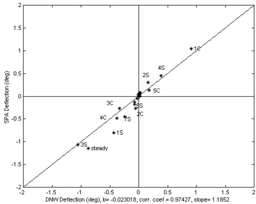
Figure 87. Linear Regression Plot of Five-Mode SPA versus Measured Torsional Deformation by Harmonic at x = 0.55 .
