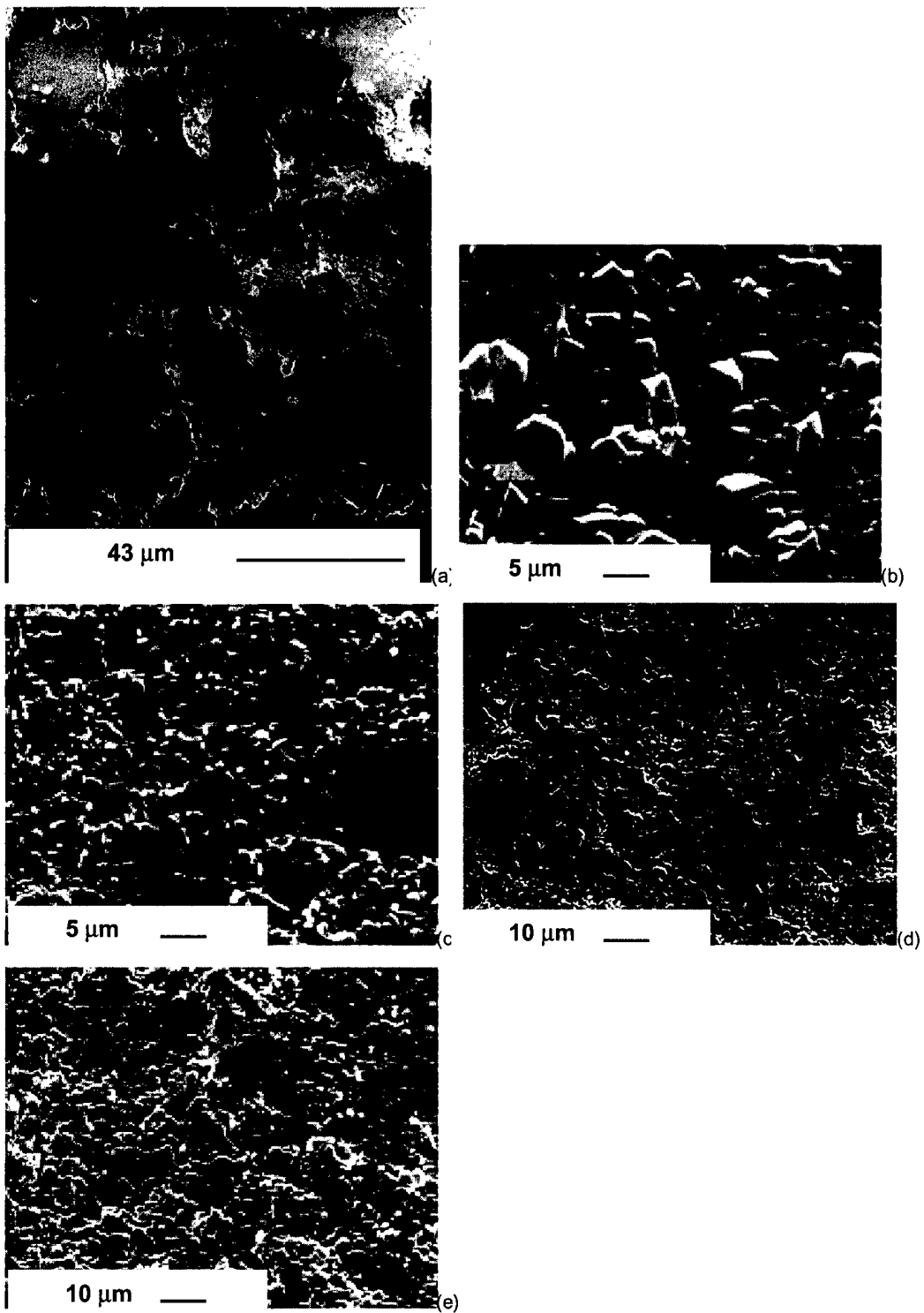
Figure 6.8: Wear tracks of Al 2 O 3 with the addition of (a) CuO, (b) MnO 2 , (c) MgO, (d) ZnO and (e) B 2 O 3 , after sliding against alumina balls.
