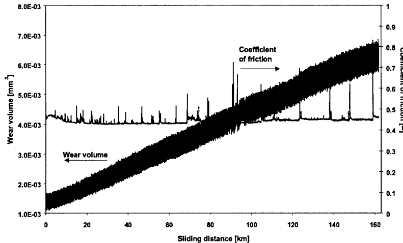
Figure 4.1: On-line analysis of the wear volume and coefficient of friction of the tribo-system measured for ZTA pin against ZTA disc made by colloidal filtration (Test conditions: F = 6 N, P_{Hertz} = 1.3 GPa, v = 0.5 m/s, r_{curv} = 5.2 mm, total sliding distance = 162 km).
