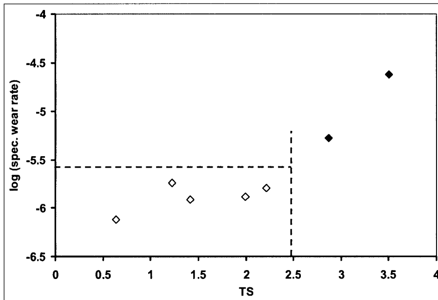
Figure 5.5: Specific wear rates of a Z3500 disc sliding against Si 3 N 4 pins at different TS -values: open markers: mild wear and solid markers: severe wear.
