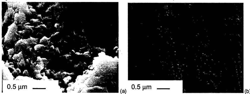
Figure 5.9: Wear tracks on ZY5 discs after sliding against two zirconia pins. Both tests were performed at 5 N. (a) Y-TZP pin at 0.07 m/s, showing severe wear, (b) ZY5 pin at 0.04 m/s, showing mild polishing.
