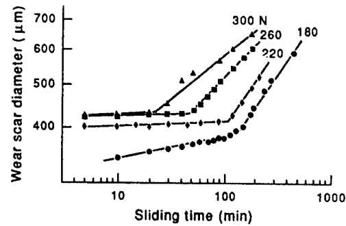
Figure 1.5: Wear vs. sliding time showing the abrupt change in functional dependence for each load, indicative of two stage wear behaviour [45].
